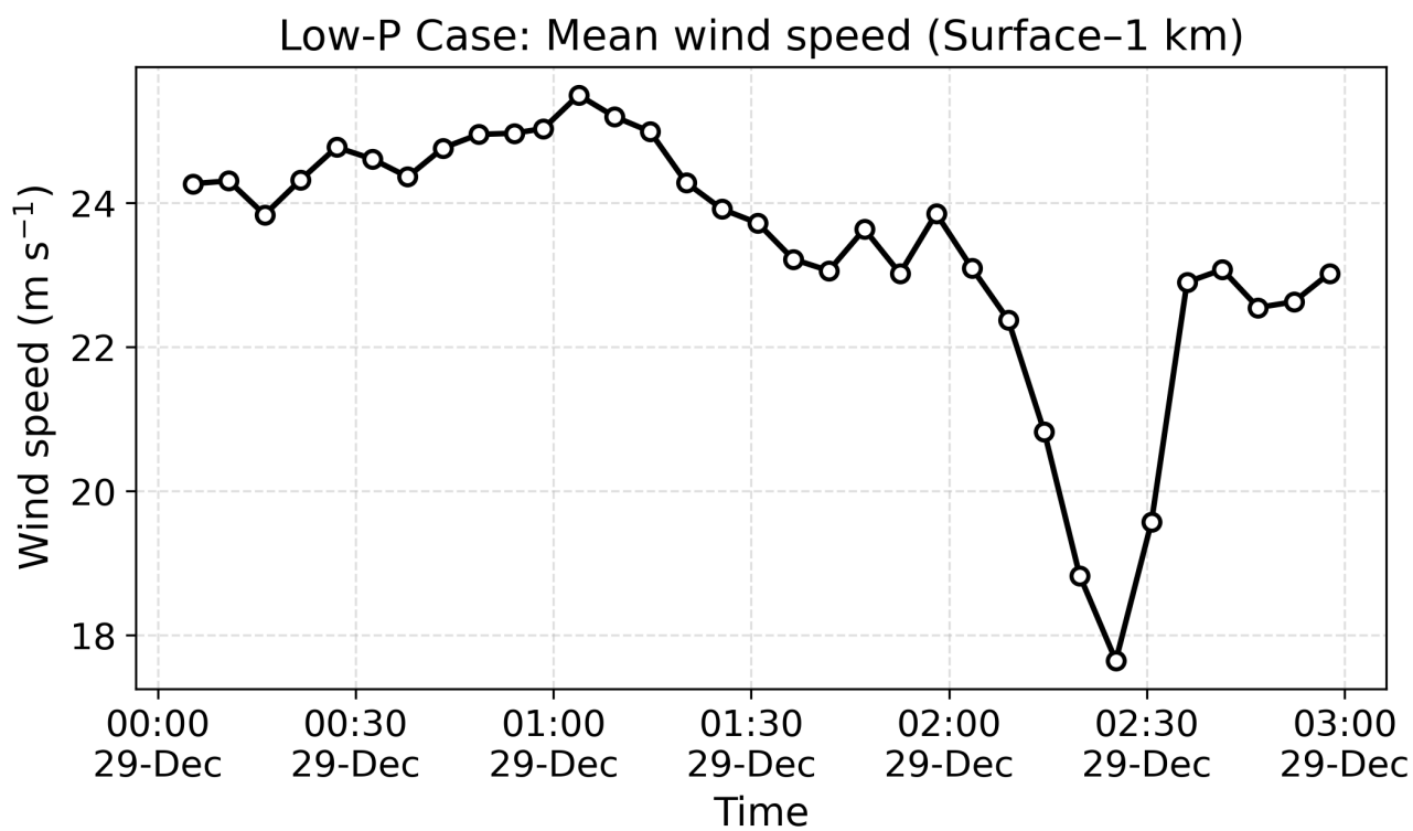
Figure S1. Wind speed time series during the Low-P event. Time series of the mean wind speed below 1 km derived from the radar VAD analysis during the Low-P event.
