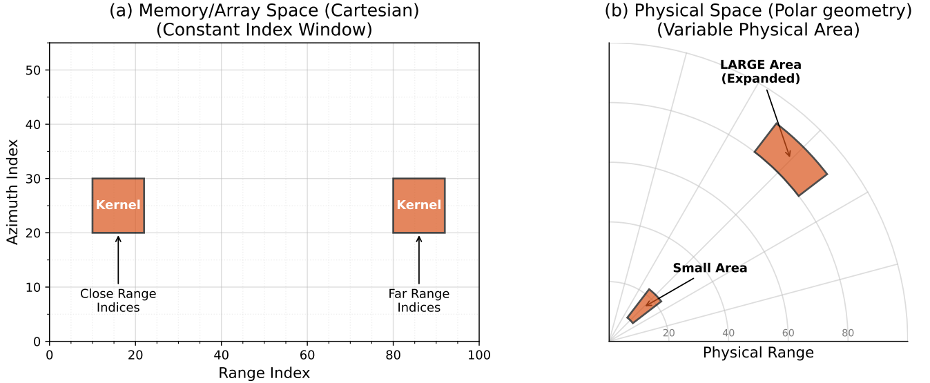
Figure 1. Conceptual comparison of coordinate distortion for (a) a window of constant size in grid space (range-angle indices) that corresponds to (b) physically different areas in a physical space depending on the range. At close range, the physical area is small, whereas at far range, it expands significantly. This distortion necessitates dynamic kernel sizing to maintain a constant physical smoothing scale.
