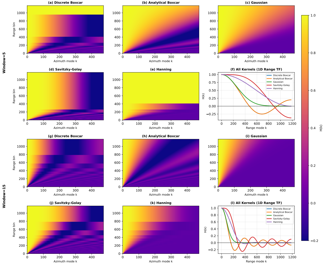
Figure 3. Spectral response of different kernels for two window sizes. Window 5: (a)-(e) 2D angle transfer functions, and (f) Range transfer function. Window 15: (g)-(k) Angle transfer functions, and (l) Range transfer function.
