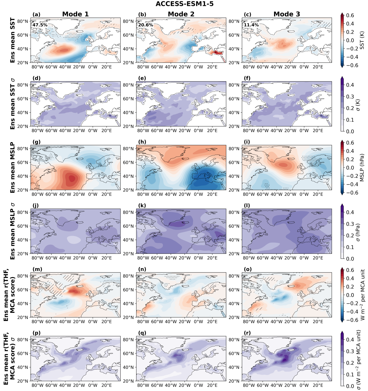
Figure S3. Ensemble mean contemporaneous autumn atmosphere-ocean co-variability in ACCESS-ESM1-5. Heterogeneous patterns for MCA modes 1-3 for autumn SST, autumn MSLP, and autumn turbulent heat flux (THF) regressed onto the corresponding MCA time series ( r(\text{THF}, \text{MCA score}) ). Panels are arranged left-to-right by mode (columns: Mode 1-3) and top-to-bottom by variable: (a-c) ensemble mean SST, (d-f) ensemble spread in SST, (g-i) ensemble mean MSLP, (j-l) ensemble spread in MSLP, (m-o) ensemble mean r(\text{THF}, \text{MCA score}) , and (p-r) ensemble spread in r(\text{THF}, \text{MCA score}) . Hatching indicates regions where the ERA5 value exceeds the 97.5th percentile of the ensemble spread, and stippling indicates regions where ERA5 falls below the 2.5th percentile of the ensemble spread.
