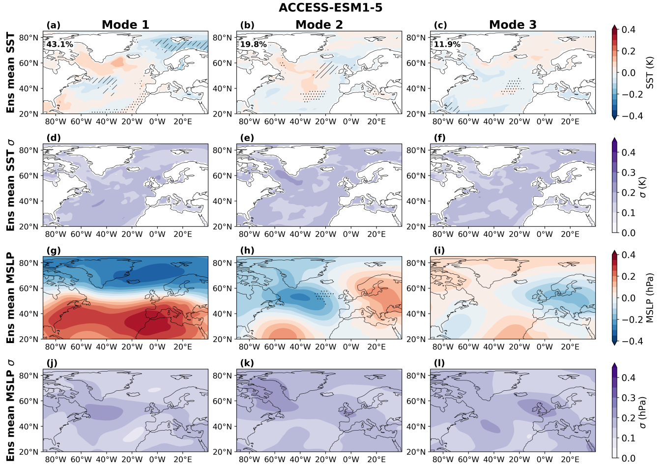
Figure S20. Ensemble mean lagged autumn-winter atmosphere-ocean co-variability. Heterogeneous patterns for MCA modes 1-3 are shown for autumn SST and winter MSLP. (a-c) ensemble mean SST, (d-f) ensemble spread in SST ( \sigma ), (g-i) ensemble mean MSLP, (j-l) ensemble spread in MSLP ( \sigma ). Hatching indicates regions where the ERA5 value exceeds the 97.5th percentile of the ensemble spread, and stippling indicates regions where ERA5 falls below the 2.5th percentile of the ensemble spread. The percentage of squared covariance explained by each mode is shown in the legend in panels a-c
