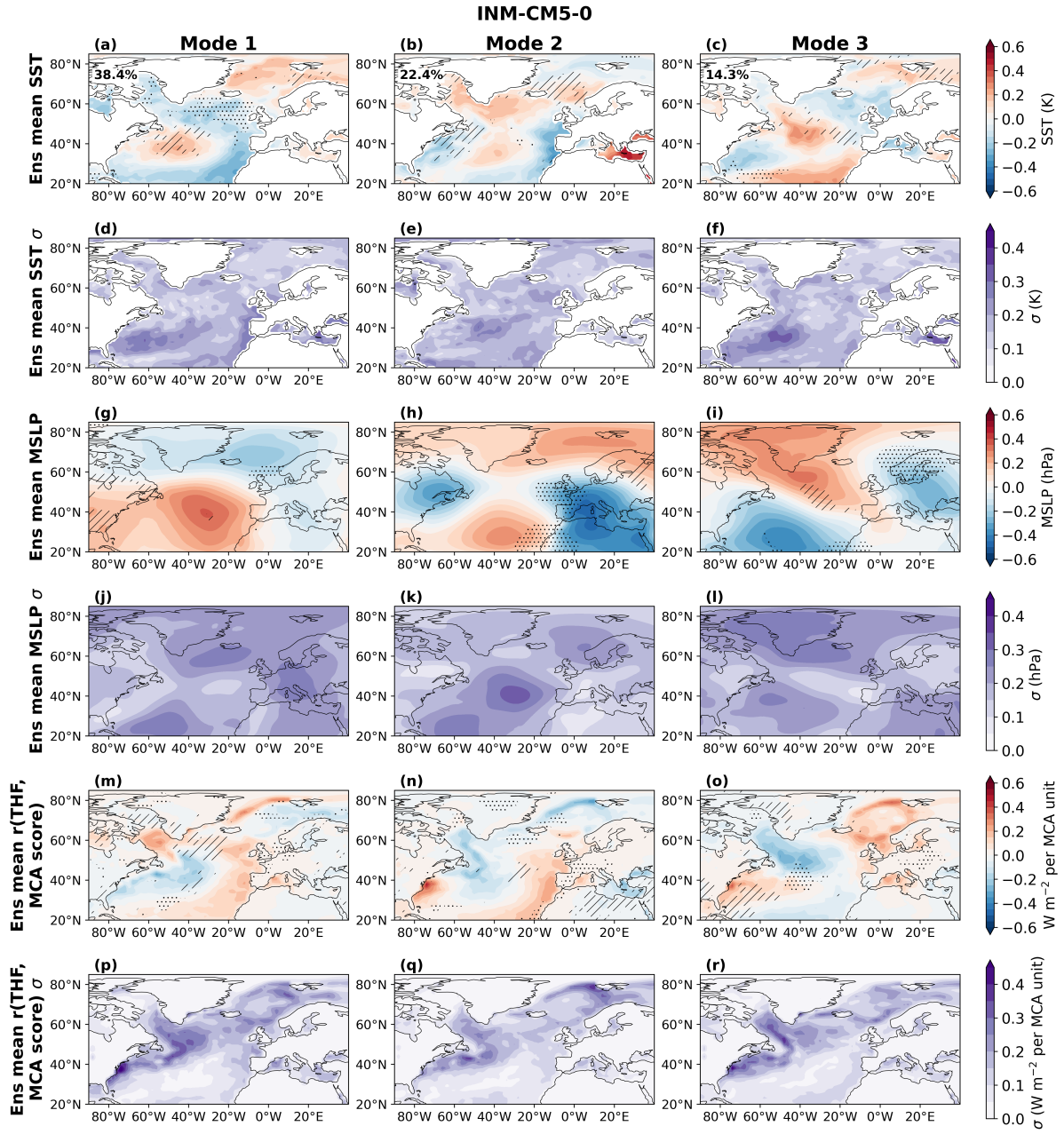
Figure S9. As in SI Fig. S3 for INM-CM5-0.
