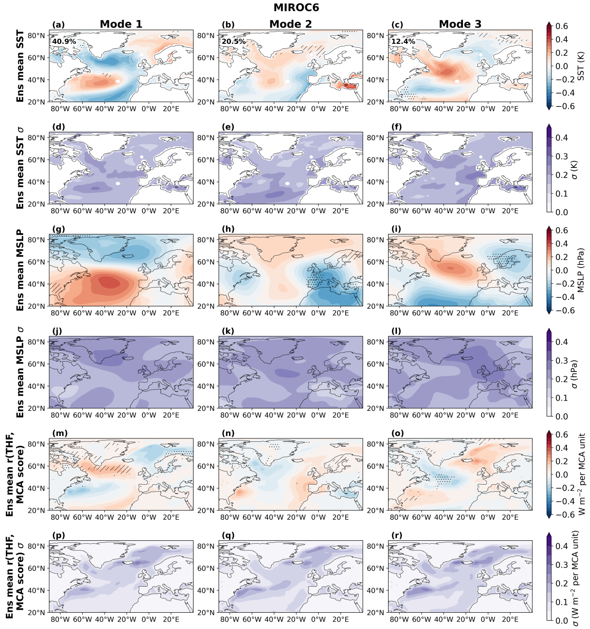
Figure S12. As in SI Fig. S3 for MIROC6.
