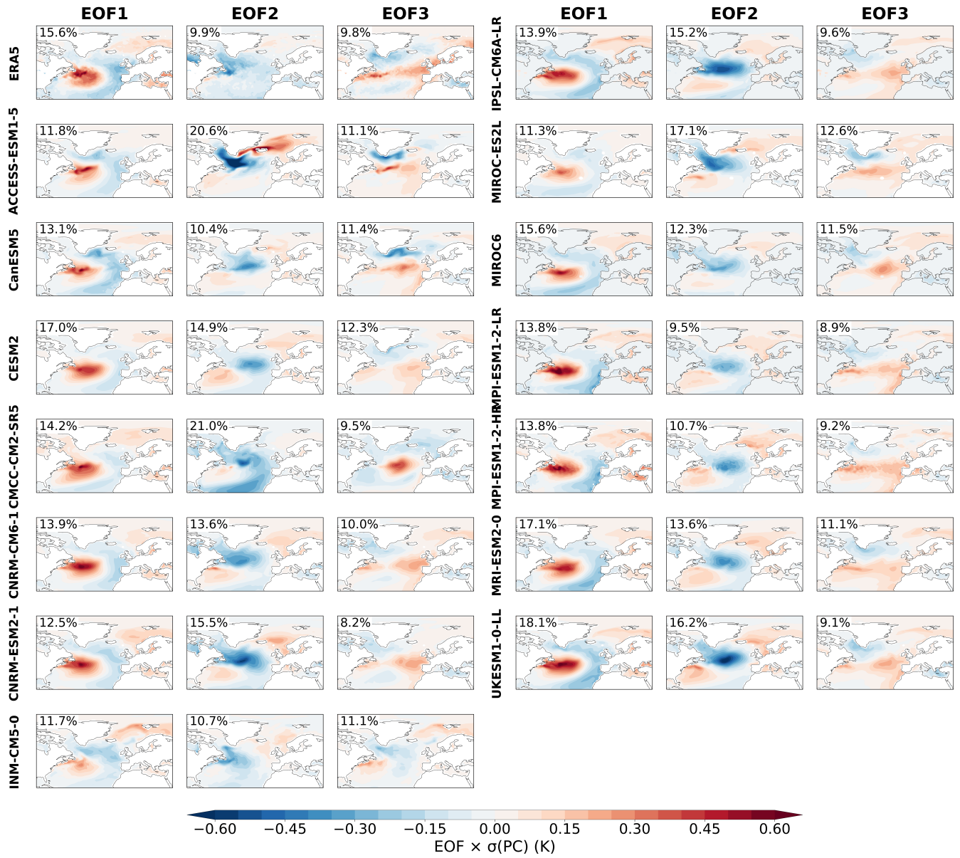
Figure S17. EOFs 1-3 of autumn SST. Percentage of variance explained by each mode indicated in left corner.
