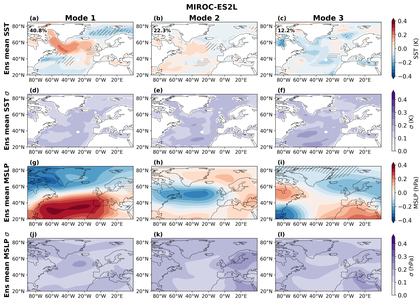
Figure S28. As in SI Fig.S20 for MIROC-ES2L.
