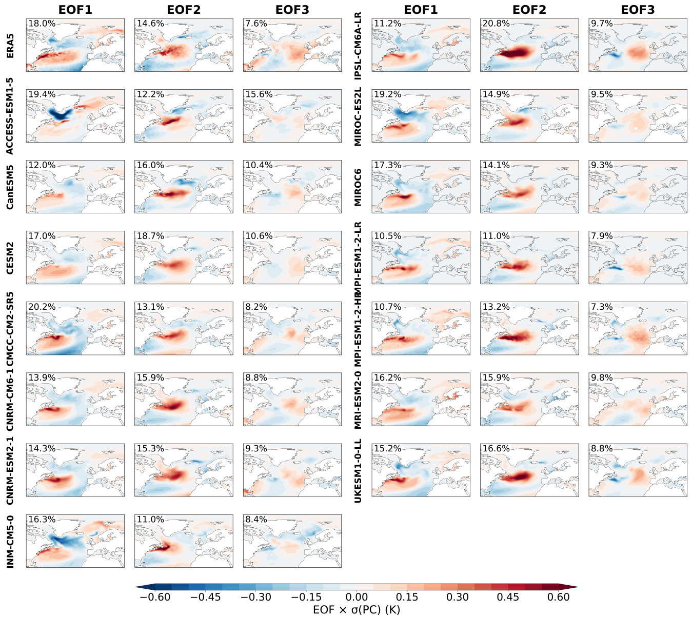
Figure S34. EOFs 1-3 of winter SST. Percentage of variance explained by each mode indicated in left corner.
