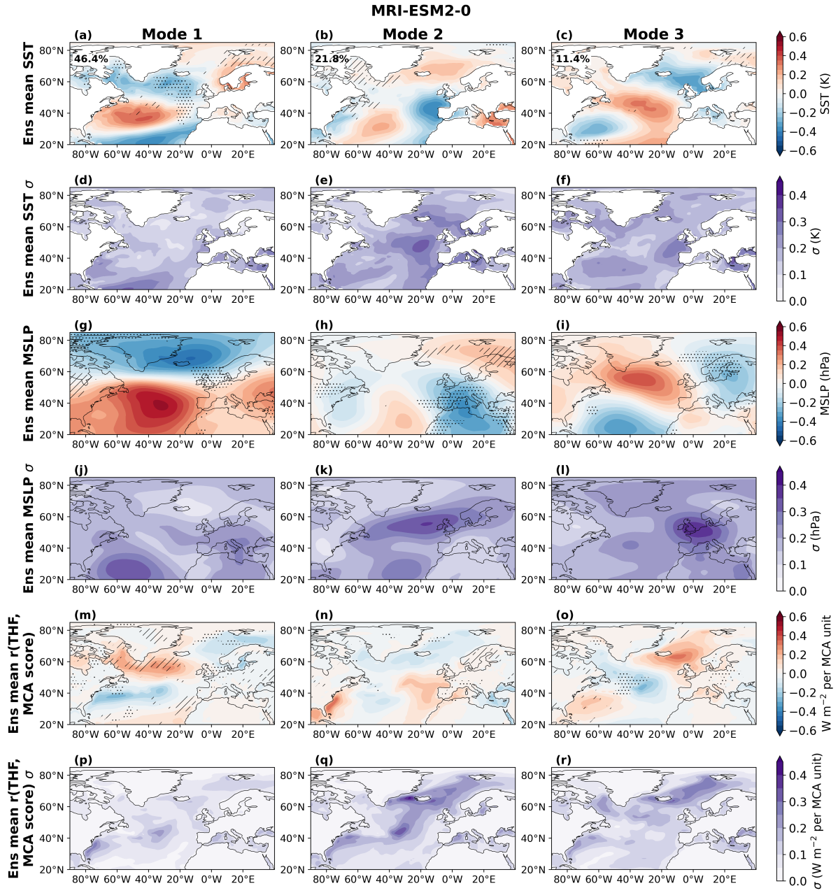
Figure S15. As in SI Fig. S3 for MRI-ESM2-0.
