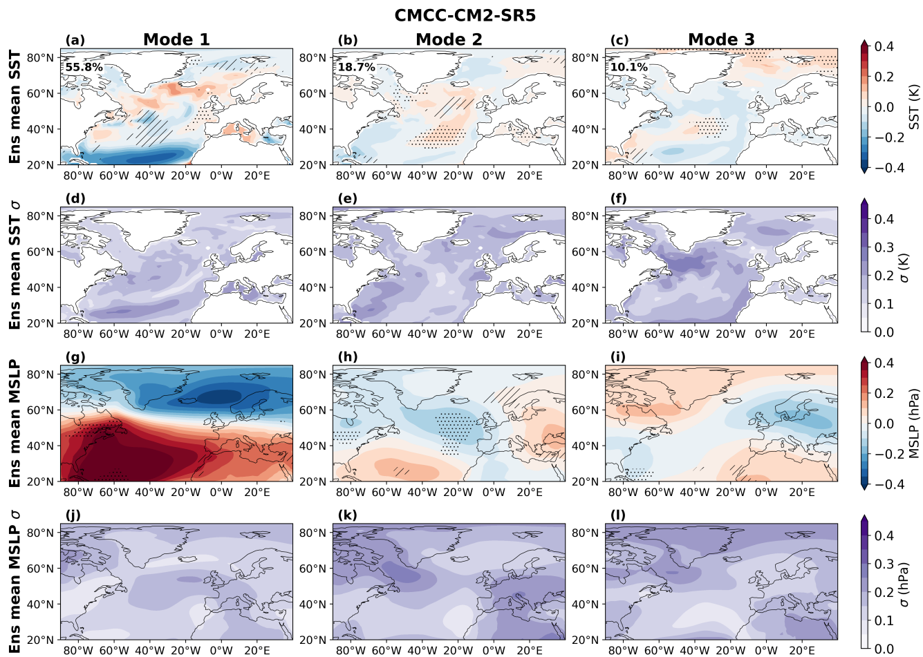
Figure S23. As in SI Fig.S20 for CMCC-CM2-SR5.
