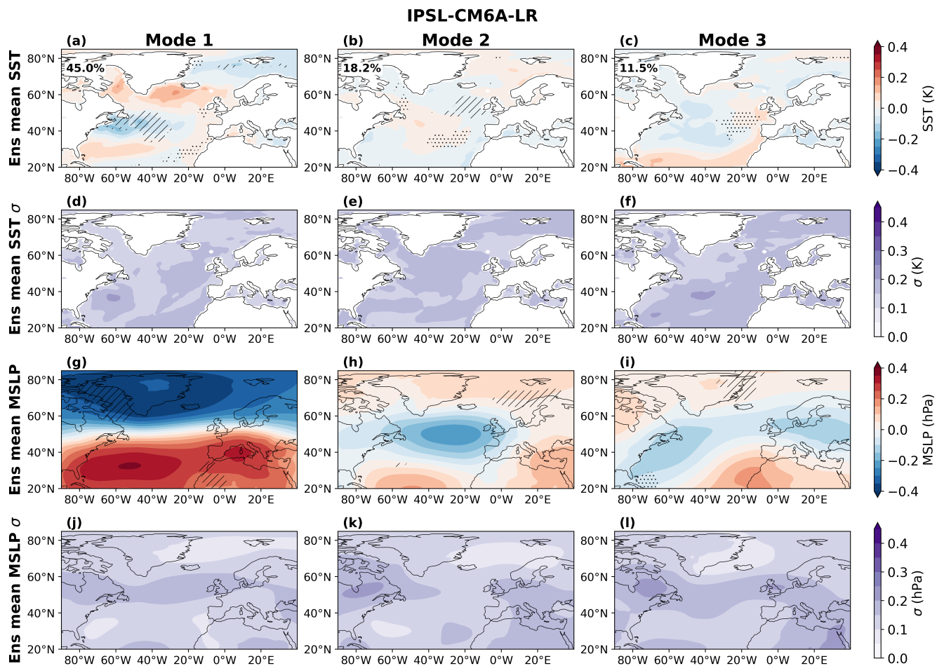
Figure S27. As in SI Fig.S20 for IPSL-CM6A-LR.
