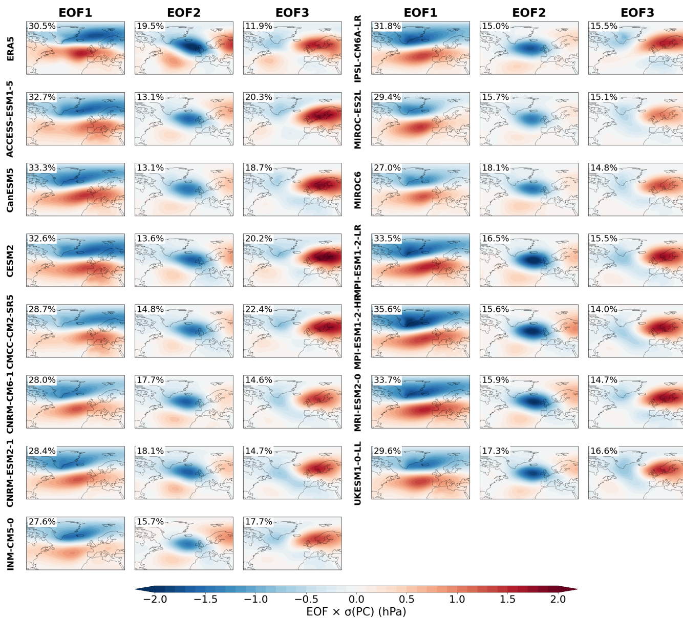
Figure S1. EOFs 1-3 of autumn MSLP. Percentage of variance explained by each mode indicated in left corner.
