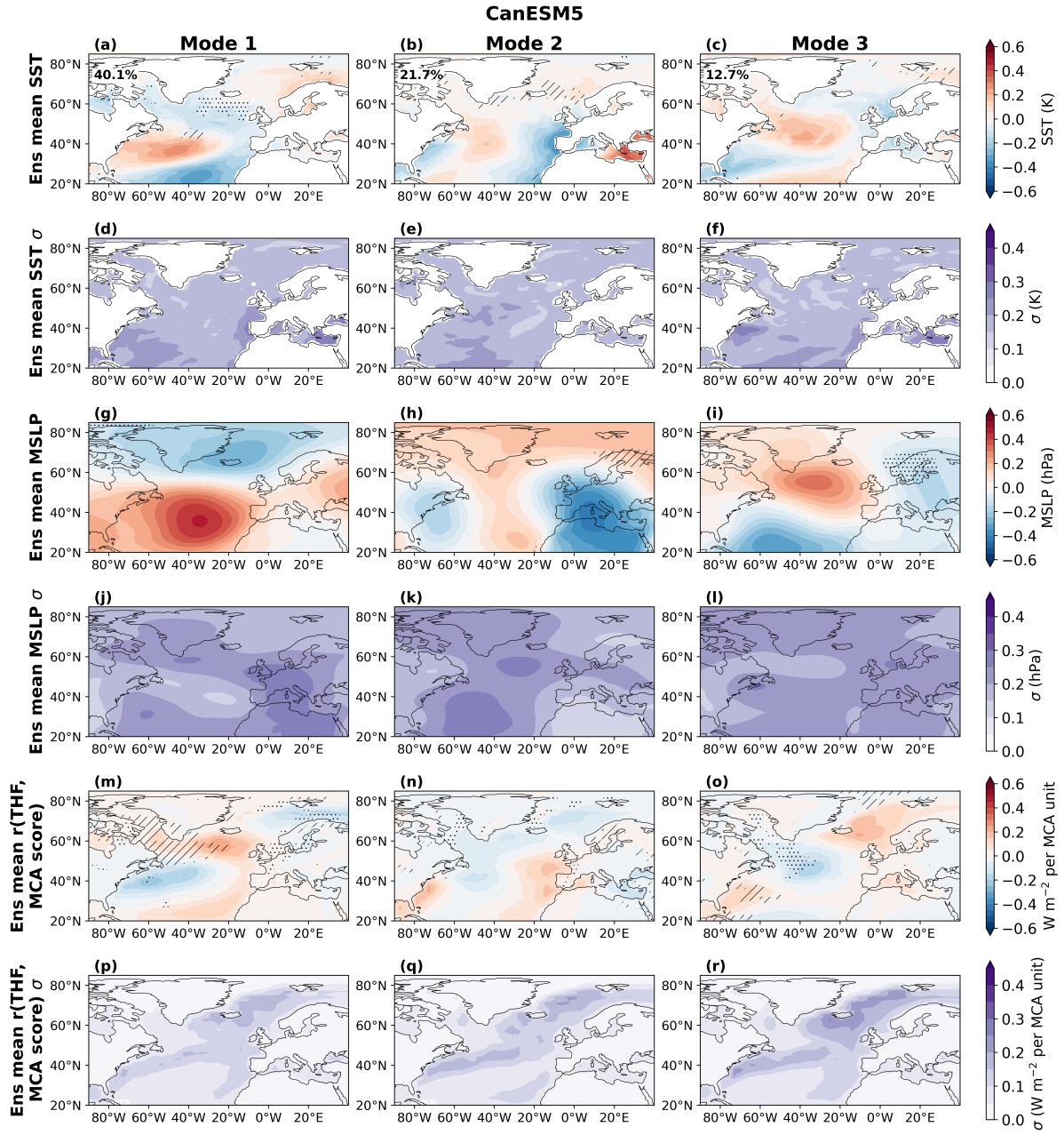
Figure S4. As in SI Fig. S3 for CanESM5.
