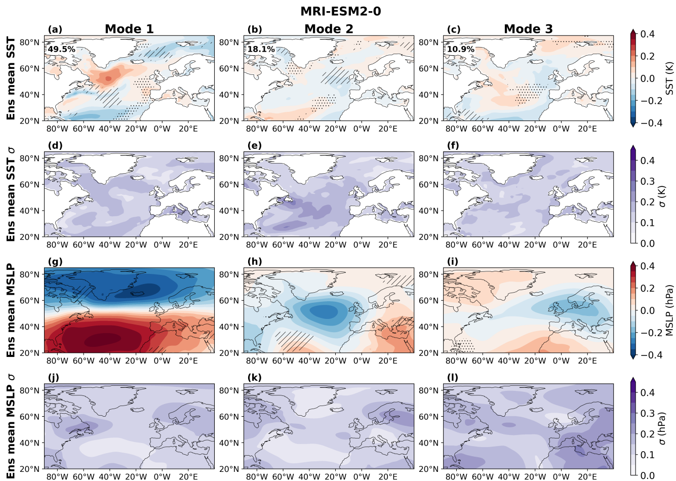
Figure S32. As in SI Fig.S20 for MRI-ESM2-0.
