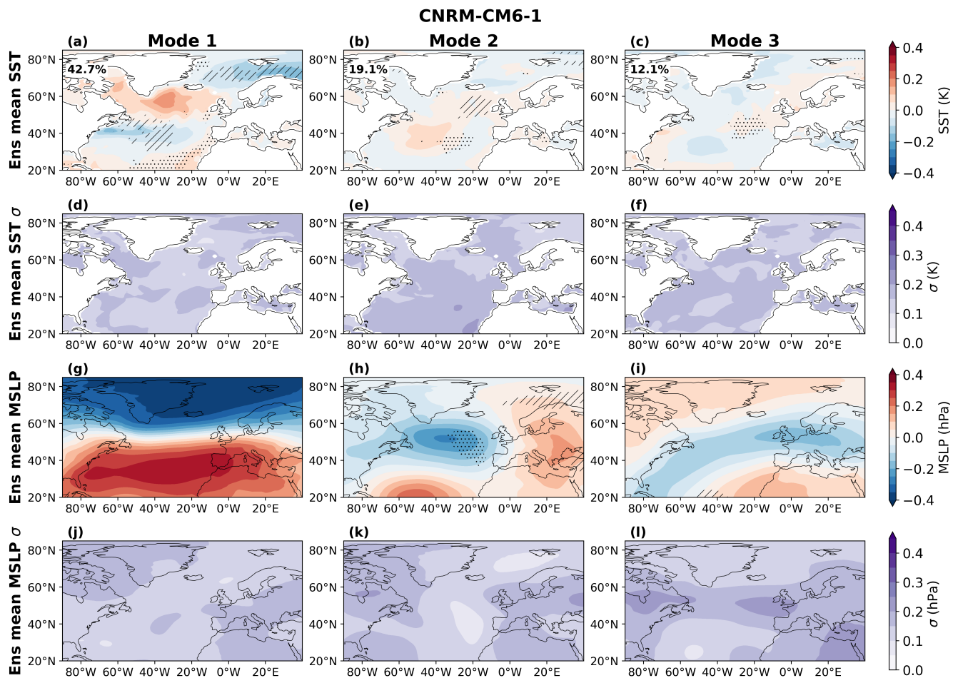
Figure S24. As in SI Fig.S20 for CNRM-CM6-1.
