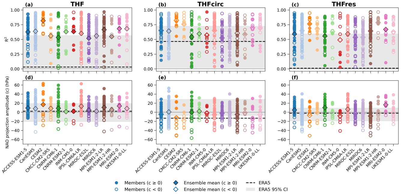
Figure S35. Projection of the regression pattern of winter North Atlantic MSLP onto PC2 of the autumn THF components onto the winter NAO (EOF1) in ERA5 and models. Fraction of the variance explained by the NAO (a-c) and strength of the NAO signal (d-f). Circles are model members, diamonds are ensemble means, dashed black lines represent ERA5 1940-2014 and grey shading represents the sampling uncertainty for 1940-2014, blue solid lines represent ERA5 1940-2022 and blue dotted lines represent the sampling uncertainty for 1940-2022. Positive c values indicate a positive NAO and negative indicate a negative NAO.
