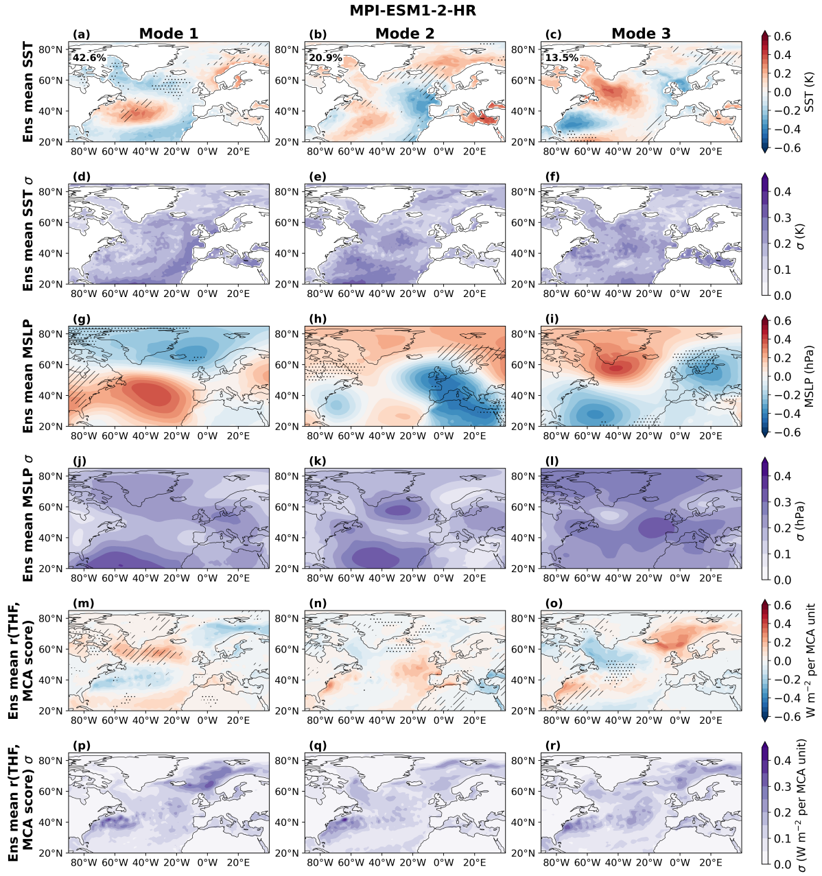
Figure S13. As in SI Fig. S3 for MPI-ESM1-2-HR.
