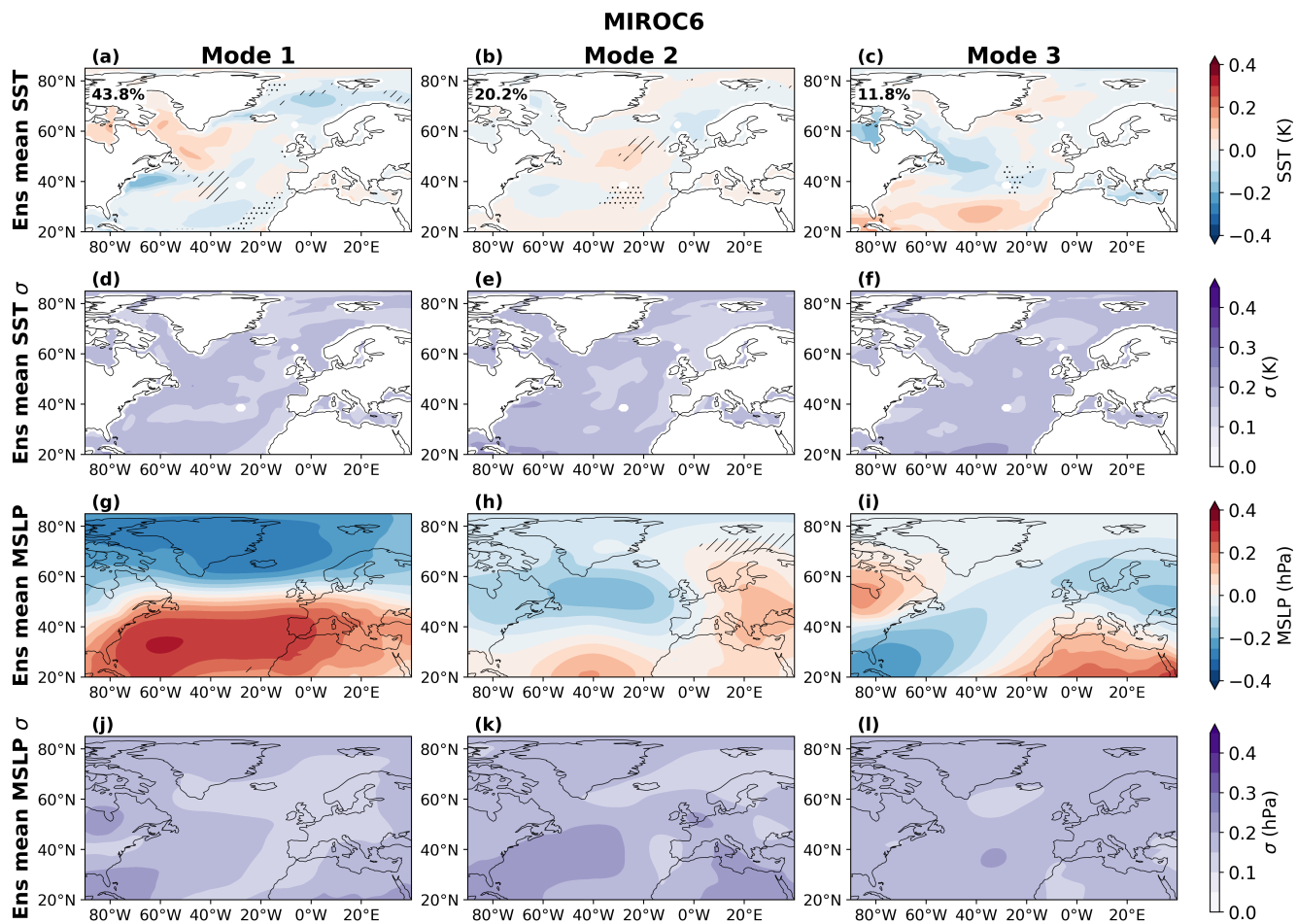
Figure S29. As in SI Fig.S20 for MIROC6.
