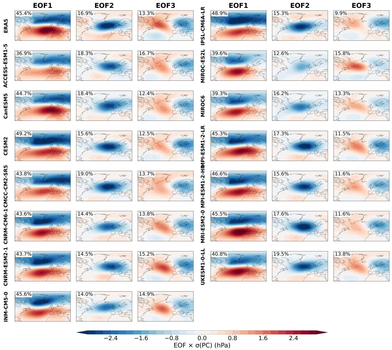
Figure S2. EOFs 1-3 of winter MSLP. Percentage of variance explained by each mode indicated in left corner.
