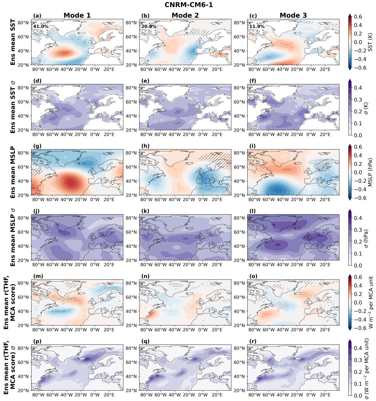
Figure S7. As in SI Fig. S3 for CNRM-CM6-1.
