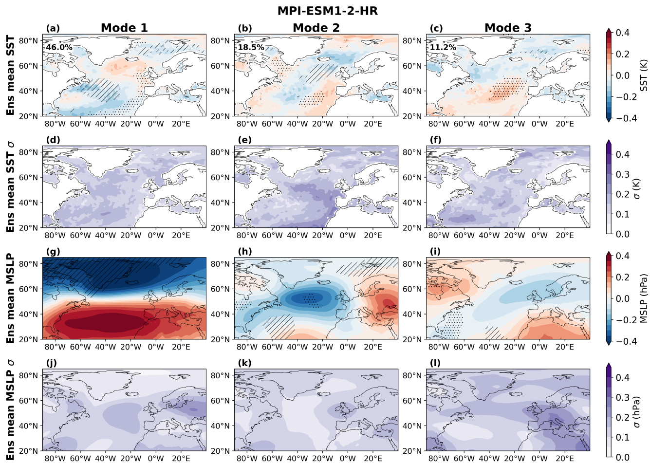
Figure S30. As in SI Fig.S20 for MPI-ESM1-2-HR.
