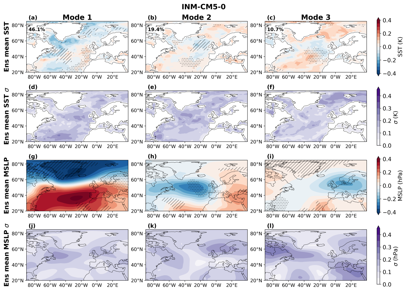
Figure S26. As in SI Fig.S20 for INM-CM5-0.
