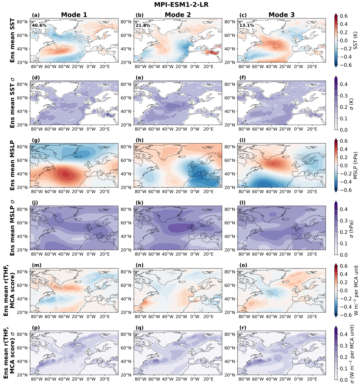
Figure S14. As in SI Fig. S3 for MPI-ESM1-2-LR.
