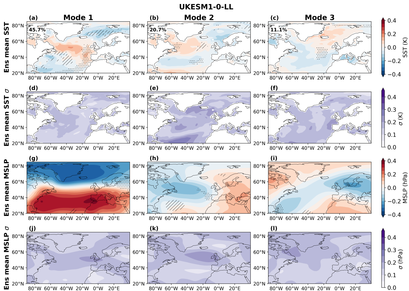
Figure S33. As in SI Fig.S20 for UKESM1-0-LL.
