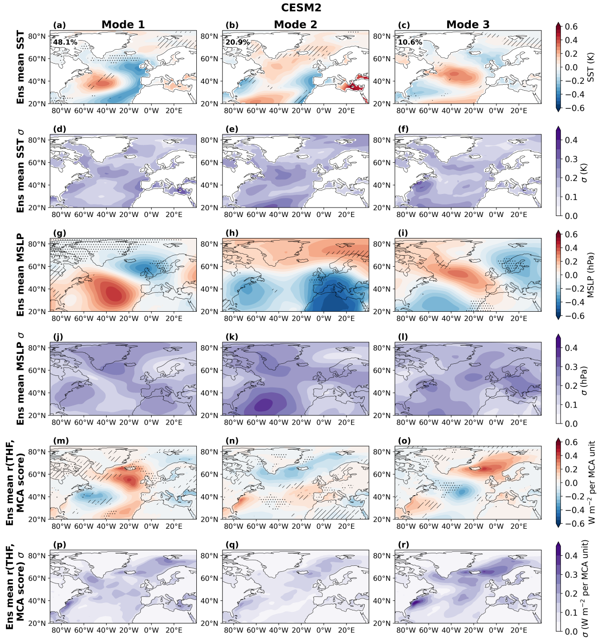
Figure S5. As in SI Fig. S3 for CESM2.
