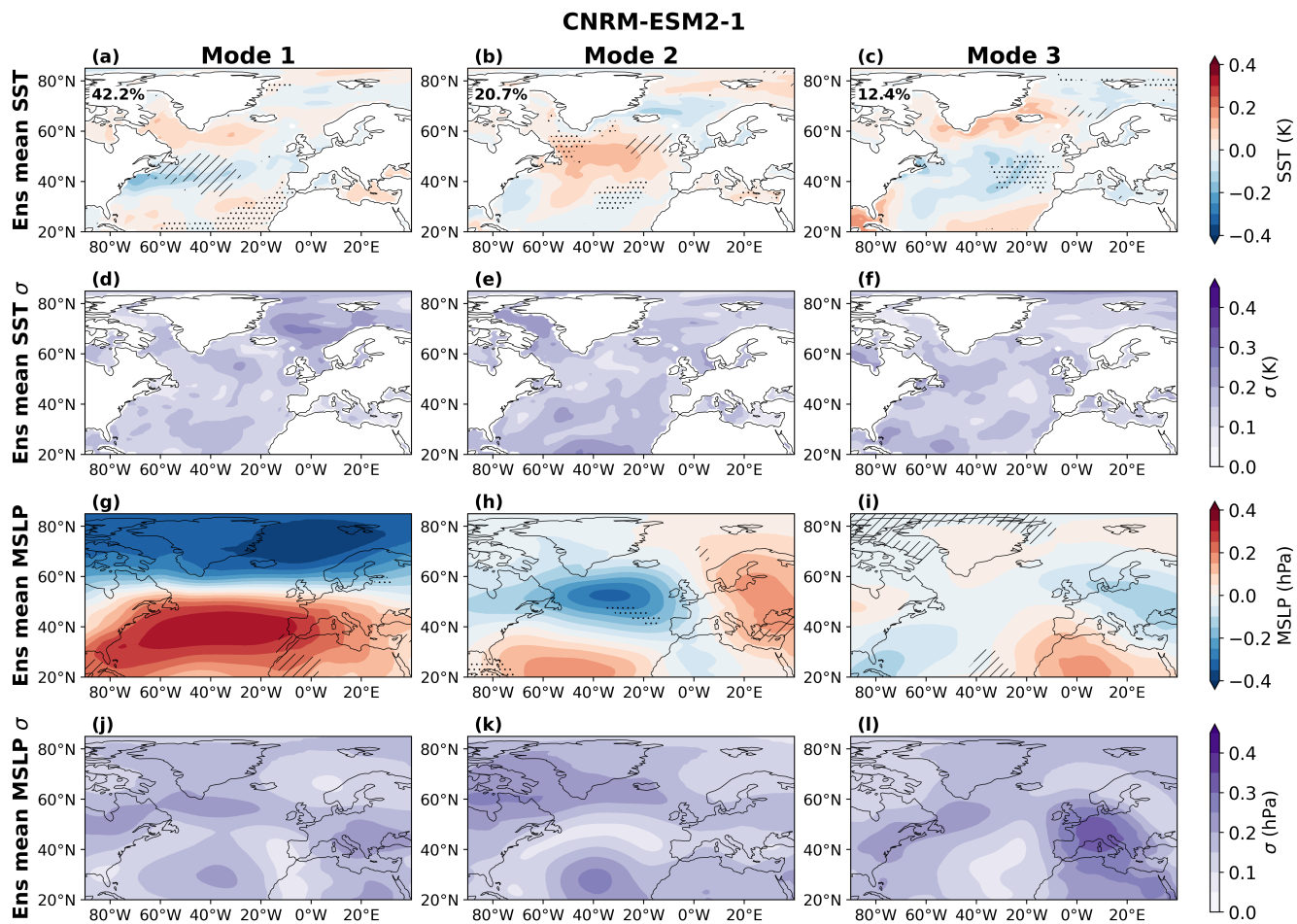
Figure S25. As in SI Fig.S20 for CNRM-ESM2-1.
