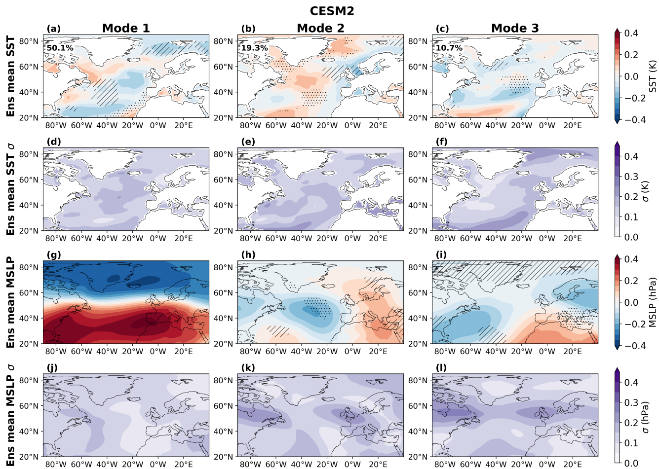
Figure S22. As in SI Fig.S20 for CESM2.
