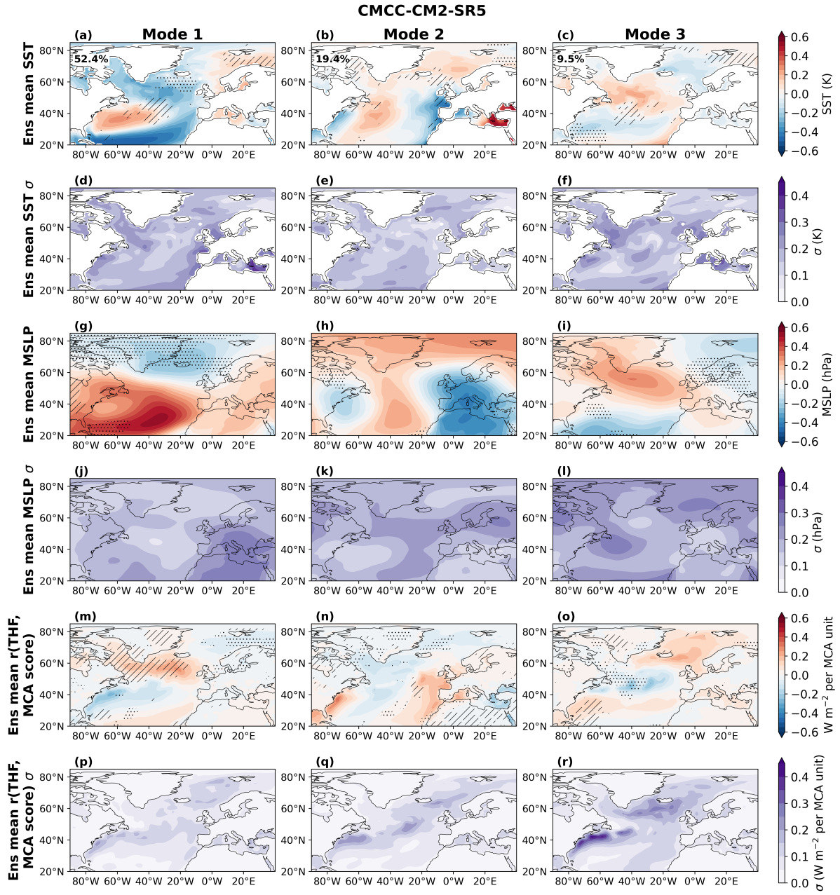
Figure S6. As in SI Fig. S3 for CMCC-CM2-SR5.
