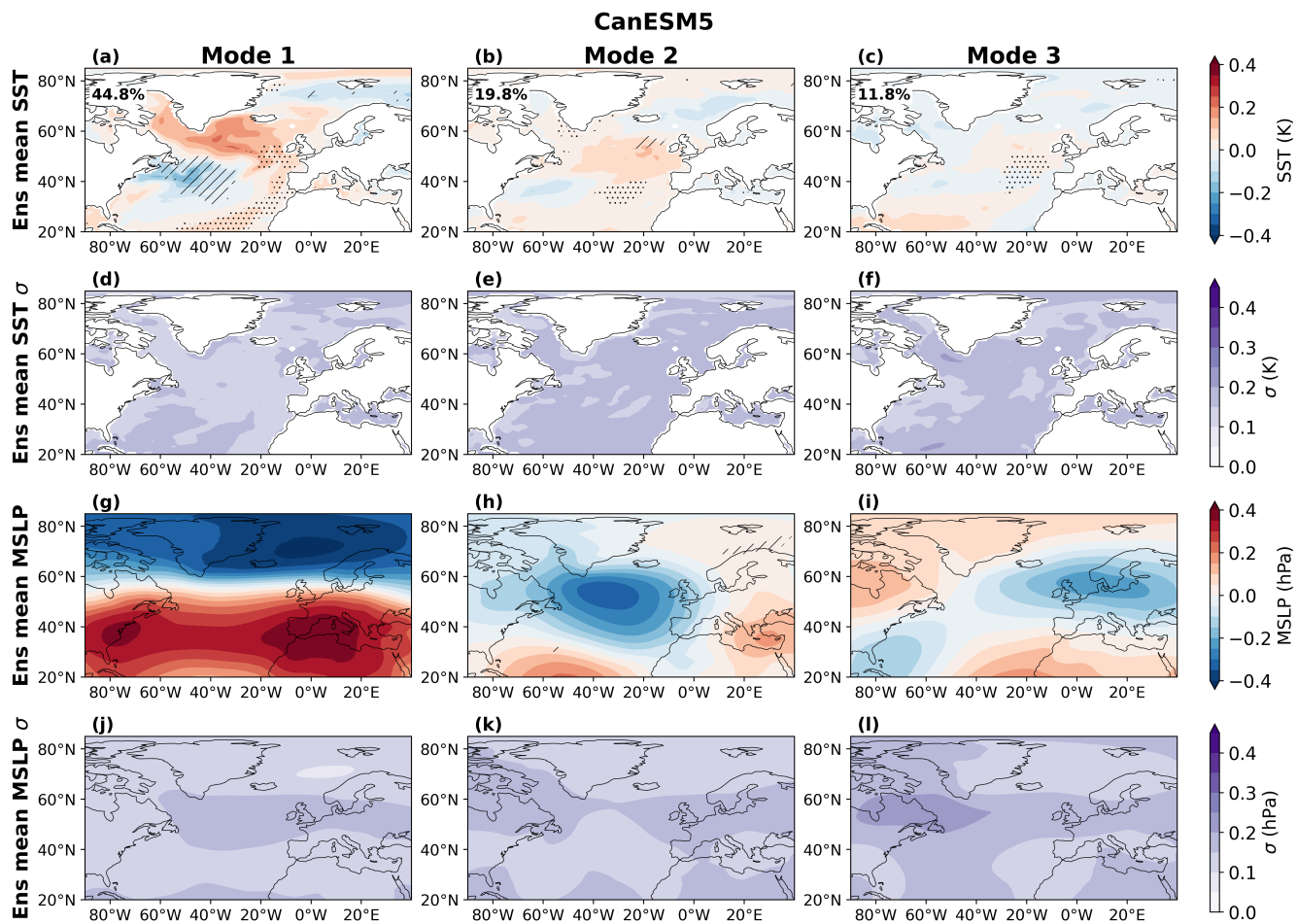
Figure S21. As in SI Fig. S20 for CanESM5.
