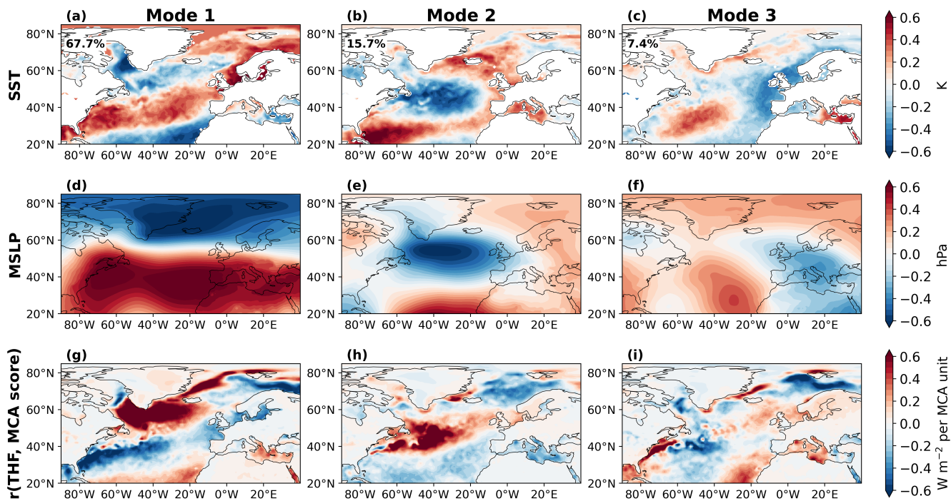
Figure S18. Contemporaneous winter atmosphere-ocean co-variability in ERA5. Heterogeneous patterns for MCA modes 1-3 are shown for winter SST (a-c), winter MSLP (d-f), and winter THF regressed onto the corresponding MCA timeseries (rTHF; MCA score) (g-i). Percentage of squared covariance explained by each mode is shown in the legend in panels a-c
