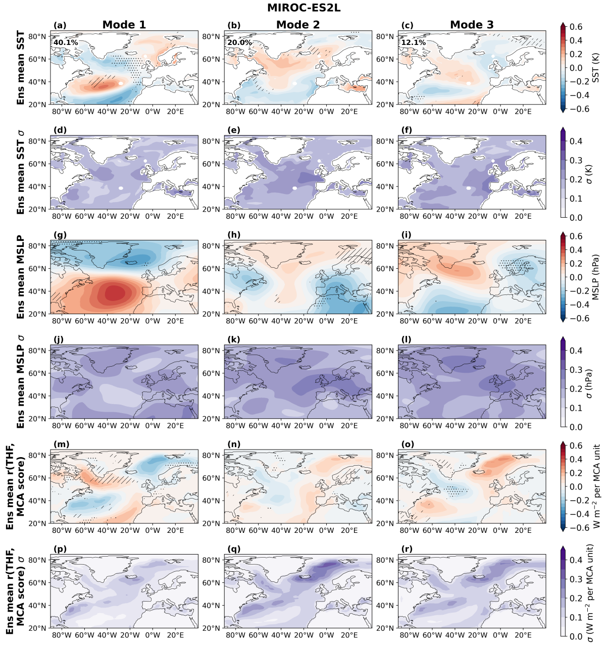
Figure S11. As in SI Fig. S3 for MIROC-ES2L.
