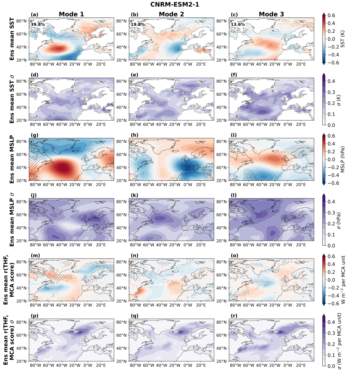
Figure S8. As in SI Fig. S3 for CNRM-ESM2-1.
