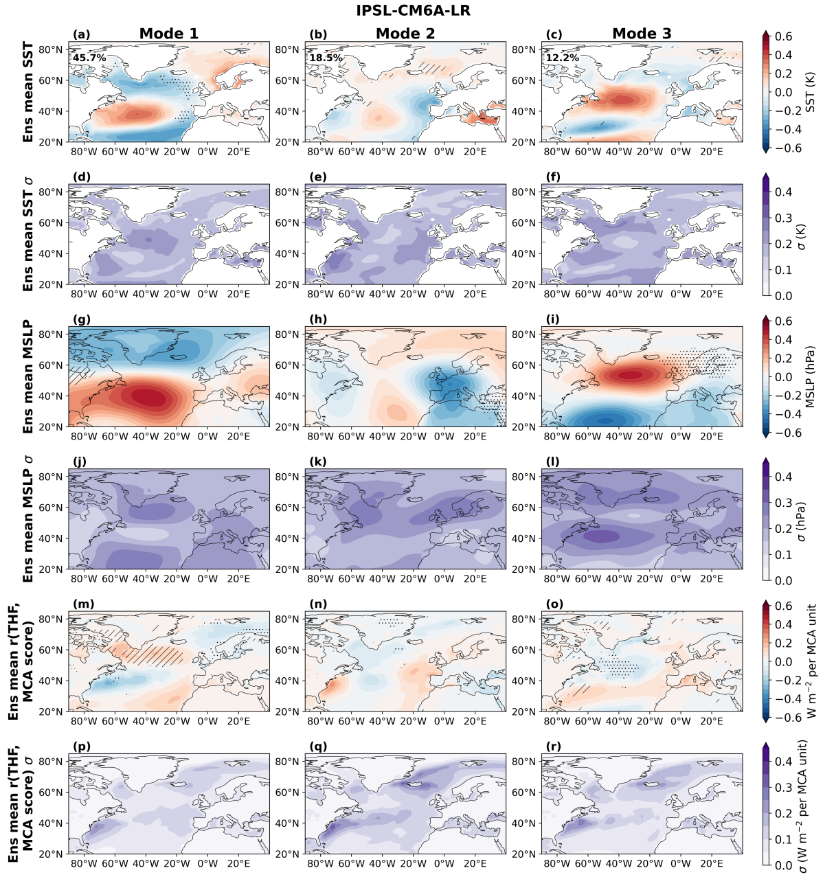
Figure S10. As in SI Fig. S3 for IPSL-CM6A-LR.
