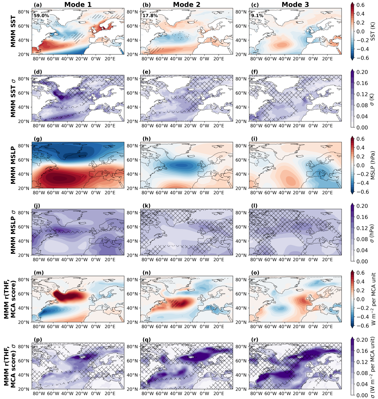
Figure S19. Multi-model mean contemporaneous winter atmosphere-ocean variability. Heterogeneous patterns for MCA modes 1-3 for winter SST, winter MSLP, and winter turbulent heat flux (THF) regressed onto the corresponding MCA time series ( r_{\text{THF}} ; MCA score). Panels are arranged left-to-right by mode (columns: Mode 1-3) and top-to-bottom by variable: (a-c) MMM SST, (d-f) inter-model spread in SST ( \sigma ), (g-i) MMM MSLP, (j-l) inter-model spread in MSLP ( \sigma ), (m-o) MMM r(\text{THF}, \text{MCA score}) , and (p-r) inter-model spread in r(\text{THF}, \text{MCA score}) ( \sigma ). Hatching indicates regions where the ERA5 value exceeds the 97.5th percentile of the ensemble spreads, and stippling indicates regions where ERA5 falls below the 2.5th percentile of the ensemble spreads. Cross-hatching in panels (d-f), (j-l) and (p-r) indicate where the inter-model spread is greater than the multi-model mean. The mean percentage of squared covariance explained by each mode is shown in the legend in panels a-c
