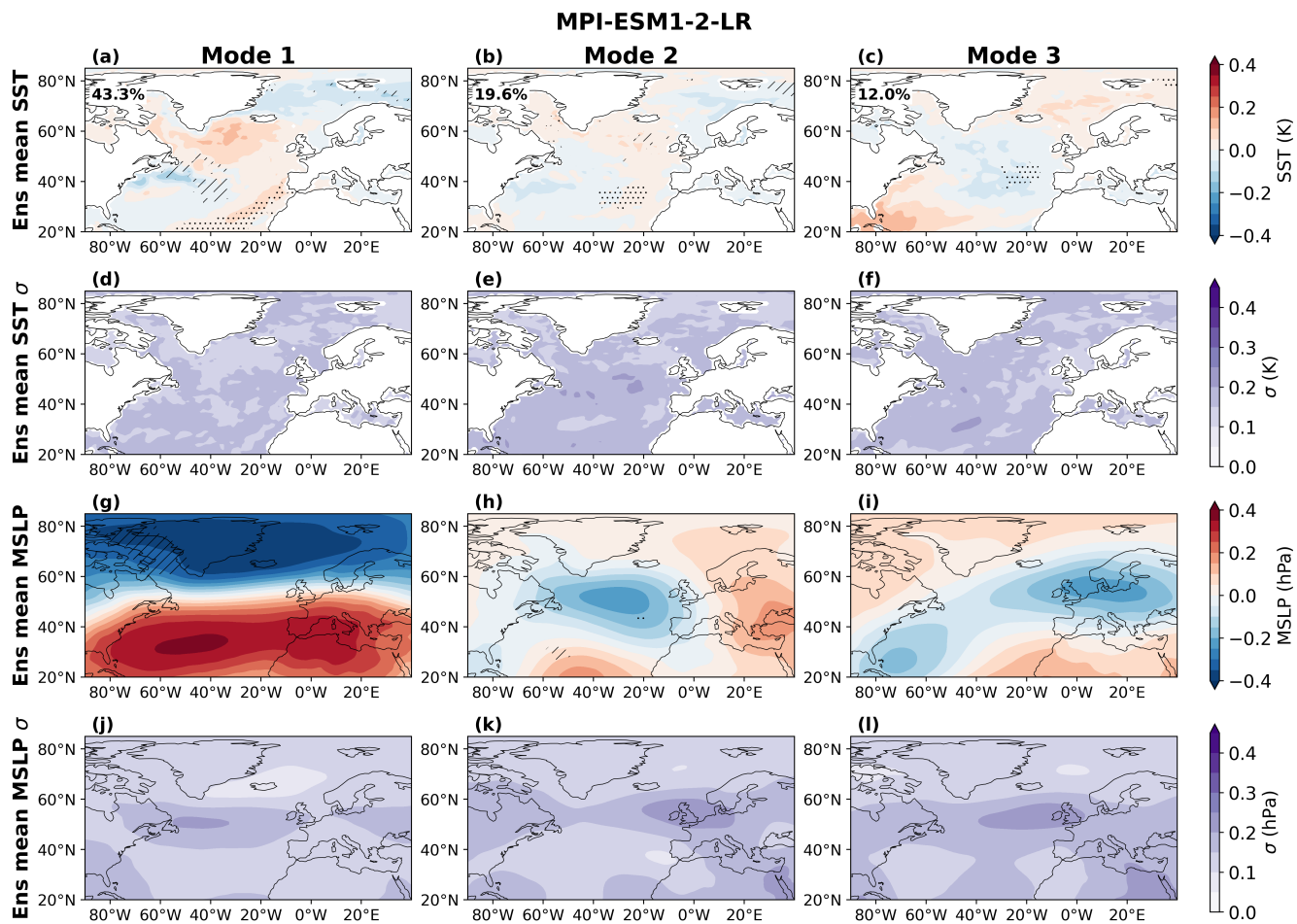
Figure S31. As in SI Fig.S20 for MPI-ESM1-2-LR.
