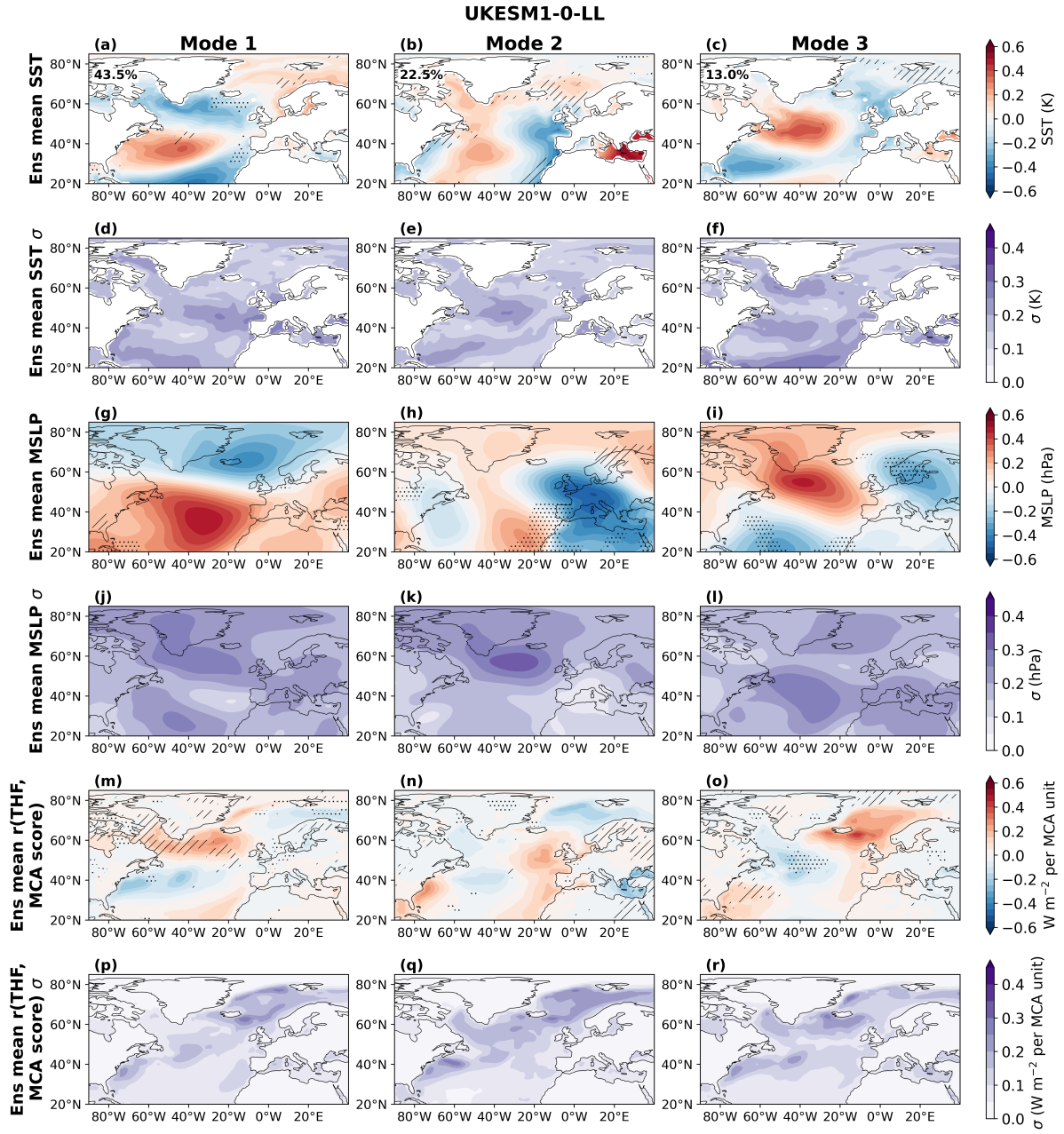
Figure S16. As in SI Fig. S3 for UKESM1-0-LL.
