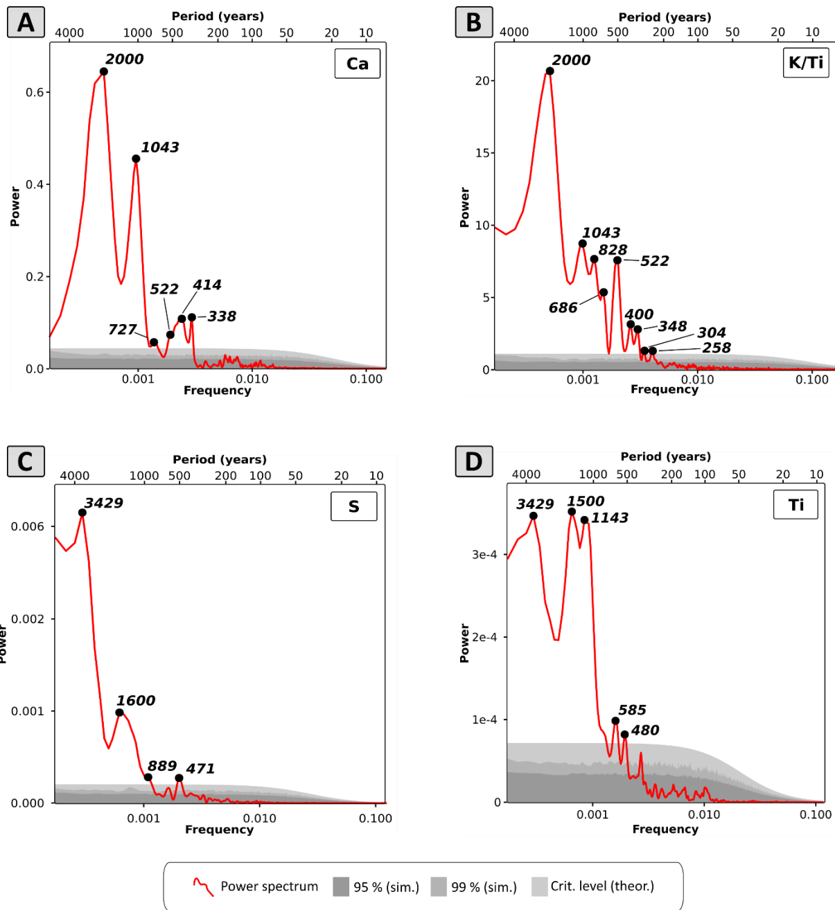
Figure 3: Redfit periodograms with significance levels of selected and calibrated cs-XRF proxies a) Ca (RPG 1), b) K/Ti ratio (RPG 1), c) S (RPG 2) and d) Ti (RPG 2). Black dots with numbers show local peaks with periodicity in years that are significant at the highest critical level. Note: X-axis is on logarithmic scale.
