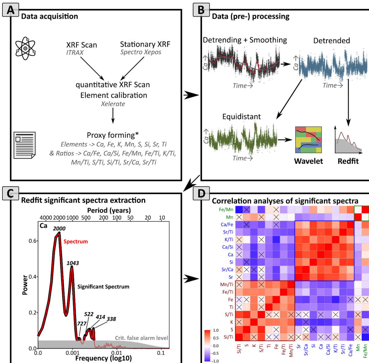
Figure 2: Flowchart of the high resolution XRF methodological approach. A) Acquisition of high resolution XRF data, calibration and forming elements and elemental ratios. *Proxy choice was done by common and published palaeolimnological XRF proxies (Cohen, 2003; Davies et al., 2015). B) Processing of high-resolution data for time series (Redfit and Wavelet) analyses, by detrending and equidistant resampling (precondition for Wavelet analyses). C) Extraction of significant (line above the critical Level of the AR1 red noise) Redfit power spectra of each proxy. D) Correlation analysis of the significant Redfit power spectra using the Spearman coefficient. The crosses show the non-significant (0.05 level) correlation values.
