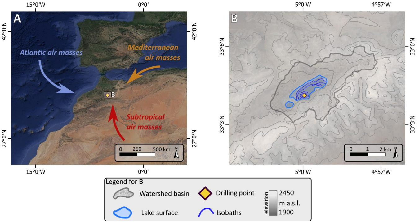
Figure 1: Geographical, climatological and topographical context of the study area. A) Location of Lake Sidi Ali in the Western Mediterranean / Northwest African context. The three major air masses influencing the Middle Atlas hydroclimate are indicated by the coloured arrows. B) Local topographical context of Lake Sidi Ali based on SRTM (NASA Shuttle Radar Topography Mission (SRTM), 2013). The contour lines have a vertical spacing of 50 m. Isobath intervals are not evenly spaced. Both panels are underlain by Google Earth satellite images (Image data: © NASA 2024, maps data: © Google 2024) (EPSG: 4326).
