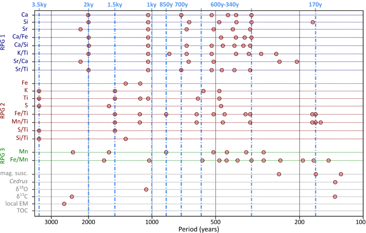
245 Figure 4: Synoptic graph of the positive peaks of the significant Redfit spectra of each XRF and non-XRF proxy. The x-axis is log 10 scaled, reflects the period and the red dots show the position of the peaks. The configuration and grouping of the XRF proxies follow the results from the correlation analysis (Redfit Proxy Groups). The blue dotted lines (with labels on top of the graph) show dominant modes of periodicity of the presented proxies.
