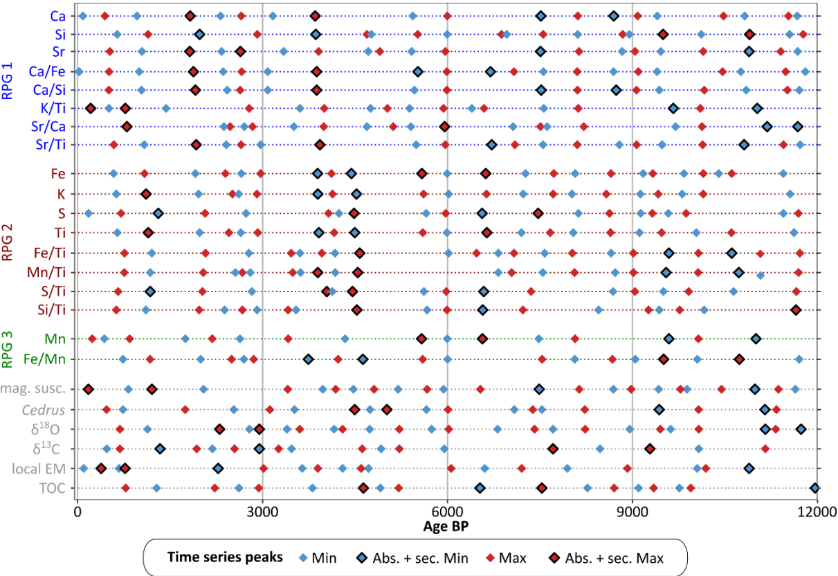
265 Figure 5: Temporal distribution of major minima and maxima derived from the smoothed proxy time series throughout the Holocene. Red diamonds indicate local maxima and blue diamonds local minima of the individual proxy records after 500-year kernel smoothing. Encircled symbols mark the dominant absolute and secondary extrema of each proxy series. The arrangement of the proxies follows the Redfit Proxy Groups (RPGs) identified from the correlation analysis of the significant spectral power. Grey-labelled proxies represent independent non-XRF datasets. The figure highlights similarities and contrasts in long-term temporal
