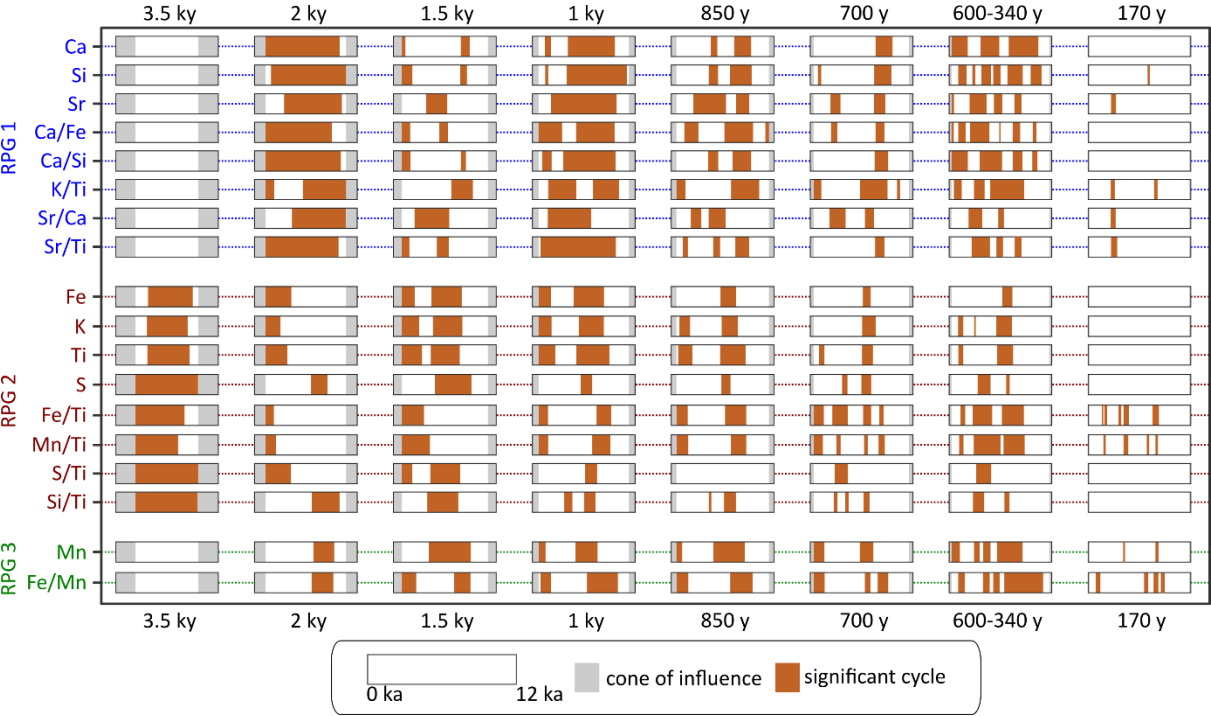
Figure 7: Synoptic graph of extracted significant wavelet power spectra of each proxy. The configuration and grouping of the proxies follow the results from the correlation analysis (Redfit Proxy Groups). The columns of the graph represent the main modes from the Redfit synoptic results (blue, dashed lines in Fig. 4). Each box reflects the whole Holocene time series. Grey bars show the cone of influence, where no significant wavelet periods were calculated due to edge effects. The red-brown colour shows the appearance of the specific cycle (see columns) throughout the Holocene, which occur within the 0.05 significance level and have a power value higher than the 80 % quantile.
