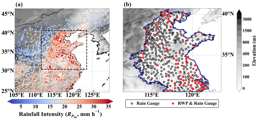
Figure 1. (a) Spatial distribution of 99 th -percentile hourly rainfall intensity ( R_{P99} ; \text{mm h}^{-1} ) at rain gauges across eastern China during the warm seasons (June–September) of 2021–2025. Grayscale shading represents terrain elevation, and the dashed black rectangle marks the subdomain zoomed in panel (b). (b) Enlarged view of the study domain covering the eastern China plains. The dark blue contour denotes areas within 111.5–123.5°E and 30.5–40.7°N with terrain elevation at or below 200 m. Open black circles indicate standalone rain gauge sites, while red filled circles mark co-located radar wind profiler (RWP) and rain-gauge stations.
