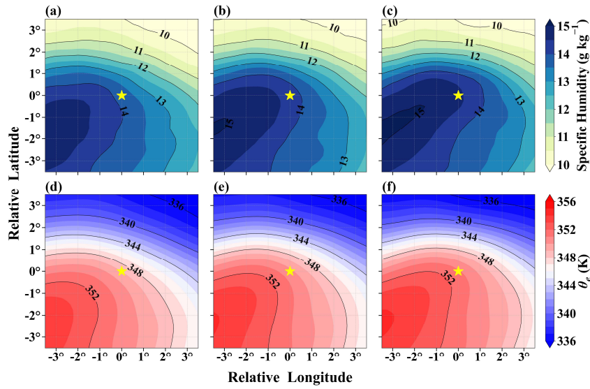
Figure 7. Composite 850-hPa specific humidity (a–c; shading, \text{g kg}^{-1} ; contours every 1 \text{ g kg}^{-1} ) and pseudo-equivalent potential temperature \theta_e (d–f; shading, K; contours every 4 K) fields for WSHR events, centered on the event target station (yellow star at origin). Columns correspond to 6 h before onset (a, d), 3 h before onset (b, e), and the onset hour (c, f).
