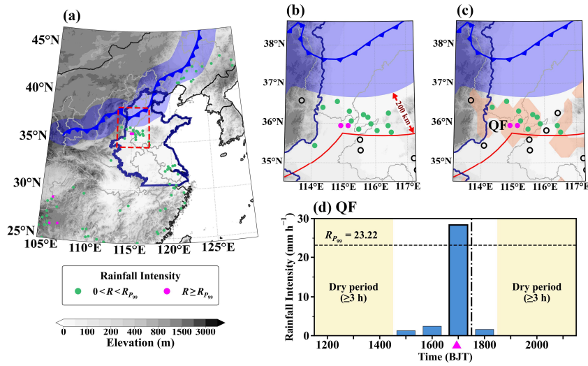
Figure 3. Example of an identified WSHR event at Qingfeng (QF) weather station on August 18, 2023. (a) Cold front (blue line) and its 200-km frontal zone (blue shading) at 1700 Beijing Time (BJT), with station rainfall overlaid (green dots: 0 < R < R_{p99} ; magenta dots: R \geq R_{p99} ). (b) and (c) Enlarged views of the red dashed rectangle in (a): (b) shows rainfall at stations 200–400 km from the front (the warm-sector candidate region); (c) additionally shows the warm-sector mask (orange shading) and rainfall at stations falling within it. Open black circles denote stations with rainfall ( R > 0 ) that fall outside the study region or fail the warm-sector criteria. (d) Hourly rainfall time series at QF station. The dashed line marks R_{p99} = 23.22 \text{ mm h}^{-1} ; the dash-dotted line marks the first hour reaching R_{p99} , with all rainfall hours from onset to this hour required to lie within the warm sector. Yellow shading denotes dry periods ( \geq 3 \text{ h} ) bounding the event, and the magenta triangle marks the hour identified as WSHR.
