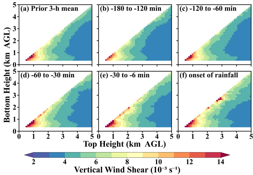
Figure 10. Composite vertical wind shear (shading, 10^{-3} \text{ s}^{-1} ) preceding the onset of WSHR events. (a) prior 3-h mean, (b) -180 to -120 min, (c) -120 to -60 min, (d) -60 to -30 min, (e) -30 to -6 min, and (f) the onset of rainfall. The abscissa and ordinate denote the top and bottom heights (km AGL), respectively, of the layer over which the bulk shear is computed.
