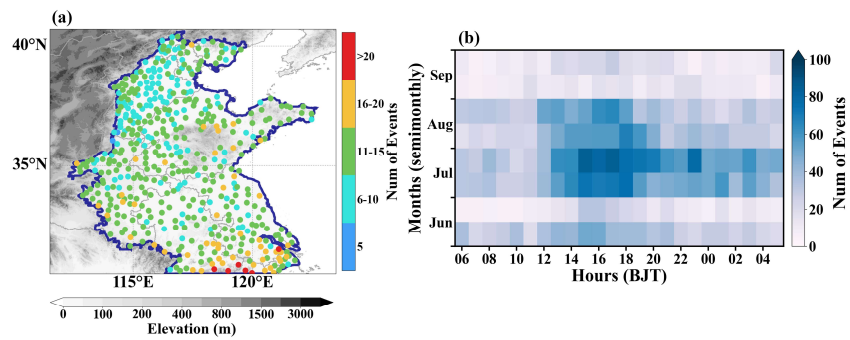
1096 Figure 5. Same as Fig. 4, but for other heavy rainfall events.
