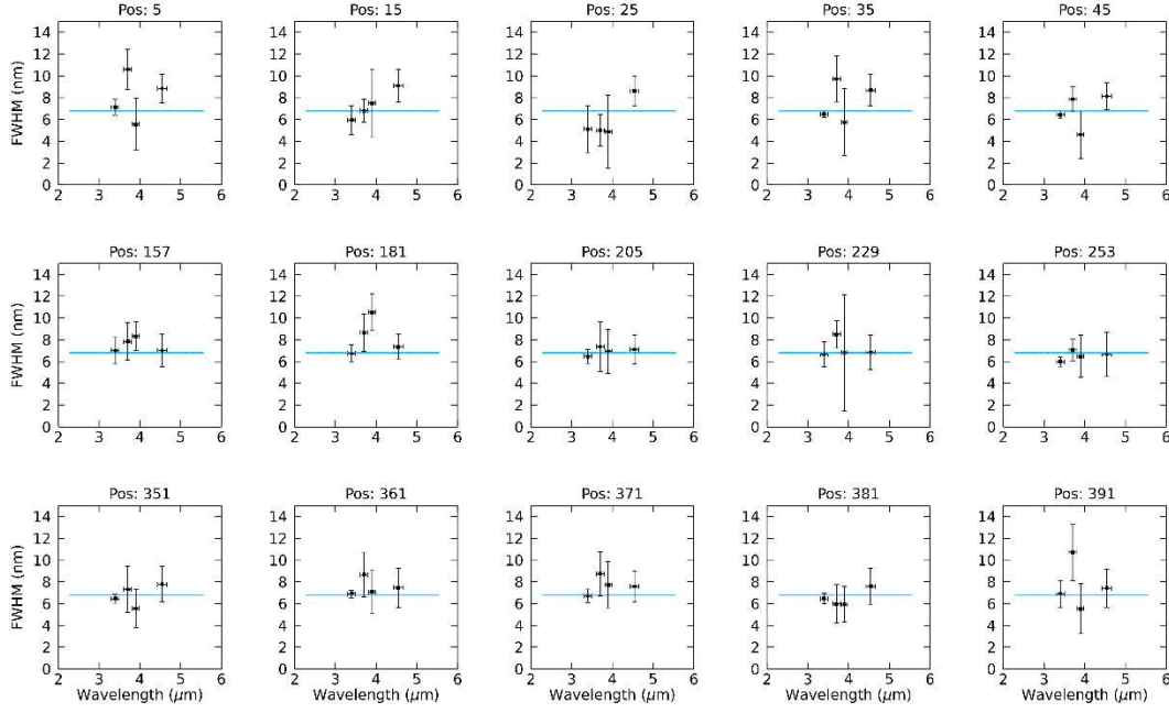
Figure A2. Same as Figure A1 but for the FWHM estimation from the joint retrievals of the spectral residual and FWHM. The blue line shows the reference FWHM in the IR channel (a constant 6.8 nm value in the case of nominal pixels) as recommended by Haffoud et al. (2024) from on-ground calibration measurements.
