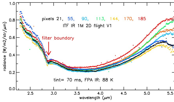
Figure 10. Radiance spectra of the Moon obtained over the left half of the FOV after the first stage of ITF adjustment. The 7 spectra correspond to MAJIS pixels (36 \mu\text{m} pitch) from pixel 600 21 (close to the left edge) to pixel 185 (close to the center of the 400 pixels FOV)
