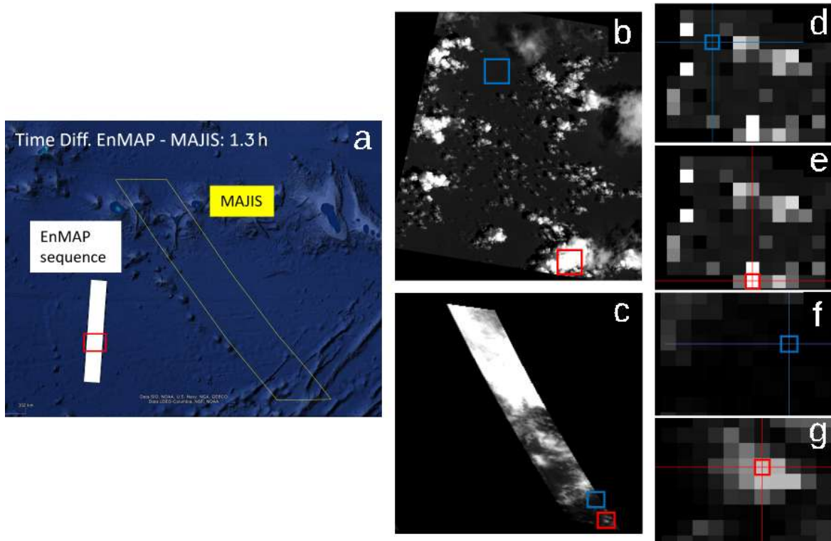
Figure 17. Panel (a): location of the ENMAP observation (white area) and the MAJIS observation (C17, yellow outline) over the Pacific Ocean; Panel (b): ENMAP radiance map at 0.75 \mu\text{m} for the red rectangle in panel A, with the locations of the areas selected as representative of cloudy (red) and cloud-free (blue) ENMAP data; Panel (c): Radiance map at 0.750 \mu\text{m} for the full MAJIS swath, with areas selected for cloudy (red) and cloud-free (blue) representative spectra. Panels (d), (e): Panel (b) resampled at the MAJIS resolution with the resampled pixels selected as representative of cloudy (red) and cloud-free (blue) areas; Panels (f), (g): Zoom on the red and blue areas in panel (c), indicating the MAJIS pixels selected as representative of cloud-free (blue) and cloudy (red) areas.
