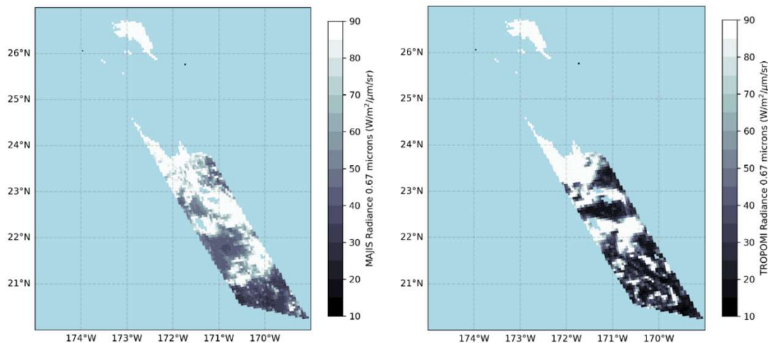
Figure 19. Weighted mean MAJIS radiances (left panel) and TROPOMI radiances (right panel) for the areas covered by MAJIS observation C17 (20/08/2024, 21:48 UTC) in the TROPOMI band 5 wavelength range. The TROPOMI data was collected 3 hours later. MAJIS and TROPOMI radiances corresponding to MAJIS saturated pixels have not been displayed. The
