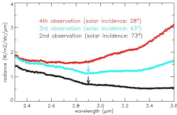
Figure 12. MAJIS radiance spectra obtained during three of the five observations of the Moon by MAJIS (see Poulet et al., 2026) applying the updated IR 2D-ITF. Blue and black arrows
