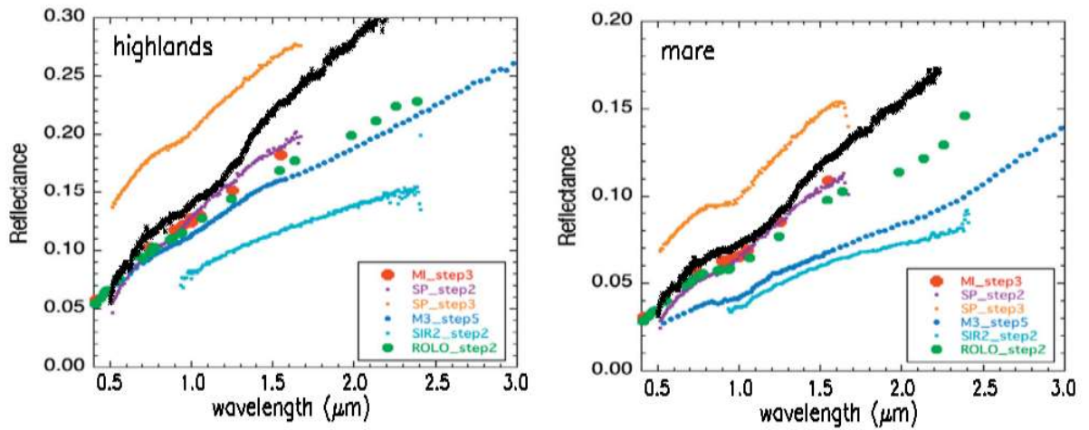
Figure 15. lunar reflectance spectra from MAJIS observations (black stars) in the VISNIR spectral range (0.5 – 2.250 μm) corrected for straylight and assuming Lambert scattering for highlands (left panel) and for mare (right panel) compared to lunar reflectance spectra of highlands and mare obtained by other instruments (Ohtake et al., 2013).
