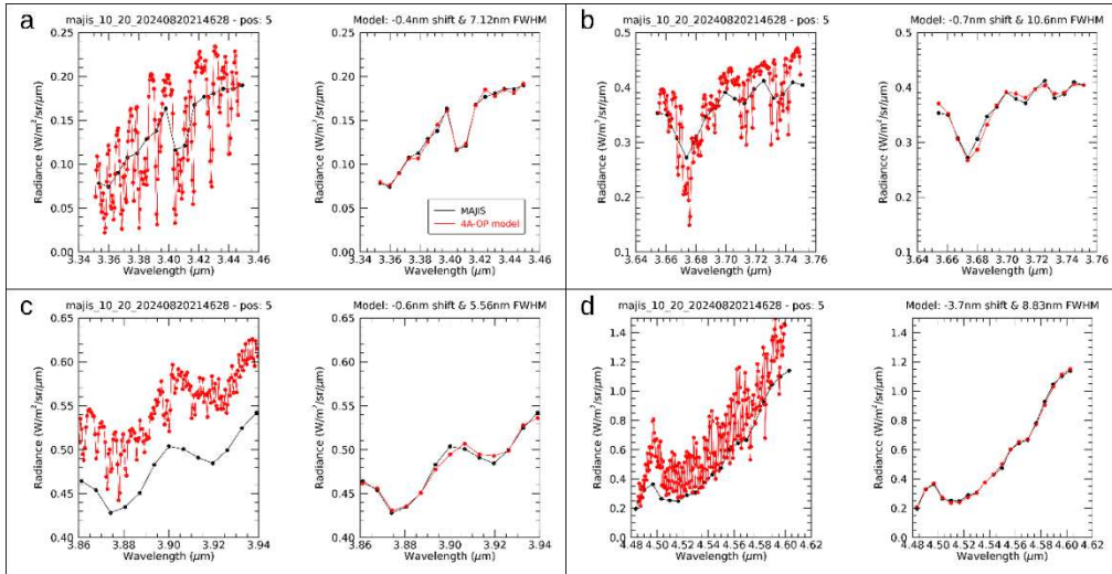
Figure 5. Examples of simultaneous retrievals of the spectral residual and the spectral width (FWHM) in 4 spectral ranges within the MAJIS IR channel, for the position 5 (in nominal pixels) of the MAJIS slit. Each spectral range includes a specific absorption band used for constraining both the CWL and FWHM at the nominal pixel level within the wavelength range of the IR channel; Panel (a): residuals and FWHM retrievals for the interval 3.35-3.45 \mu\text{m} including the \text{CH}_4 band at 3.4 \mu\text{m} . The black lines and dots display a MAJIS spectrum extracted from the cube C15 (#20240820214628) at the across- x along-slit position [10, 5] in nominal pixels. Red lines and dots present the results of the 4A/OP model adapted to match the
