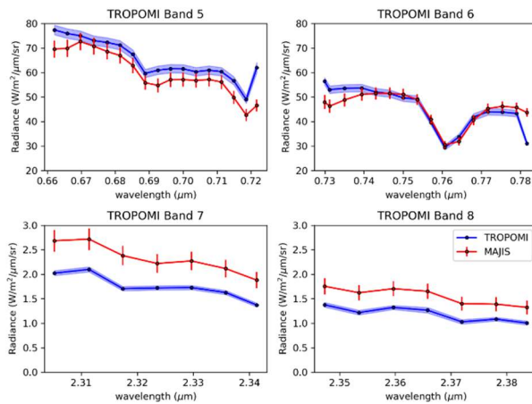
Figure 20. Averaged results of collocated TROPOMI and MAJIS radiances for MAJIS observations C15 and C17. The blue shaded area represents the TROPOMI total uncertainty, and the red error bars represent the MAJIS total uncertainty, the largest contribution resulting from the variability within sets of co-located MAJIS pixels corresponding to a single TROPOMI pixel.
