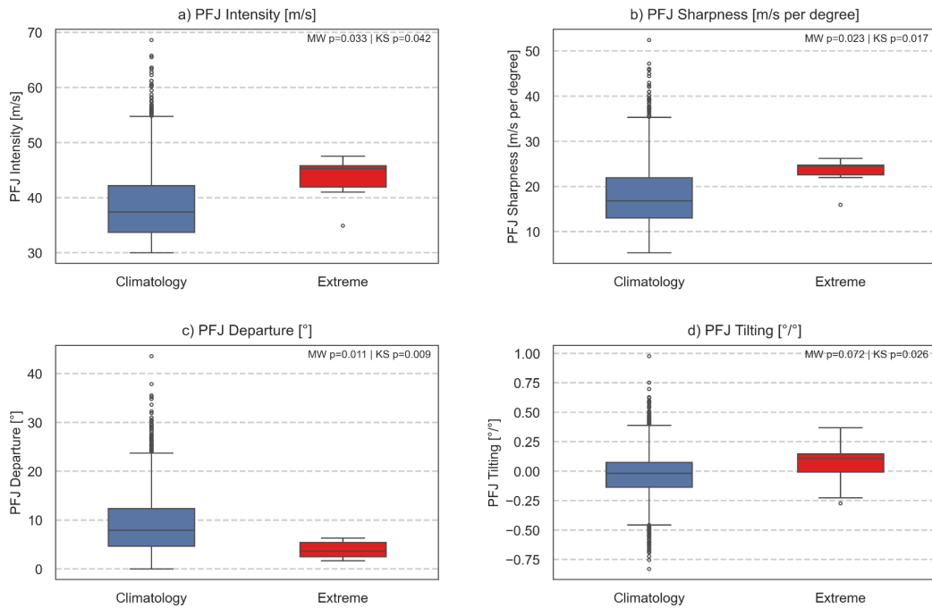
Figure 2: Southern Hemisphere jet diagnostics during extreme-swell events E1–E5 (MJJAS). Boxplots of polar-front jet (PFJ) significant metrics for event days (red) versus austral winter climatology (blue) from ERA5 250-hPa winds: (a) PFJ intensity, (b) PFJ sharpness, (c) PFJ departure and (d) PFJ tilting. P-values from Mann–Whitney and Kolmogorov–Smirnov tests are shown above panels; robustness to unequal sample size is assessed in Table S4 and Fig. S6 (Supplement).
