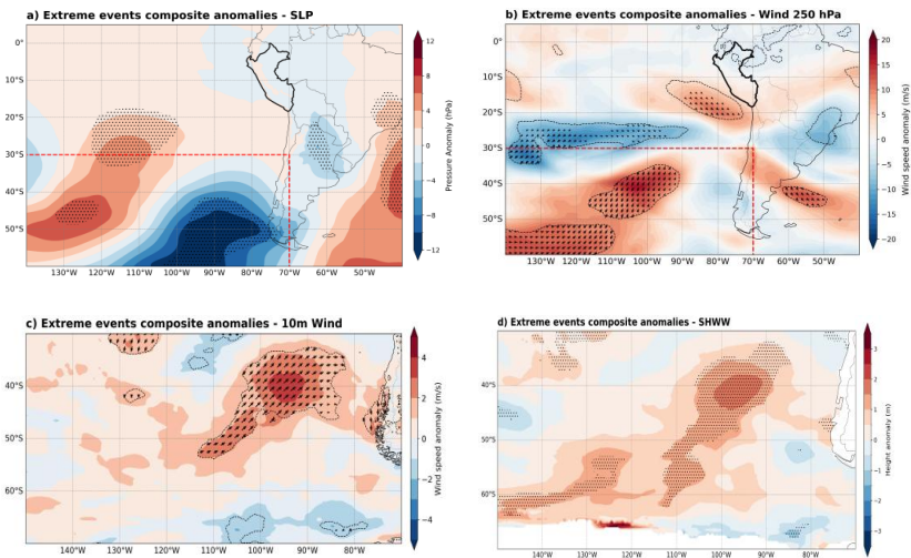
202 Figure 1: Southern Hemisphere composite anomalies during extreme-swell events (E1-E5; MJJAS). Panels (a)–(b) show large- 203 scale conditions over 140°W–40°W and 5°N–60°S: (a) sea-level pressure (SLP) anomaly (shading) and (b) 250-hPa wind-speed 204 anomaly (shading) with wind-anomaly vectors. The red boxes in (a) and (b) indicate the regional domain analyzed in (c) 205 and (d) (150°W–70°W, 30°–70°S): (c) 10-m wind-speed anomaly (shading) with wind-anomaly vectors and (d) significant height of 206 wind waves (SHWW) anomaly (shading). Anomalies are computed relative to the 1991–2020 MJJAS climatology and averaged 207 over days D-4 to D-3 relative to day D0. Statistical significance at p < 0.05 (two-sided Mann–Whitney U test) is indicated by 208 stippling in (a) and (d), and by dashed contours enclosing the wind vectors in (b) and (c). The Peruvian coastline is outlined to 209 indicate the impacted coastal sector.
