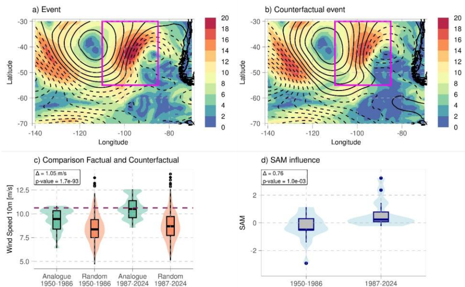
Figure 3: Analogue analysis for the E1 event. (a) Wind speed at 10-m (shaded) and SLP (contours) observed during E1 in the ERA5 reanalysis. Dashed contours indicate pressures below 1013 hPa. (b) Counterfactual reconstruction of 10-m winds (shading) and SLP (contours), obtained by removing the climate-change signal—defined as the median differences between present and past analogue flows—from the observed event. (c) Mean wind speed at 10m over the box, indicated in panels (a) and (b), reconstructed from flow analogues (green) and random (orange) days of the past (1950-1986) and present (1987-2024) period. The dotted horizontal line indicates the intensity of the event observed in ERA5. The legend shows the difference in medians between the present and past periods for wind speed at 10-m for days with similar flow and its statistical significance according to the Mann-Whitney U test. (d) Monthly SAM associated with days with flow analogues for the past and present periods. The difference between medians for both periods and statistical significance is indicated in the legend.
