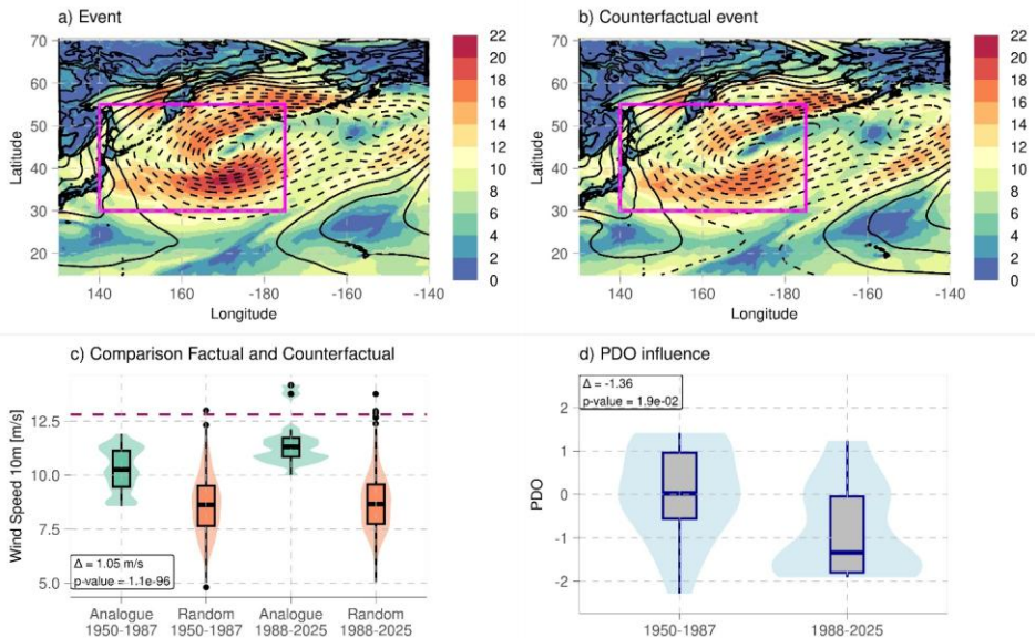
Figure 7. Same as figure 6 for the E9 event.
