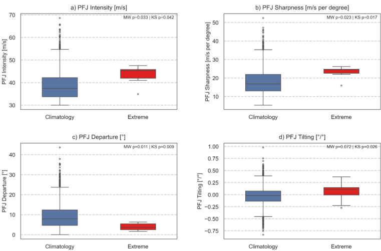
Figure 2: Southern Hemisphere jet diagnostics during extreme-swell events E1–E5 (MJJAS). Boxplots of polar-front jet (PFJ) significant metrics for event days (red) versus austral winter climatology (blue) from ERA5 250-hPa winds: (a) PFJ intensity, (b)
