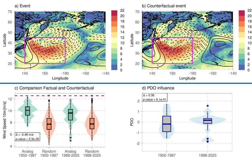
Figure 6. Analogue analysis for the E7 event. (a) Wind speed at 10-m (shaded) and SLP (contours) observed during E7 in the ERA5 reanalysis. Dashed contours indicate pressures below 1013 hPa. (b) Counterfactual reconstruction of 10-m winds (shading) and SLP (contours), obtained by removing the climate-change signal—defined as the median differences between present and past analogue flows—from the observed event. (c) Mean wind speed at 10m over the box, indicated in panels (a) and (b), reconstructed from flow analogues (green) and random (orange) days of the past (1950-1987) and present (1988-2025) period. The dotted horizontal line indicates the intensity of the event observed in ERA5. The box shows the difference in medians between the present and past periods for wind speed at 10-m for days with similar flow and its statistical significance according to the Mann-Whitney U test. (d) Monthly PDO associated with days with flow analogues for the past and present periods. The difference between medians for both periods and statistical significance is indicated in the box.
