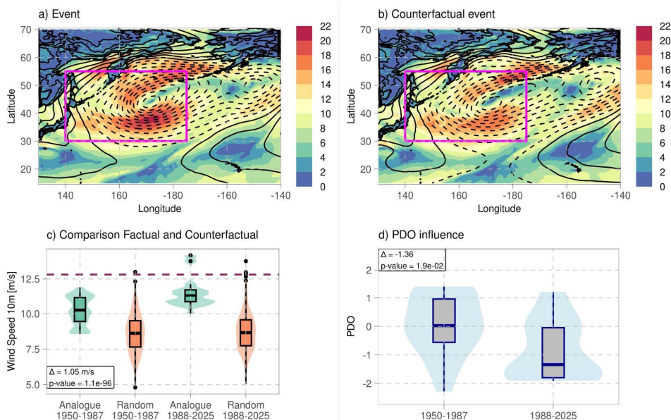
Figure 7. Same as figure 6 for the E9 event.
