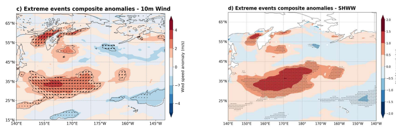
Figure 4: Northern Hemisphere composite anomalies during extreme-swell events (E6–E11; DJFM). Panels (a)–(b) show basin-scale anomalies over 140°E–70°W and 80°N–60°S, averaged over days D–11 to D–38 relative to day D0: (a) sea-level pressure (SLP) anomaly (shading) and (b) 250-hPa wind-speed anomaly (shading) with wind-anomaly vectors. Panels (c)–(d) show a zoomed view of the North Pacific swell-source region (140°E–140°W, 15°–70°N): (c) 10-m wind-speed anomaly (shading) with wind-anomaly vectors and (d) significant height of wind waves (SHWW) anomaly (shading). Anomalies are computed relative to the 1991–2020 DJFM climatology. Statistical significance at p < 0.05 (two-sided Mann–Whitney U test) is indicated by stippling in (a) and (d), and by dashed contours enclosing the wind vectors in (b) and (c). The Peru outline is highlighted for reference.
