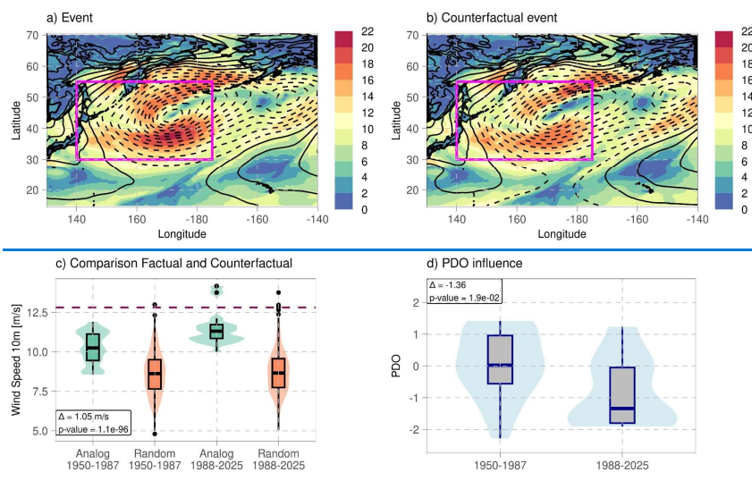
502 Figure 7. Same as figure 6 for the E9 event.
