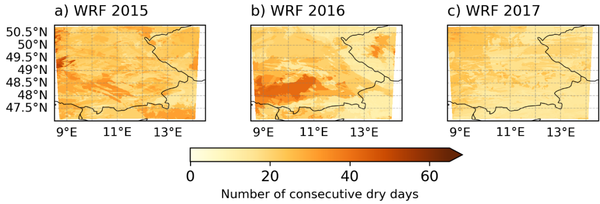
Figure S1: Number of consecutive dry days in 2015 (a), 2016 (b), and 2017 (c) based on the convection-permitting 1.5 km resolution WRF simulation by Collier & Mölg (2020).
