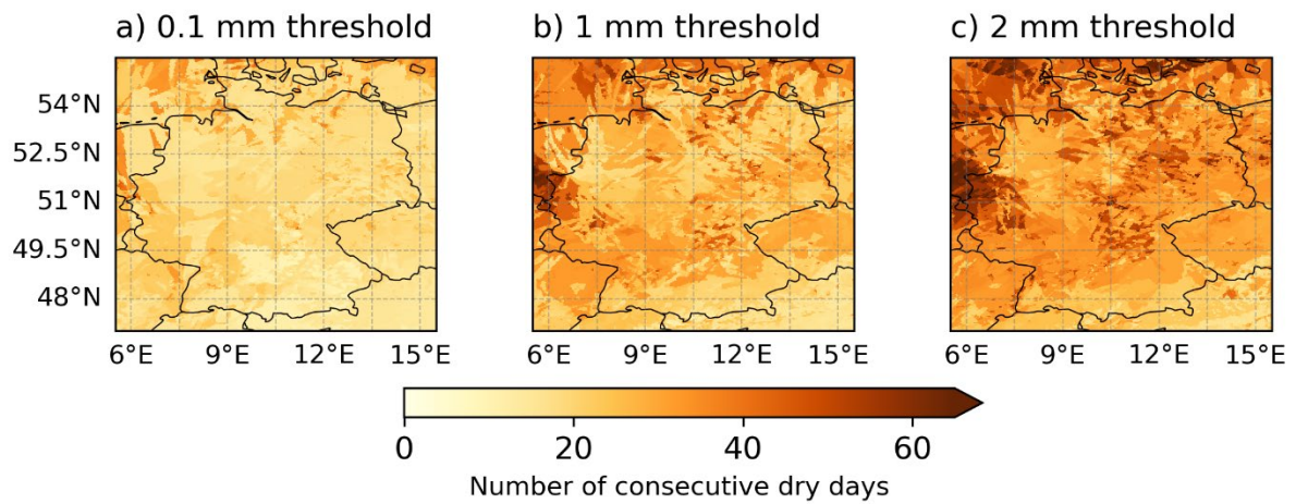
Figure S2: Number of consecutive dry days in 2018 for convection-permitting simulations of COSMO-CLM using a dryness threshold of 0.1 mm (a), 1 mm (b), and 2 mm (c).
