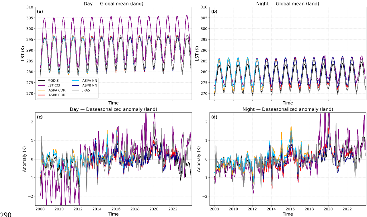
Figure 1. Global mean land surface temperature (LST, panels a and b) and deseasonalised anomalies (panels c and d) for daytime (left) and nighttime (right). IASI Metop-A and Metop-B observations (IASI-A/B) are shown separately for the CDR and NN products. Global means are computed using cosine-latitude weighting.
