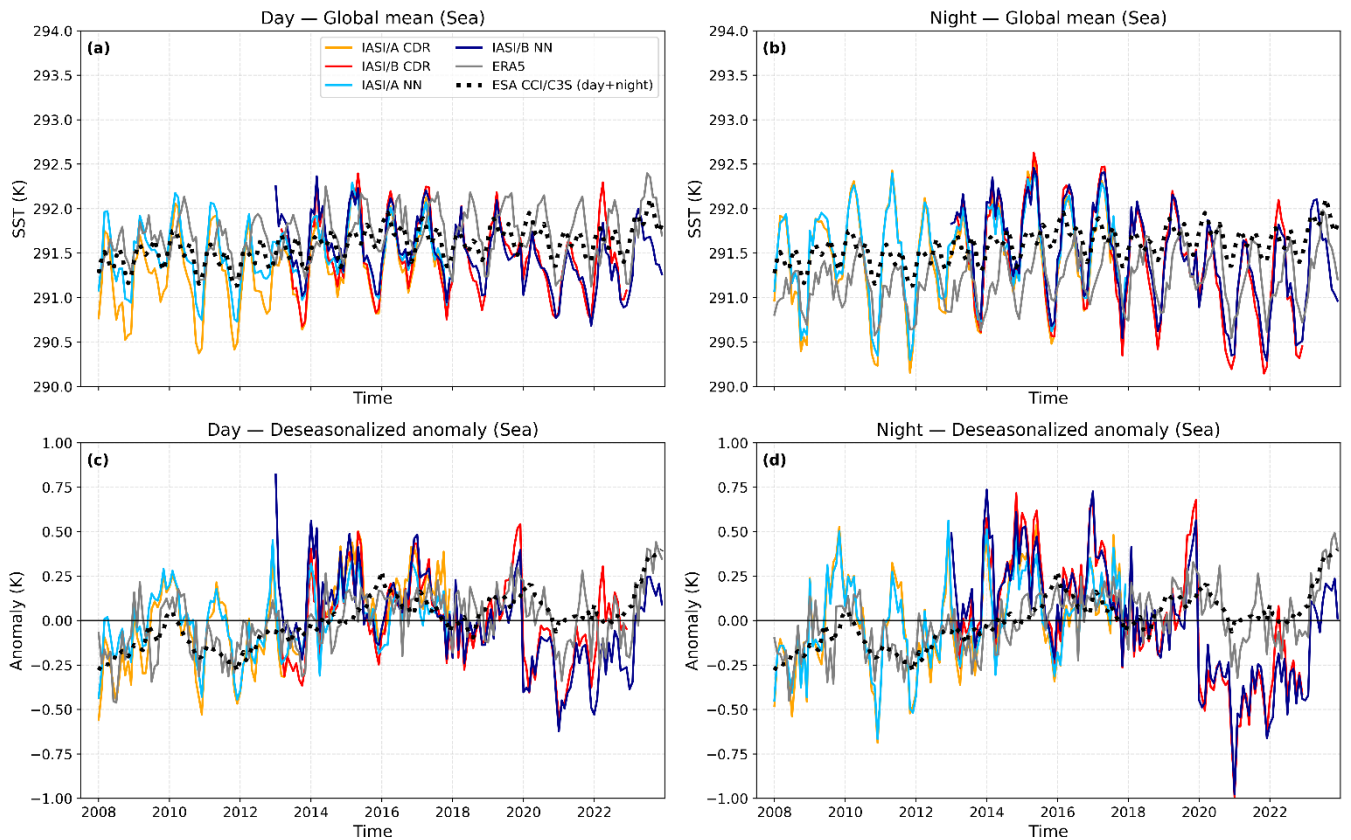
380 Figure 4. Upper panels: SST global mean during the day (panel a) and the night (panel b) for ERA5, IASI-CDR and IASI-NN, and ERA5 CCI and C3S SST all-sky product which is shown in dotted black line. It is the same for the day and night panels as it is a combined product. IASI data are separated between Metop A and Metop B. Lower panels: the deseasonalized anomaly of SST for the different products, during the day (panel c) and night (panel d). Global means are computed using cosine-latitude weighting.
