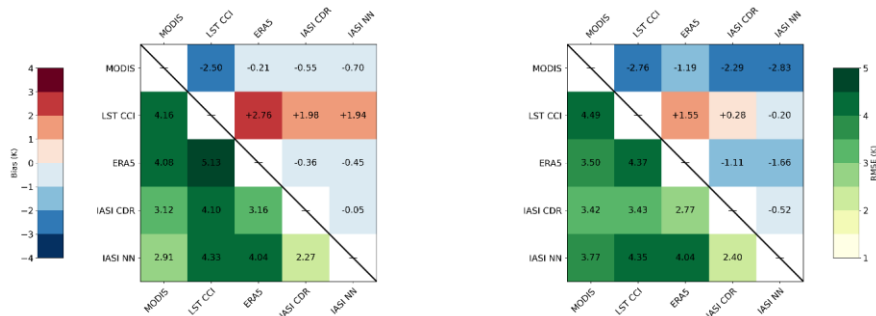
Figure 3. Upper triangle (blue to red): global mean bias (row – column, y-x ); Lower triangle (in yellow to green): root mean square error (RMSE) between the different pairs of LST datasets, for daytime (left) and nighttime (right). Statistics are computed over land grid cells only (using the ERA5 land sea mask) and weighted by cosine-latitude.
