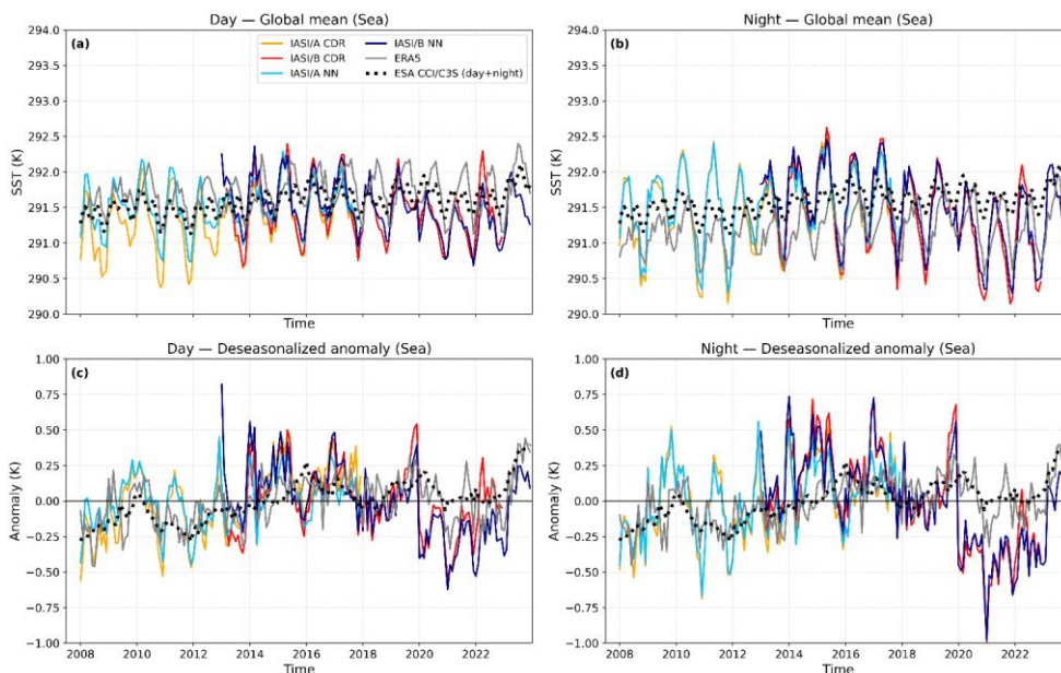
Figure 4. Upper panels: SST global mean during the day (panel a left) and the night (panel b right) for ERA5, IASI-CDR and IASI-NN, and ERA5 CCI and C3S SST all-sky product which is shown in dotted black line. It is the same for the day and night panels as it is a combined product. IASI data are separated between Metop A and Metop B. Lower panels: the deseasonalized deseasonalized anomaly of SST for the different products, during the day (panel c) and night (panel d). Global means are computed using cosine-latitude weighting.
