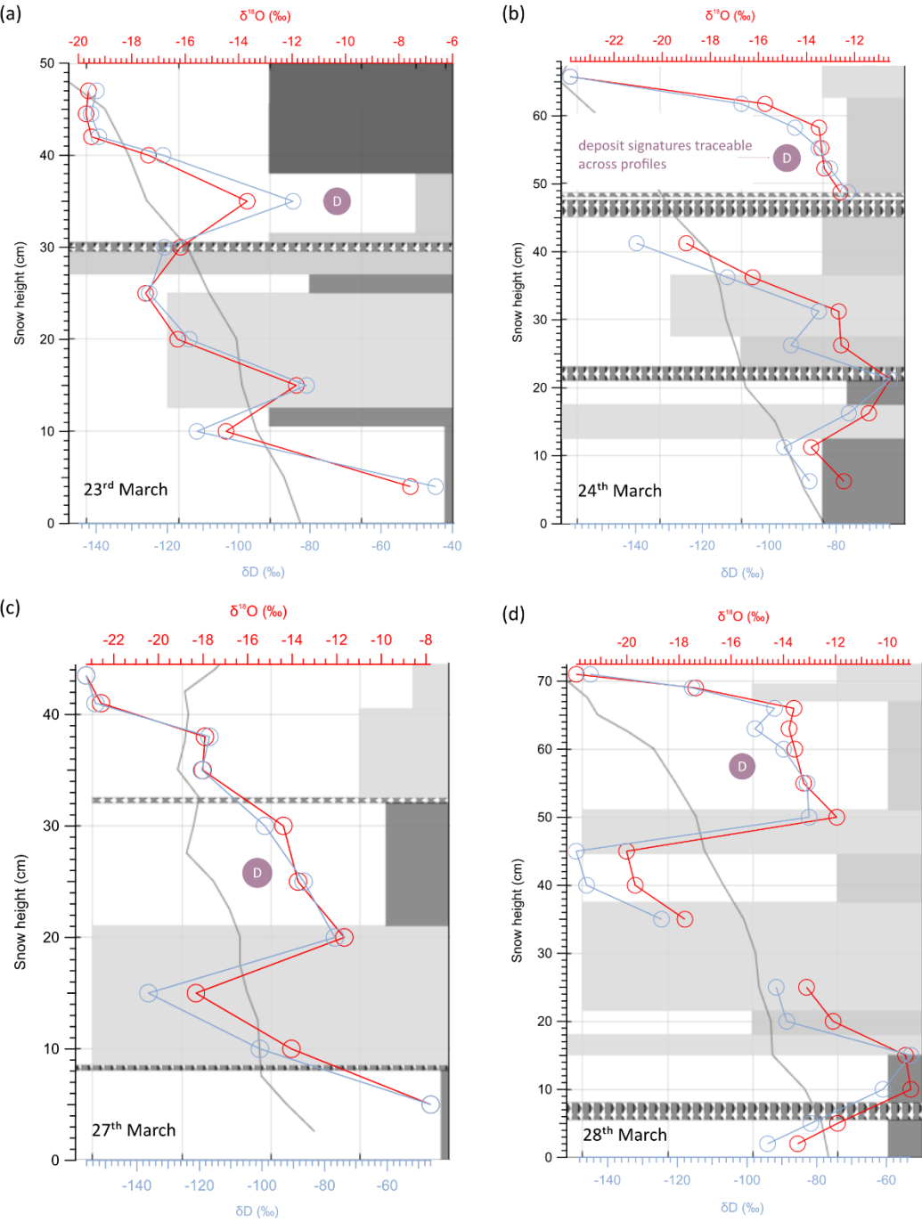
Figure D1: Overview of stable water isotope signatures \delta^{18}\text{O} (red) and \delta\text{D} (blue) with depth prior to melt experiments in March 2023, against the background of grey-coloured stratigraphy based on layer hardness.
