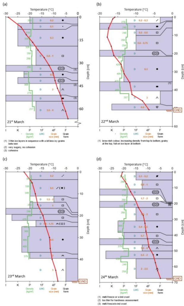
Appendix- Figure C1: Overview of snow profile characteristics prior to melt experiments in March 2023, categories based on Fierz et al. (2009).
