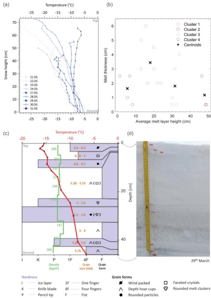
240 Figure 4: Snowpack characteristics as assessed prior to tracer percolation experiments: (a) temperature profiles plotted with-versus snow height above ground; (b) K-means based clustering of melt layers in the local snowpack based on their thickness and height above ground across all snow pits; (c–d) snow pit example of 29 th March 2023: (c) snow stratigraphy with depth (niViz plot), including temperature, hardness, density, grain size and grain shape, symbols based on Fierz et al. (2009) explained in legend below, with (d) corresponding digital photo of snow pit wall with red markers for each layer boundary.
