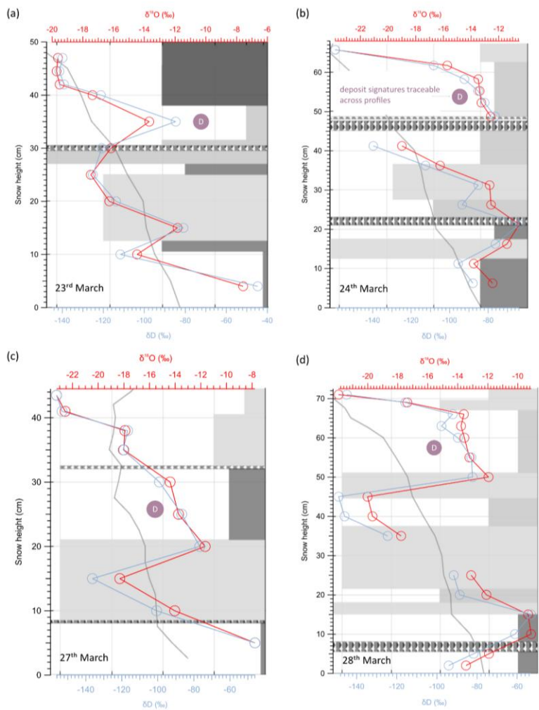
600 Appendix Figure D1: Overview of stable water isotope signatures \delta^{18}\text{O} (red) and \delta\text{D} (blue 2 H) with depth prior to melt experiments in March 2023 , against the background of grey-coloured stratigraphy based on layer hardness.
