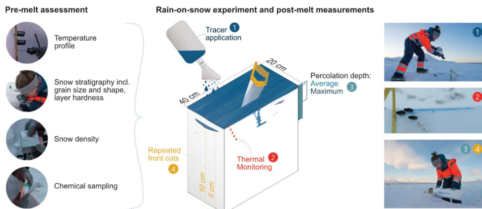
150 Figure 2: Overview of methodological steps before, during and after rain-on-snow experiments conducted near Ny-Ålesund in March 2023; left: photos of the pre-melt assessment steps; centre: schematic visualisation of tracer experiment snow pit setup and post-melt measurements as discussed in Sect. 2.2.2; right: photos of tracer application, temperature monitoring and percolation assessment on repeated front cuts obtained during fieldwork, credit for all photos: Iain Rudkin.
