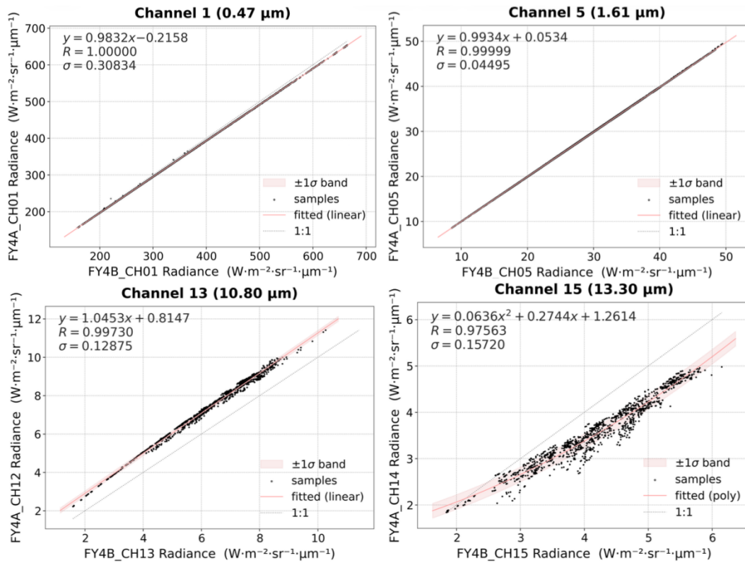
1285 Figure 3. Application of the new physics-constrained transfer learning framework from FY-4B to 1286 FY-4A AGRI radiance observations. From left to right, the panels show Channels 1 (0.47 \mu\text{m} ), 5 1287 (1.61 \mu\text{m} ), 13 (10.80 \mu\text{m} ), and 15 (13.30 \mu\text{m} ) (following the FY-4B channel designations). They 1288 demonstrate the framework’s linear fitting performance in the visible, near-infrared, and thermal 1289 infrared bands, as well as an example of higher-order polynomial fitting for FY-4B/AGRI Channel 1290 15 (13.30 \mu\text{m} ). R and \sigma denote the correlation coefficient and fitting residuals, respectively.
