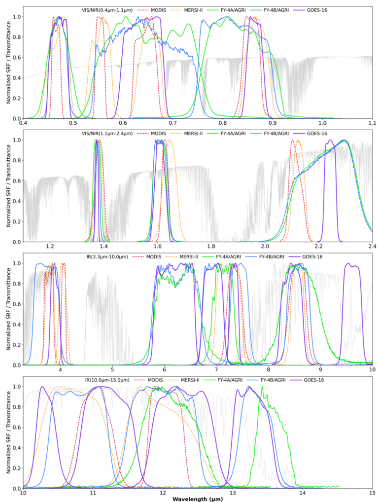
1349 Figure 2. Normalized Spectral response functions from the visible to infrared channels across 1350 China FY-4A/B GEO imagers (AGRI, Advanced Geosynchronous Radiation Imager, green/blue 1351 solid line), the U.S. GOES-16 GEO imager (Advanced Baseline Imager, ABI, purple solid line), 1352 China FY-3D polar-orbiting imager (MERSI-II, Medium Resolution Spectral Imager II, orange 1353 dashed line), and the U.S. Aqua/MODIS polar-orbiting sensor (cardinal red dashed line). The light 1354 gray solid curve in each subfigure denotes the simulated transmittance using the 1976 U.S. 1355 Standard Atmosphere profile.
