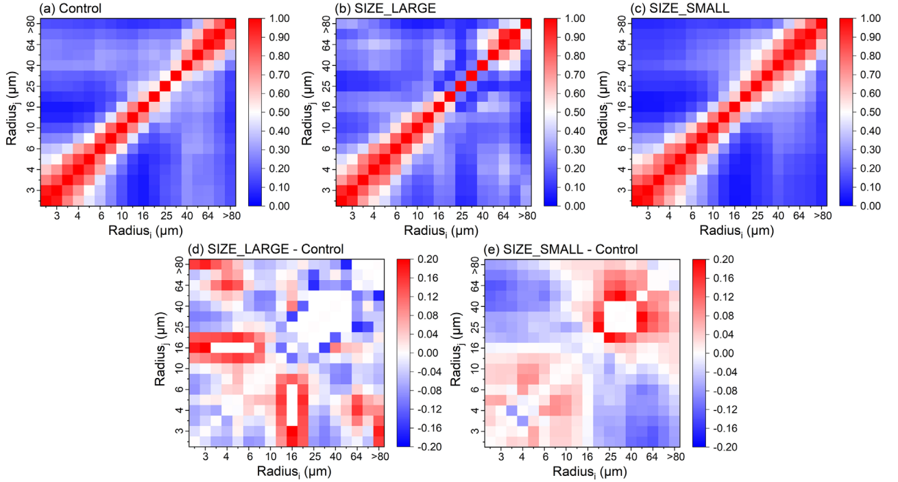
Figure 6. Correlation map between liquid droplets number concentrations in size bins i and j from the Control (a), SIZE_LARGE (b), and SIZE_SMALL (c) experiments, and differences of SIZE_LARGE (d) and SIZE_SMALL (e) with the Control. For each size bin, the four-dimensional (time, height, latitude, longitude) droplet number concentration field is first flattened into a one-dimensional array in the same order, and the Pearson correlation coefficient between bins i and j is then computed.
