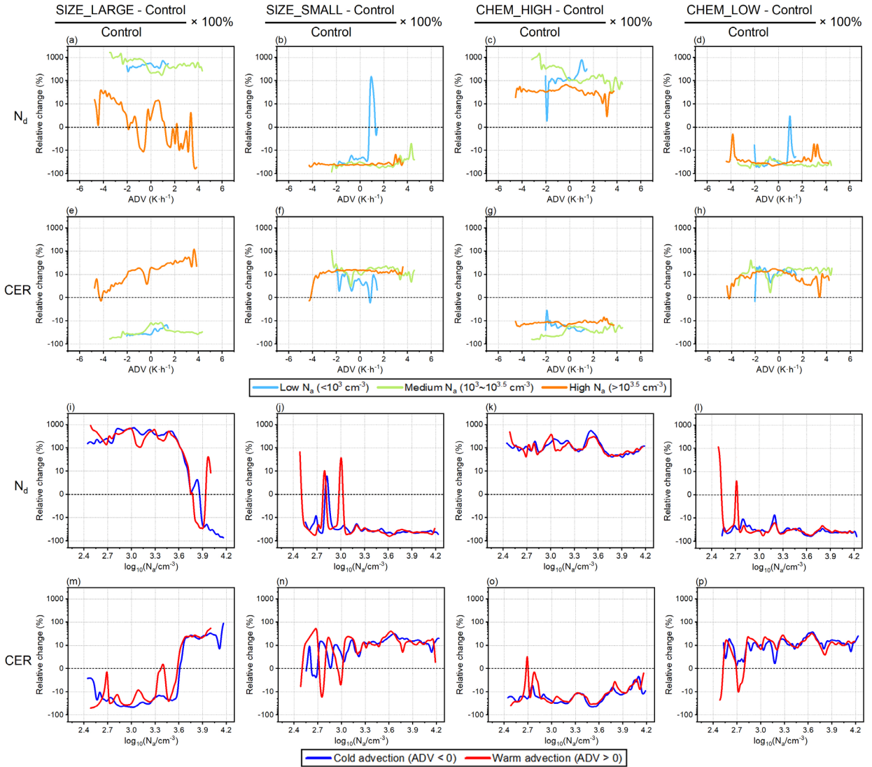
Figure 9. Percentage changes in N_d and CER for the sensitivity experiments relative to the Control experiment. Upper two rows: dependence on ADV (x axis) for different N_a conditions; lower two rows: dependence on N_a (x axis) for different ADV conditions.
