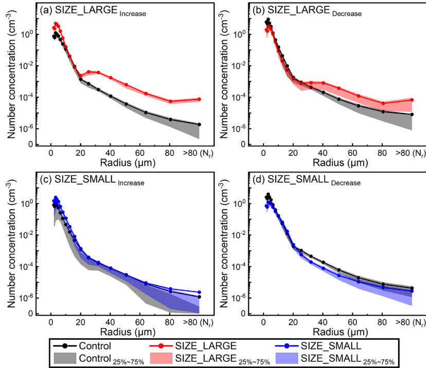
320 Figure 5. Changes in droplet spectra (lines, mean; shading, the 25-75% interquartile range; droplets with a radius greater than 80 \mu\text{m} are raindrops and those less than 80 \mu\text{m} are cloud droplets) for the samples with an increase (left column) or decrease (right column) in N_d of more than 0.1 \text{ cm}^{-3} , in response to increases (upper row) or decreases (lower row) in aerosol size.
