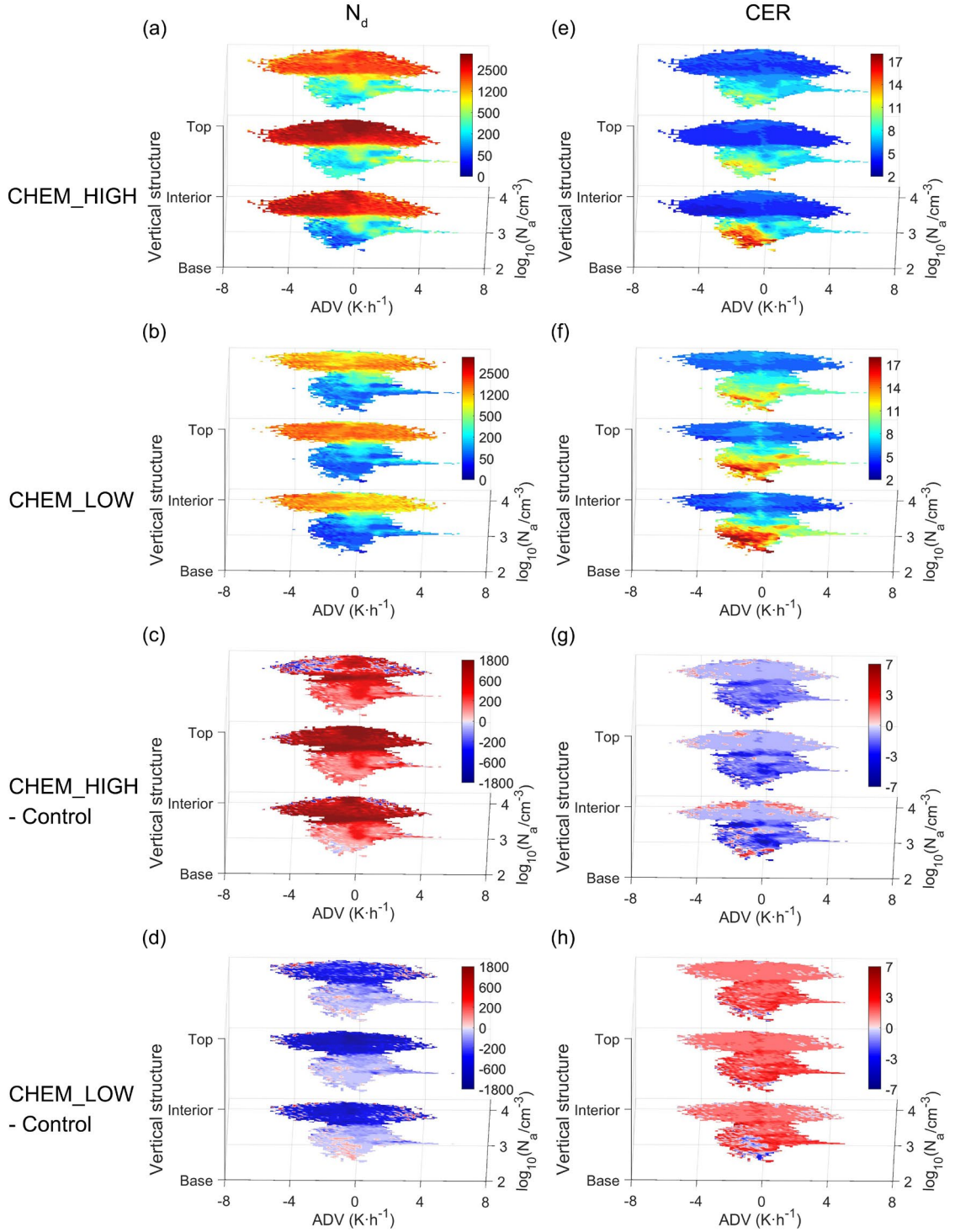
Figure 12. Variation of N_d (in \text{cm}^{-3} ) and CER (in \mu\text{m} ) with ADV, N_a and cloud parts for the CHEM_HIGH and CHEM_LOW experiments and their difference relative to the Control experiment.
