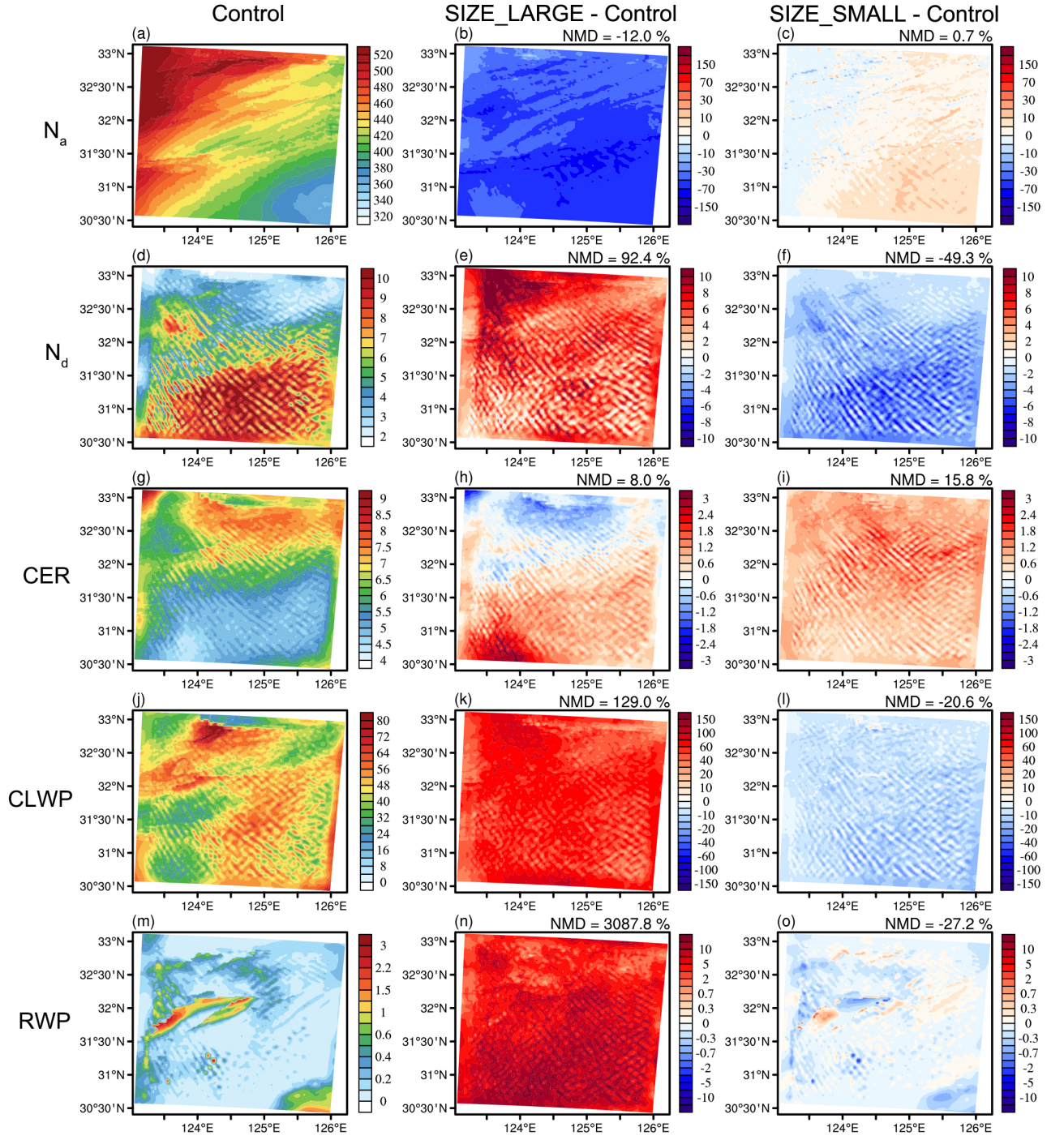
Figure 3. Spatial distributions of column-mean N_a (in \text{cm}^{-3} ) and N_d (in \text{cm}^{-3} ), mean CER (in \mu\text{m} ), CLWP (in \text{g m}^{-2} ), and RWP (in \text{g m}^{-2} ) averaged over the simulation period from the Control experiment (left column), and differences of SIZE_LARGE (middle column) and SIZE_SMALL (right column) relative to the Control (NMD of each sensitivity experiment relative to the Control is indicated at the top-right of each subplot). Values represent liquid-phase clouds averaged over the simulation period, and grid points without clouds or with non-liquid-phase clouds are excluded. N_a and N_d are column averages, CLWP and RWP are column totals, and CER is calculated based on the droplet number in each bin.
