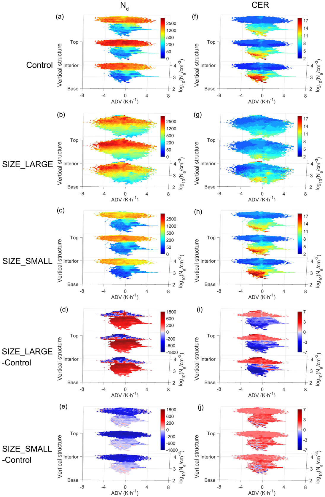
Figure 4. Variation of N_d (in \text{cm}^{-3} ) and CER (in \mu\text{m} ) of liquid-phase clouds with N_a , ADV and cloud parts in the three experiments, and the difference of the SIZE_LARGE and SIZE_SMALL experiments relative to the Control experiment.
