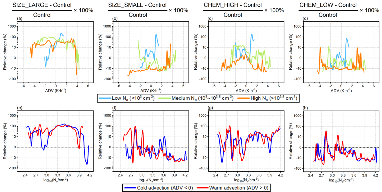
Figure 10. Same as Fig. 9, but for changes in CLWC.
