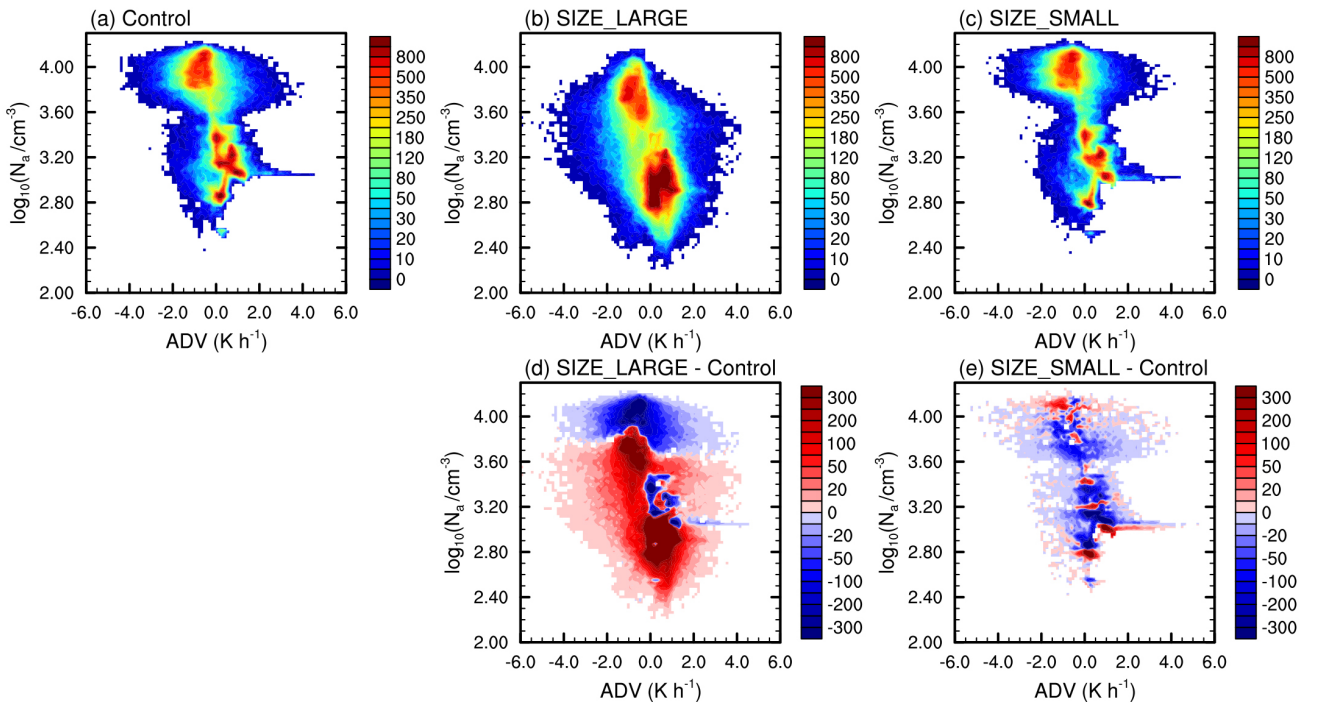
Figure 8. Variation of cloud lifetime (characterized by liquid-phase cloud sample count) with ADV and N_a . a, b, c, d, and e are the results of the Control, SIZE_LARGE, and SIZE_SMALL experiments, and the differences of SIZE_LARGE and SIZE_SMALL experiments relative to the Control experiment, respectively.
