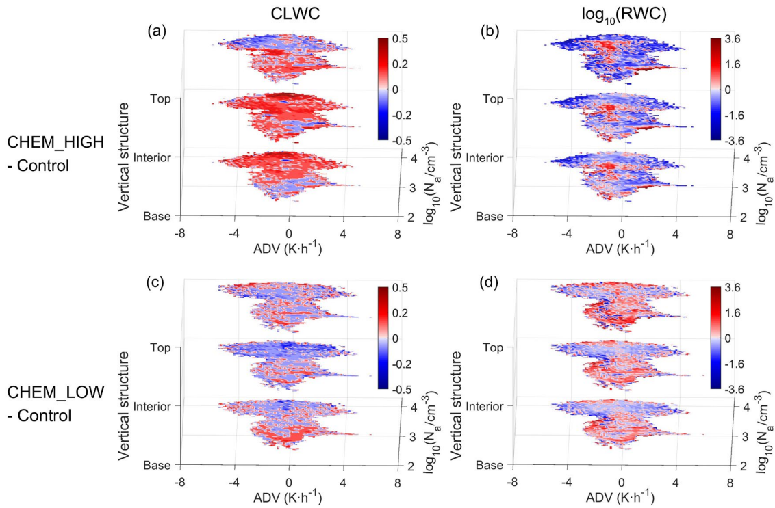
Figure 13. Differences of the CHEM_HIGH and CHEM_LOW experiments relative to the Control experiment in CLWC (unit: \text{g m}^{-3} ) and RWC (unit: \text{g m}^{-3} , presented logarithmically in base 10) as a function of N_a , ADV and cloud parts.
