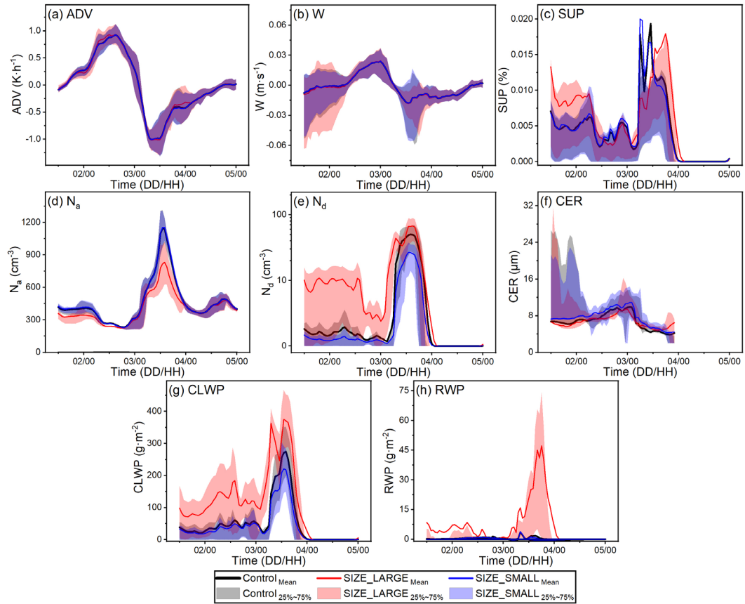
Figure 2. Temporal variations (lines, ECO regional mean) and the 25-75% interquartile range (shading, regional variability) of vertically weighted average temperature advection (a), vertical velocity (b) and supersaturation (c) from near the surface up to 1300 m (this height range is selected because over 97% of cloud droplets during the simulation period exist within this range, ensuring an accurate representation of the meteorological influence on ACI), column-mean N_a (d) and N_d (e), as well as CER (f), CLWP (g) and RWP (h) over ECO from the Control, SIZE_LARGE, and SIZE_SMALL experiments.
