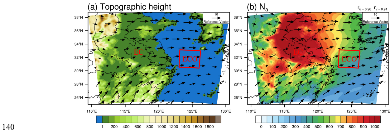
Figure 1. Topographic map of the outer domain (a, in m) and the distribution of column-mean N_a of the Control experiment (b, in \text{cm}^{-3} ) during the simulation period. The locations of EC and ECO are highlighted in red text, with the ECO extent (i.e., the inner domain) indicated by a red box. The time-averaged wind fields in (a) and (b) are derived from MICAPS data and the Control simulation, respectively. The values r_u and r_v in the upper-right corner of (b) denote the Pearson product-moment correlation coefficients for the U and V wind components between MICAPS and the simulation.
