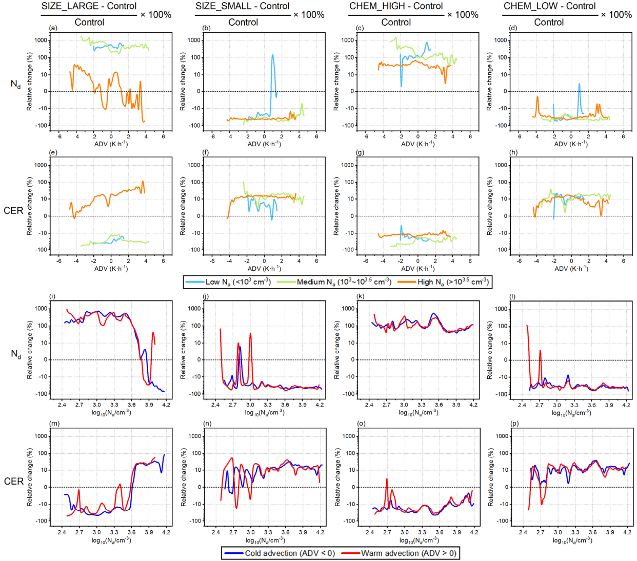
Figure 9. PercentageRelative changes in N_d and CER for the sensitivity experiments relative-compared to the Control experiment under different environmental conditions . Upper two rows: dependence on ADV (x axis) for different N_a conditions; lower two rows: dependence on N_a (x axis) for different ADV conditions.
