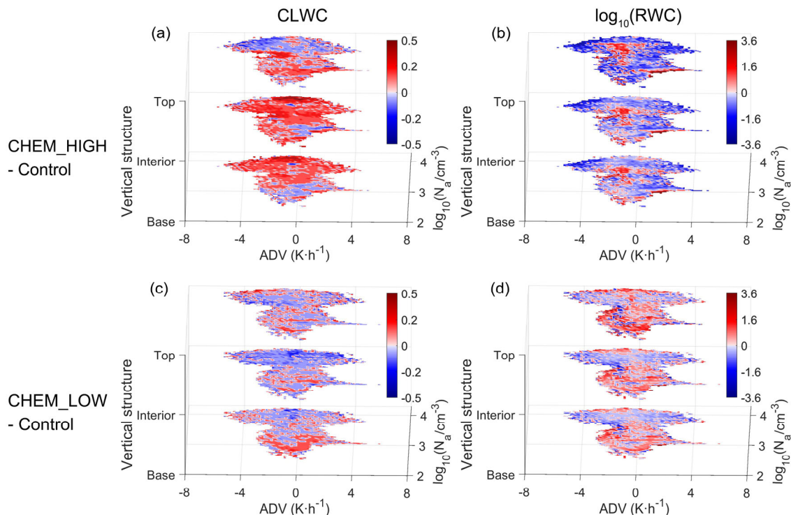
Figure 13. Differences of the CHEM_HIGH and CHEM_LOW experiments relative to the Control experiment between the CHEM_HIGH and CHEM_LOW experiments and the Control experiment in CLWC (unit: \text{g m}^{-3} ) and RWC (unit: \text{g m}^{-3} ), presented logarithmically in base 10) as a function of N_a , ADV and cloud parts.
