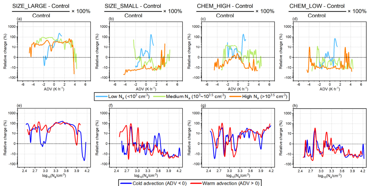
Figure 10. Same as Fig. 9, but for changes in CLWC. Relative changes in CLWC for the sensitivity experiments compared to the Control experiment under different environmental conditions.
