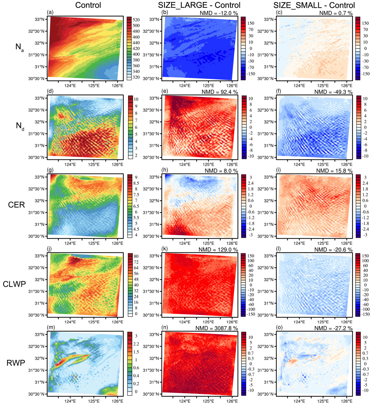
Figure 3. Spatial distributions of column -mean N_a (in \text{cm}^{-3} ), and , N_d (in \text{cm}^{-3} ), mean CER (in \mu\text{m} ), CLWP (in \text{g m}^{-2} ), and RWP (in \text{g m}^{-2} ) averaged over the simulation period from the Control experiment (left column), and differences of SIZE_LARGE (middle column) and SIZE_SMALL (right column) relative to the Control (NMD of each sensitivity experiment relative to the Control is indicated at the top-right of each subplot). Values represent liquid-phase clouds averaged over the simulation period, and grid points without clouds or with non-liquid-phase clouds are excluded. N_a and N_d are column averages, CLWP and RWP are column totals, and CER is calculated based on the droplet number in each bin.
