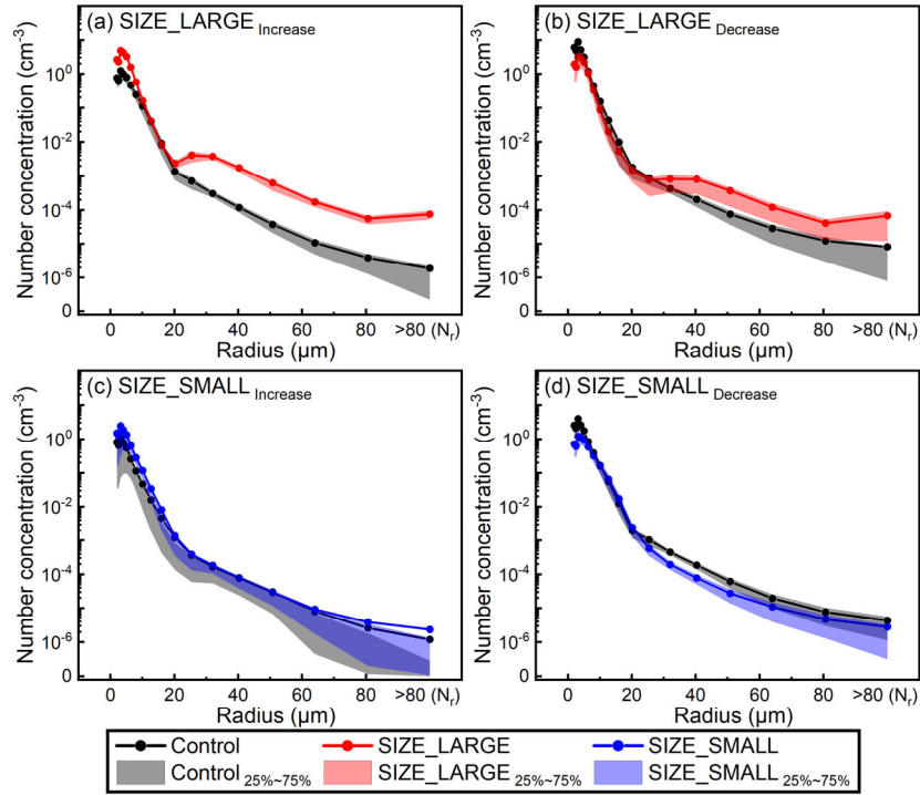
345 Figure 5. Mean changes Changes in droplet spectra ( lines, mean; shading, the 25-75% interquartile range ; droplets with a radius greater than 80 \mu\text{m} are raindrops and those less than 80 \mu\text{m} are cloud droplets) for the samples with an N_d -increase (left column) or decrease (right column) in N_d of more than exceeding 0.1\text{ cm}^{-3} , in response to increases (upper row) or decreases (lower row) in aerosol size.
