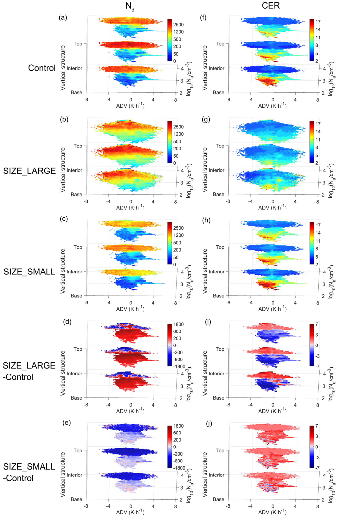
Figure 4. Variation of N_d (in \text{cm}^{-3} ) and CER (in \mu\text{m} ) of liquid-phase clouds with N_a , ADV and cloud parts in the three experiments, and the difference of between the SIZE_LARGE and SIZE_SMALL experiments relative to and the Control
