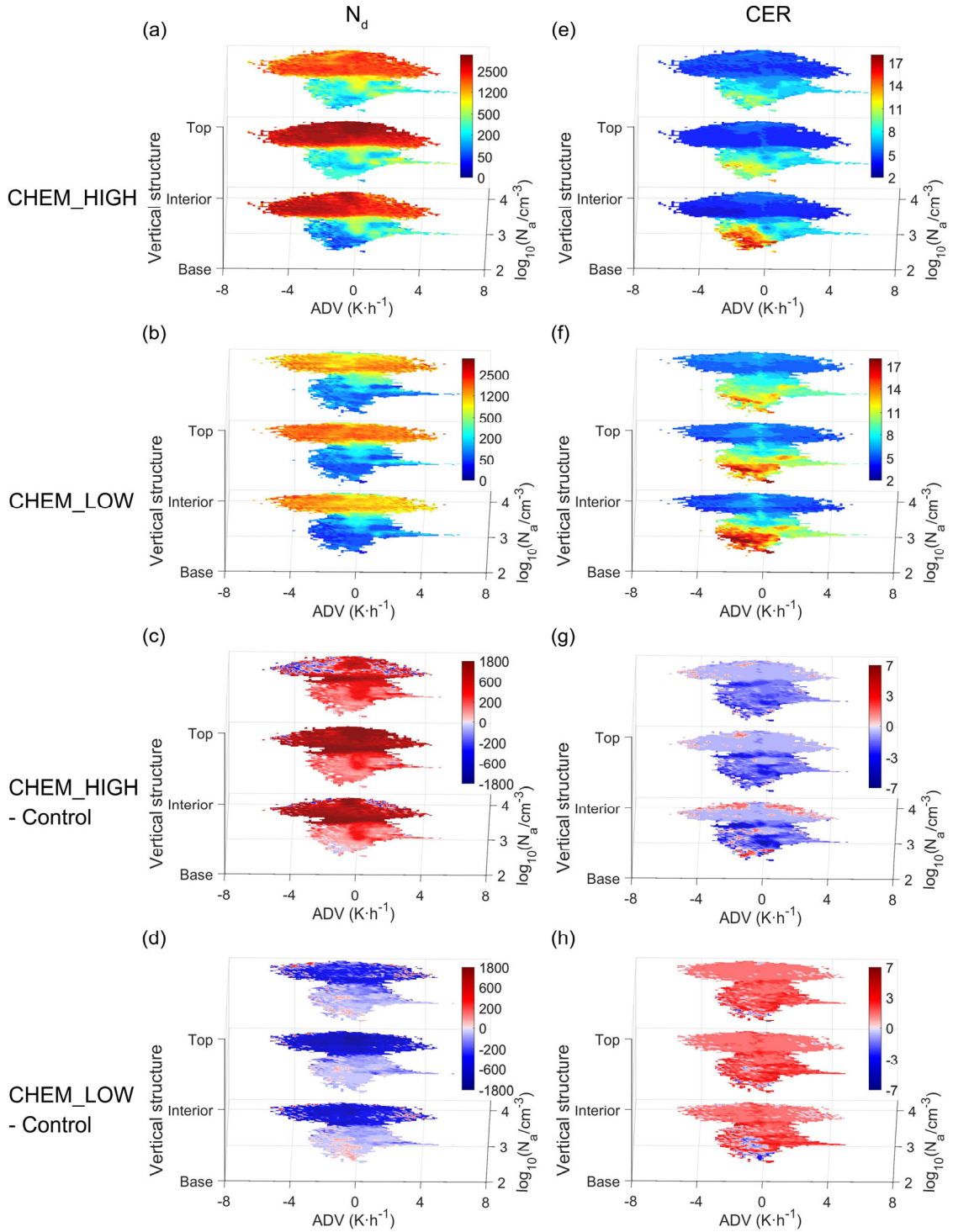
Figure 12. Variation of N_d (in \text{cm}^{-3} ) and CER (in \mu\text{m} ) with ADV, N_a and cloud parts for the CHEM_HIGH and CHEM_LOW experiments and their difference between the two experiments relative to the Control experiment.
