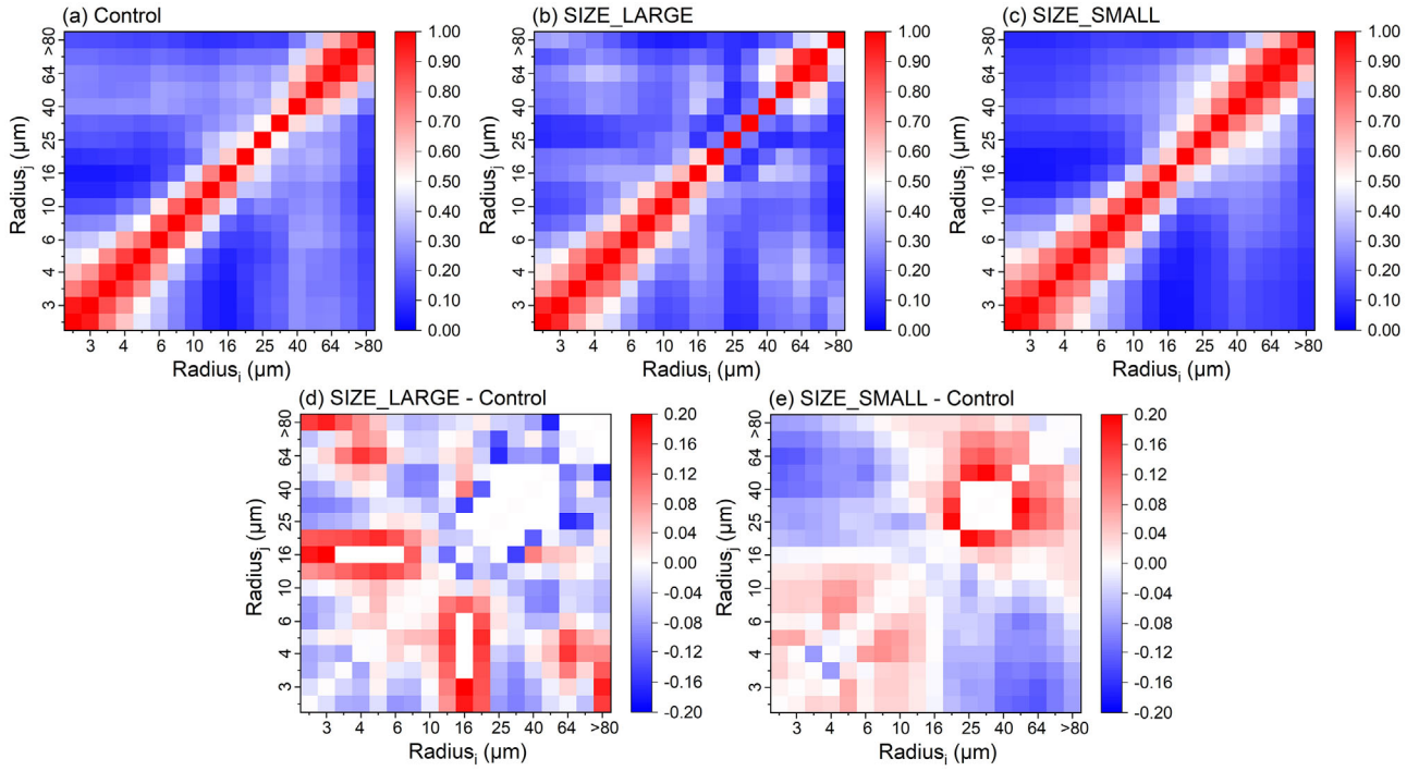
Figure 6. Correlation map distributions between liquid droplets number concentrations in size bins i and j of radius i and radius j from the Control (a), SIZE_LARGE (b), and SIZE_SMALL (c) experiments, and differences of SIZE_LARGE (d) and SIZE_SMALL (e) with the Control. For each size bin, the four-dimensional (time, height, latitude, longitude) droplet number concentration field is first flattened into a one-dimensional array in the same order, and the Pearson correlation coefficient between bins i and j is then computed. –(the correlation between two droplet size bins is calculated by first rearranging droplet number concentrations with dimensions of (time, height, latitude, longitude) for each size bin into one-dimensional arrays in the same order, and then computing the Pearson correlation coefficient between the two bins).
