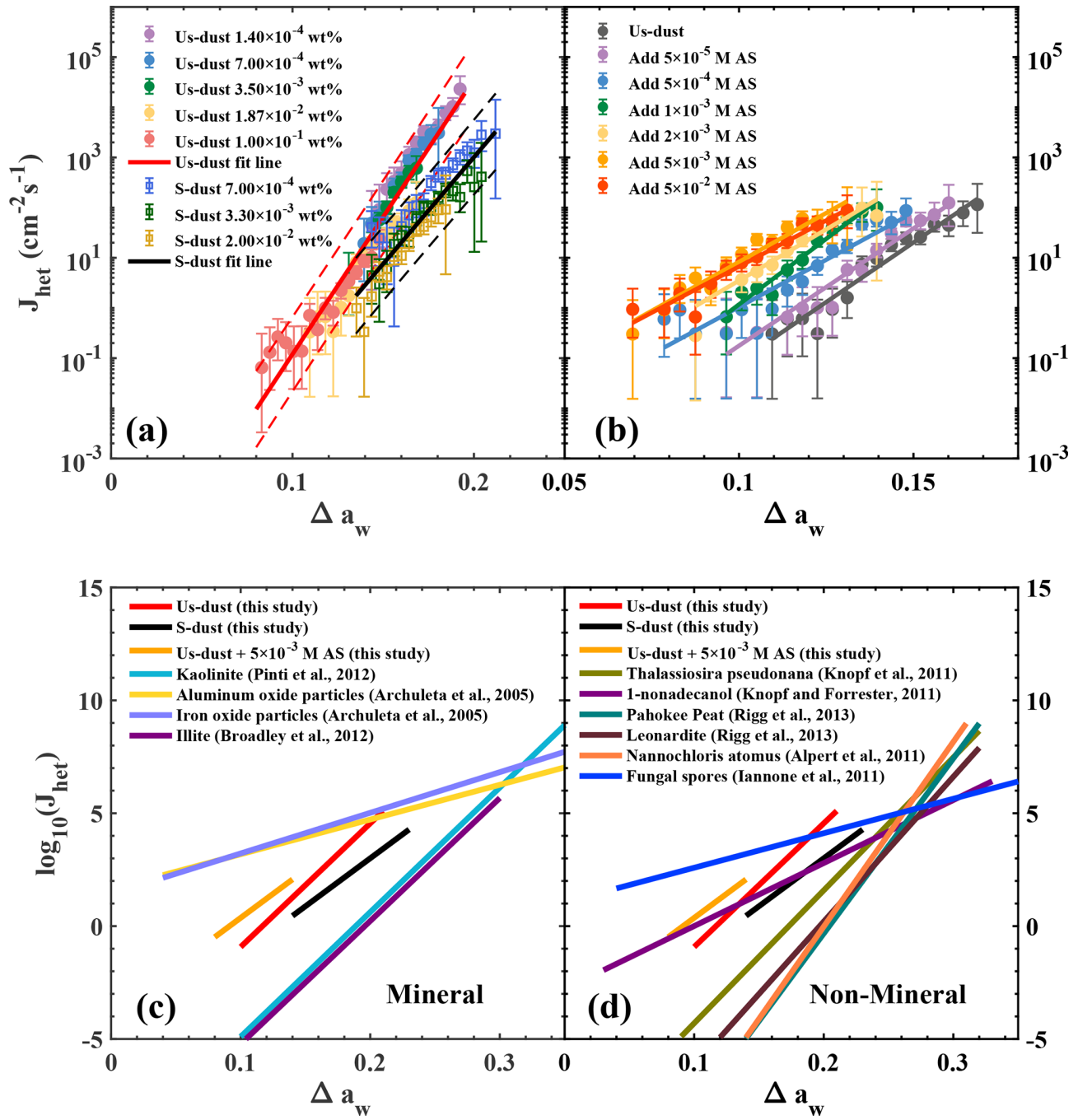
Figure 9. J_{\text{het}} as a function of \Delta a_w for Us-dust and S-dust (a), and Us-dust ( 1.87 \times 10^{-2} wt %) mixed with AS (b). Comparison J_{\text{het}} of Us-dust, S-dust, and Us-dust mixed with 0.005 M AS with minerals (c) and non-minerals (d) from previous studies (Alpert et al., 2011; Archuleta et al., 2005; Broadley et al., 2012; Iannone et al., 2011; Knopf et al., 2002, 2011; Knopf and Alpert, 2013; Knopf and Forrester, 2011; Murray et al., 2011; Pinti et al., 2012; Rigg et al., 2013). Dashed lines (a) are the 95 % prediction intervals. Solid lines (a, b) are parameterizations according to \log_{10}(J_{\text{het}}) = m_2 \times \Delta a_w + n_2 and the values of m_2 and n_2 are listed in Table S2.
