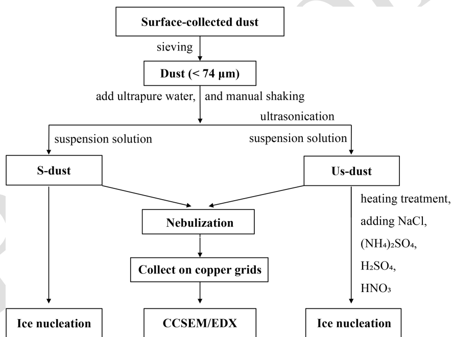
Figure 2. Schematic diagram of experimental procedures.
