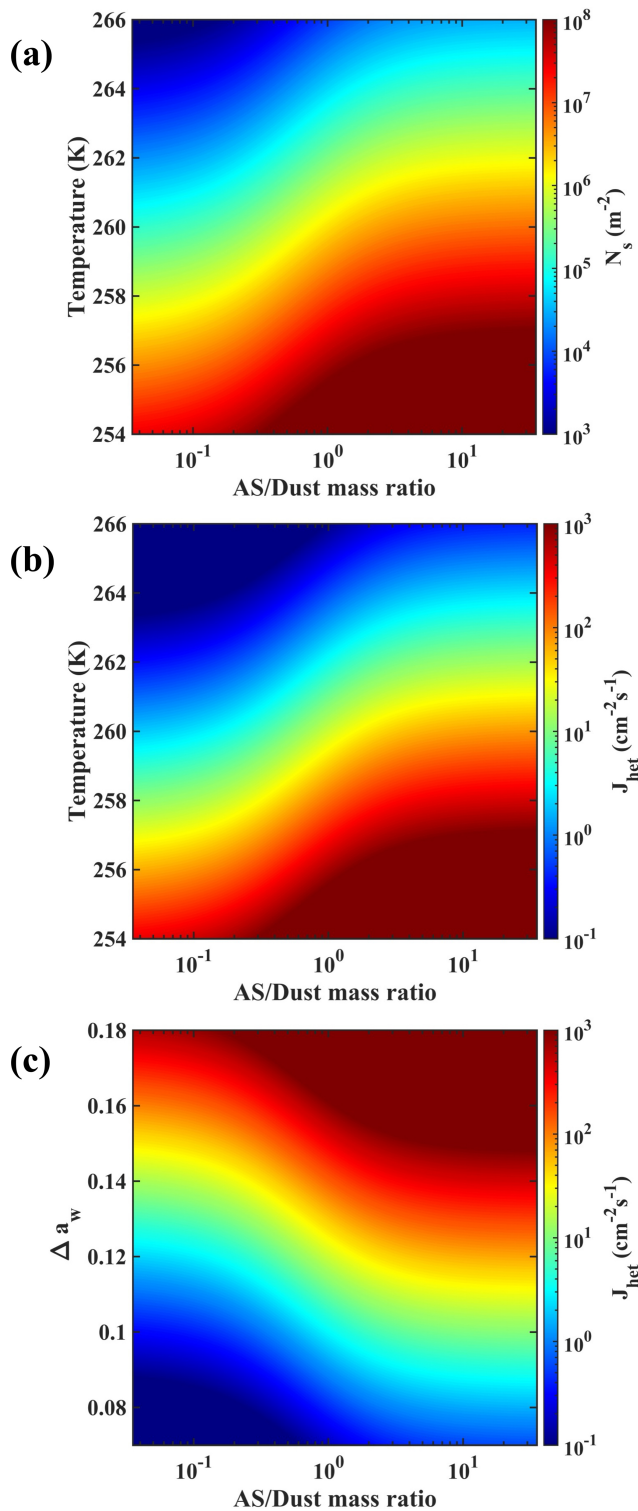
Figure 10. Prediction of N_s and J_{het} based on the parameterization of Us-dust mixed with AS. (a) N_s and (b) J_{het} as a function of temperature and AS/Dust mass ratio, (c) J_{het} as a function of \Delta a_w and AS/Dust mass ratio.
