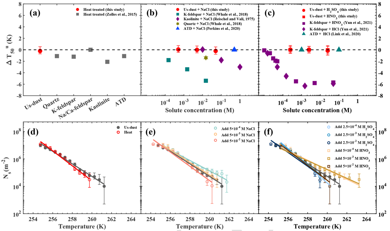
Figure 8. Comparison of \Delta T_{50}^u (a–c) and N_s (d–f) for Us-dust treated by heating, adding NaCl, H 2 SO 4 and HNO 3 . Error bars for +\Delta T_{50}^u represent the 25th and 75th percentiles. Error bars for N_s correspond to the 95 % confidence intervals. Solid lines are parameterizations of N_s . The comparison data in panels (a)–(c) are from previous studies (Link et al., 2020; Perkins et al., 2020; Reischel and Vali, 1975; Whale et al., 2018; Yun et al., 2021; Zolles et al., 2015).
