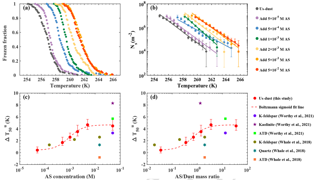
Figure 7. (a) Frozen fraction for Us-dust ( 1.87 \times 10^{-2} wt%) mixed with ammonium sulfate (AS) at different concentrations. (b) N_s with error bars corresponding to the 95 % confidence intervals. Solid lines are parameterizations of N_s . (c) \Delta T_{50}^u as a function of AS concentration. (d) \Delta T_{50}^u as a function of the mass ratio of AS to dust (AS/Dust). Dashed lines (c, d) represent the Boltzmann sigmoid fitting. Error bars (c, d) represent the 25 % and 75 % percentiles. The literature data in panels (c) and (d) are from Whale et al. (2018) and Worthy et al. (2021).
