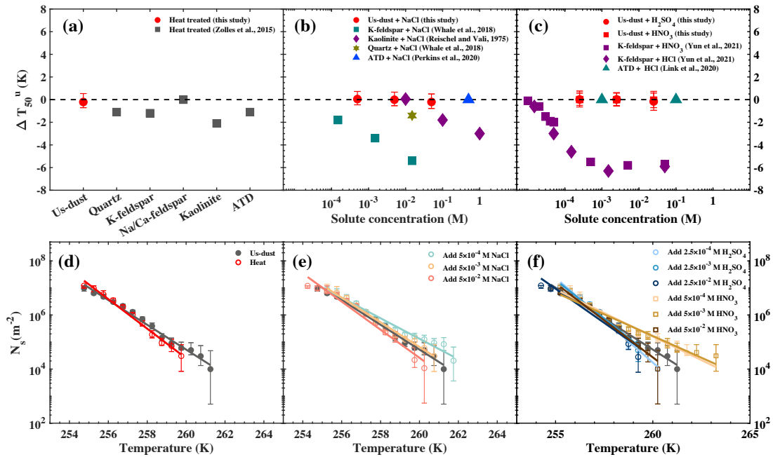
453 454 Figure 8. Comparison of \Delta T_{50}^u (a-c) and N_s (d-f) for Us-dust treated by heating, adding NaCl,
