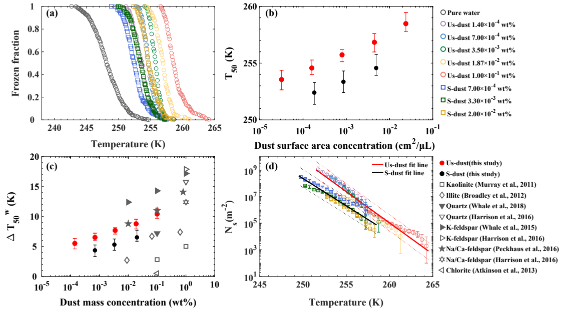
Figure 5. (a) Frozen fraction of water droplets, Us-dust and S-dust containing droplets. (b) T_{50} as a function of dust surface area concentration within a droplet. (c) \Delta T_{50}^w as a function of dust mass concentration. Error bars (b, c) in temperature correspond to the 25th and 75th percentiles of freezing temperature. Gray symbols (c) represent monomineralic dust from previous studies (Atkinson et al., 2013; Broadley et al., 2012; Harrison et al., 2016; Murray et al., 2011;
