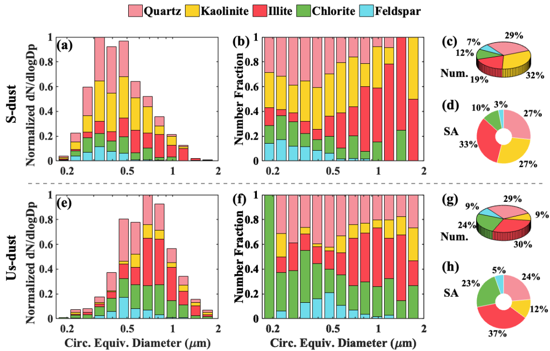
Figure 4. Particle size distribution and contribution of dust types for S-dust (upper panel, a-d) and Us-dust (lower panel, e-h). Normalized particle size distribution (a, e); relative number fraction of each particle type as a function of size (b, f); the number (c, g) and surface area (d, h) contribution of each particle type.
