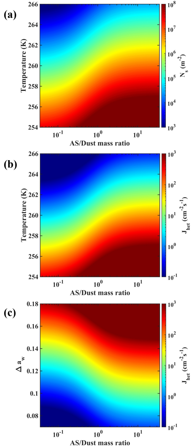
Figure 10. Prediction of N_s and J_{\text{het}} based on the parameterization of Us-dust mixed with AS. (a) N_s and (b) J_{\text{het}} as a function of temperature and AS/Dust mass ratio, (c) J_{\text{het}} as a function of \Delta a_w and AS/Dust mass ratio.
