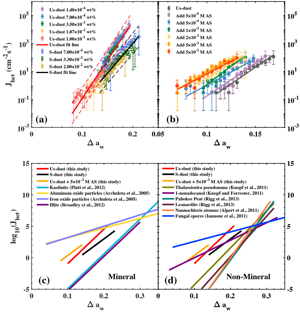
Figure 9. J_{het} as a function of \Delta a_w for Us-dust and S-dust (a), and Us-dust (1.87×10 -2 wt%) mixed with AS (b). Comparison J_{het} of Us-dust, S-dust, and Us-dust mixed with 0.005 M AS with minerals (c) and non-minerals (d) from previous studies (Alpert et al., 2011; Archuleta et al., 2005; Broadley et al., 2012; Iannone et al., 2011; Knopf et al., 2002, 2011; Knopf and Alpert, 2013; Knopf and Forrester, 2011; Murray et al., 2011; Pinti et al., 2012; Rigg et al., 2013). Dashed lines (a) are the 95% prediction intervals. Solid lines (a, b) are parameterizations according to \log(J_{het}) = m_2 \times \Delta a_w + n_2 and the values of m_2 and n_2 are listed in Table S2.
