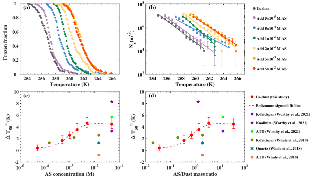
Figure 7. (a) Frozen fraction for Us-dust ( 1.87 \times 10^{-2} wt%) mixed with ammonium sulfate (AS) at different concentrations. (b) N_s with error bars corresponding to the 95% confidence intervals. Solid lines are parameterizations of N_s . (c) \Delta T_{50}^u as a function of AS concentration. (d) \Delta T_{50}^u as a function of the mass ratio of AS to dust (AS/Dust). Dashed lines (c, d) represent the Boltzmann sigmoid fitting. Error bars (c, d) represent the 25% and 75% percentiles. The literature data in panels (c) and (d) are from Whale et al. (2018) and Worthy et al. (2021).
