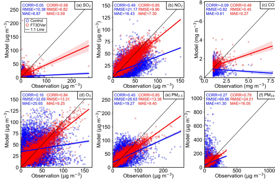
539 540 Figure 12. Scatter plots of observations against Control (blue) and FT3DVar analysis (red) 541 concentrations. The black line is the 1:1 line.
