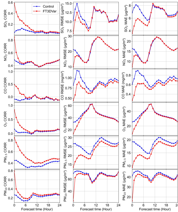
640 Figure 16. Temporal evolution of forecast performance for FT3DVar (red) and Control (blue) over the 641 24-hour period. From left to right: CORR, RMSE, MAE. From top to bottom: SO 2 , NO 2 , CO, O 3 , PM 2.5 , 642 PM 10 .
