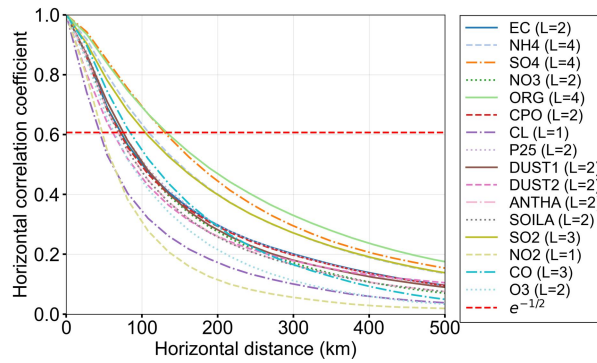
419 Figure 5. Decay of horizontal background error correlation coefficient with distance for each control 420 variable.
