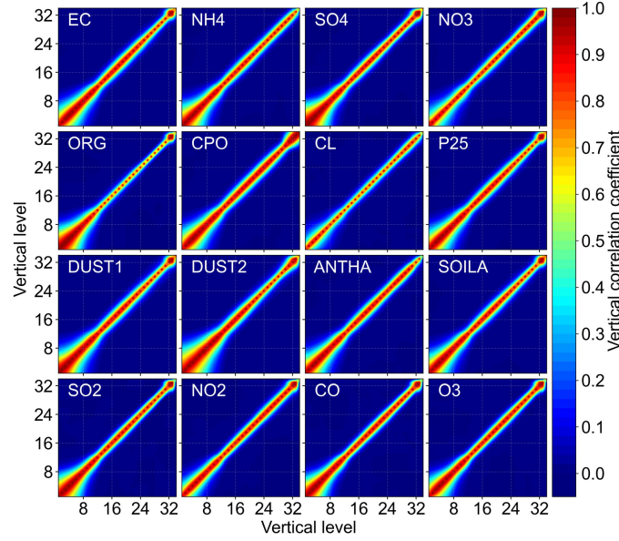
410 Figure 4. Distribution of the vertical autocorrelation matrix of background error for each control 411 variable.
