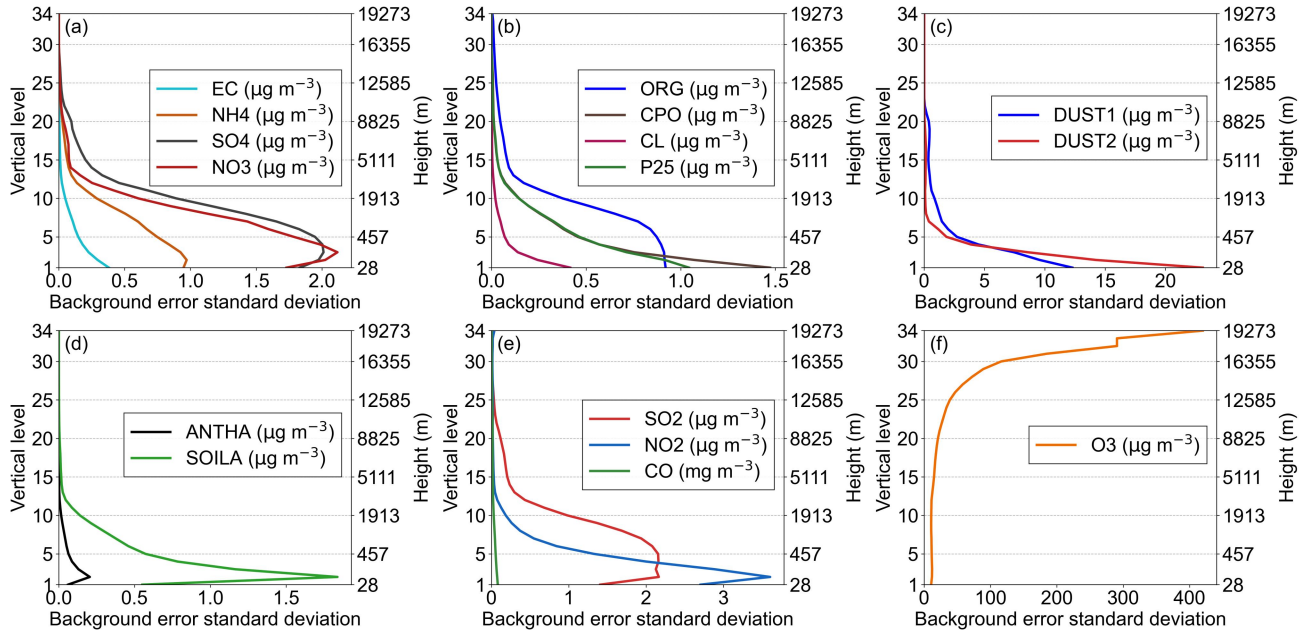
389 Figure 3. Vertical profiles of background error standard deviation for each control variable: (a) EC, 390 NH 4 , SO 4 , NO 3 ; (b) ORG, CPO, CL, P25; (c) DUST1, DUST2; (d) ANTHA, SOILA; (e) SO 2 , NO 2 , 391 CO; (f) O 3 .
