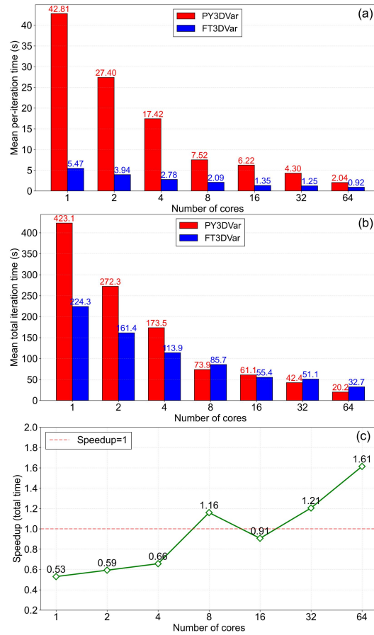
Figure 14. Parallel scalability of FT3DVar (blue) and PY3DVar (red) across CPU core counts. (a) Mean per-iteration time. (b) Mean total iteration time. (c) Speedup of PY3DVar relative to FT3DVar. Dashed line in (c): speedup = 1.
