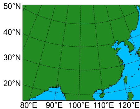
192 Figure 1. Distribution of the WRF-Chem simulation domain.
