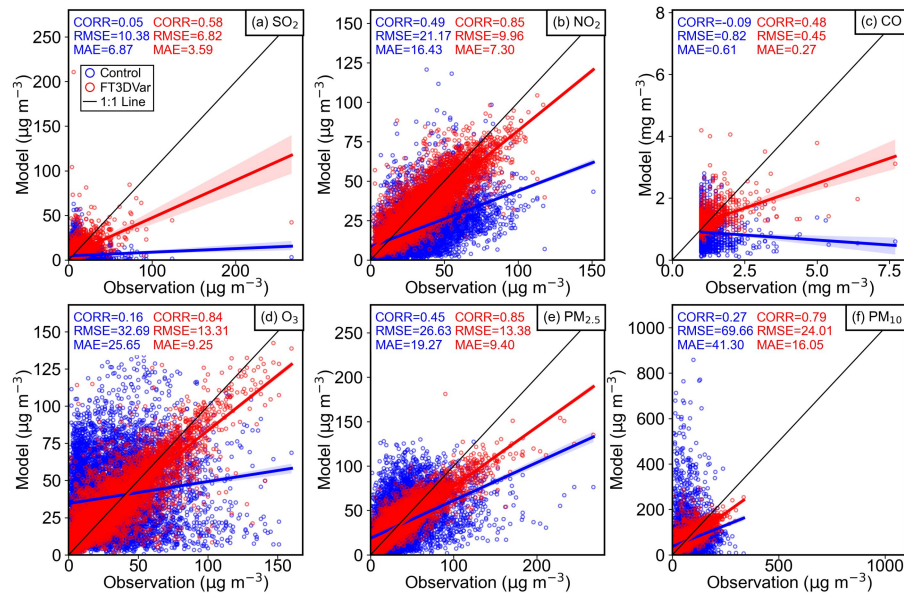
539 540 Figure 12. Scatter plots of observations against Control (blue) and FT3DVar analysis (red) 541 concentrations. The black line is the 1:1 line.
