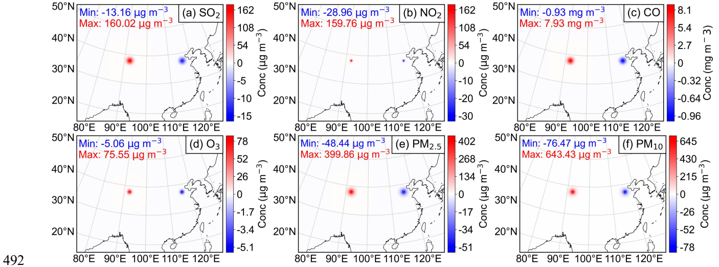
Figure 6. Surface increment fields for the six pollutants ((a) \text{SO}_2 , (b) \text{NO}_2 , (c) \text{CO} , (d) \text{O}_3 , (e) \text{PM}_{2.5} , (f) \text{PM}_{10} ) from the PY3DVar assimilation system in the idealized experiment. Blue and red colors represent negative and positive increments, respectively.
