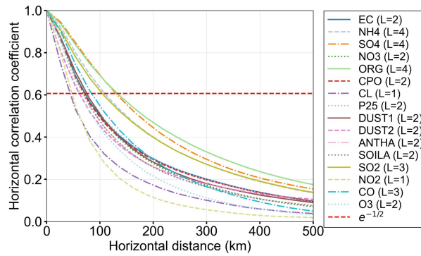
Figure 5. Decay of horizontal background error correlation coefficient with distance for each control variable.
