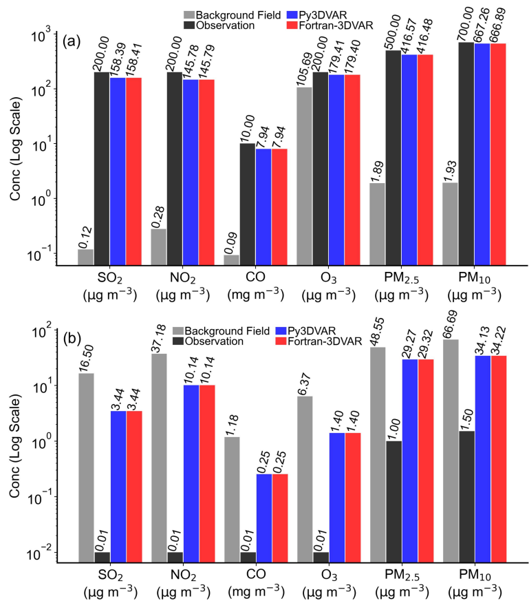
515 Figure 10. Comparison of background field (gray), observation (black), FT3DVar analysis field (red), and 516 PY3DVar analysis field (blue) under extremely high (a) and low (b) concentration conditions.
