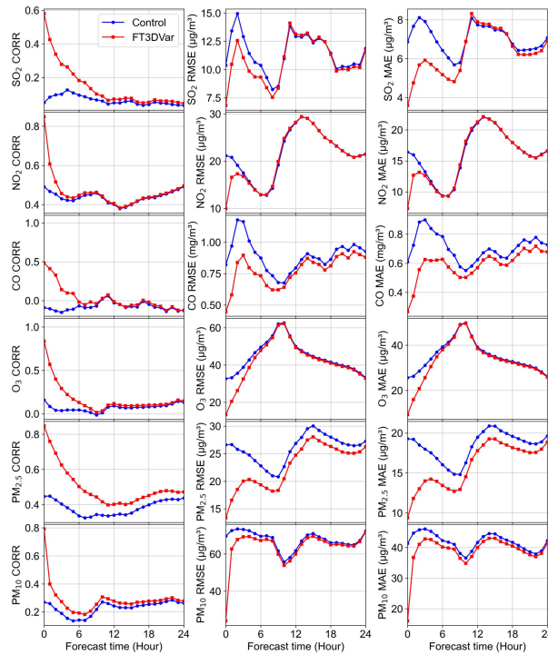
640 Figure 16. Temporal evolution of forecast performance for FT3DVar (red) and Control (blue) over the 641 24-hour period. From left to right: CORR, RMSE, MAE. From top to bottom: SO 2 , NO 2 , CO, O 3 , PM 2.5 , 642 PM 10 .
