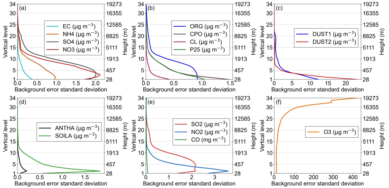
Figure 3. Vertical profiles of background error standard deviation for each control variable: (a) EC, NH 4 , SO 4 , NO 3 ; (b) ORG, CPO, CL, P25; (c) DUST1, DUST2; (d) ANTHA, SOILA; (e) SO 2 , NO 2 , CO; (f) O 3 .
