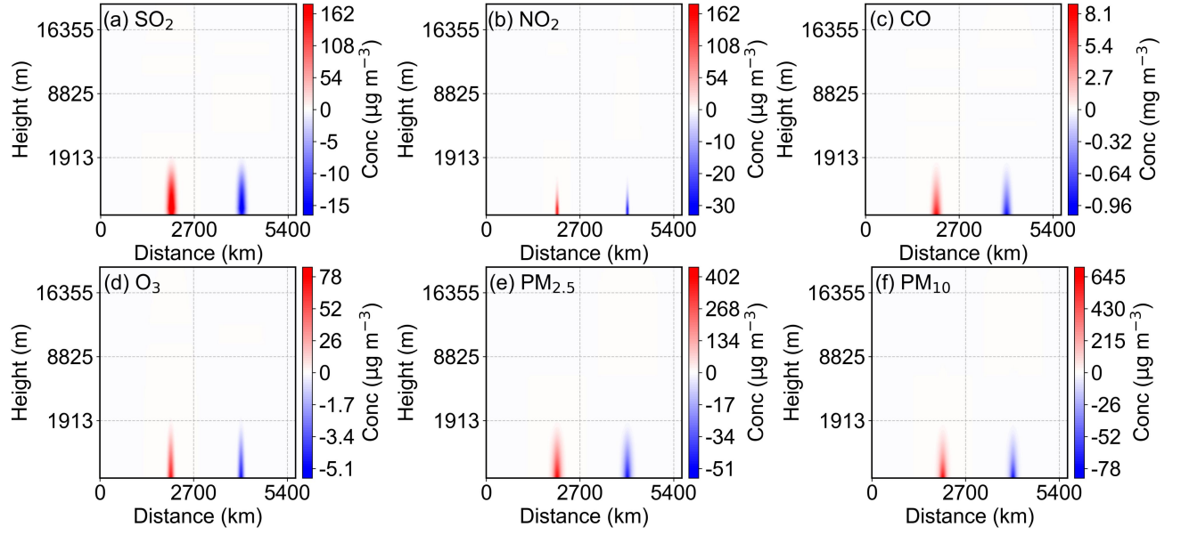
Figure 8. Vertical cross-sections of the increment fields for the six pollutants ((a) SO 2 , (b) NO 2 , (c) CO, (d) O 3 , (e) PM 2.5 , (f) PM 10 ) from the PY3DVar assimilation system in the idealized experiment. Blue and red colors represent negative and positive increments, respectively.
