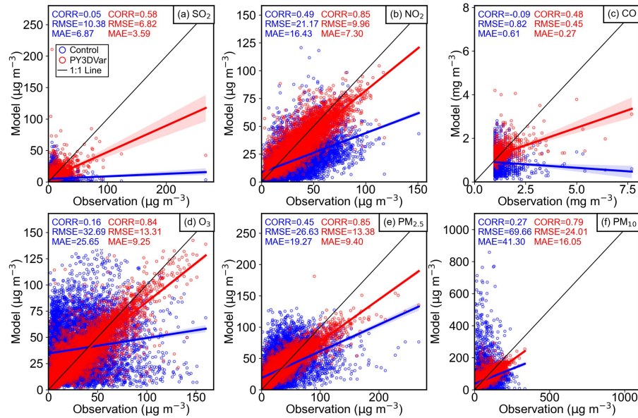
536 537 Figure 11. Scatter plots of observations against Control (blue) and PY3DVar analysis (red) 538 concentrations. The black line is the 1:1 line.
