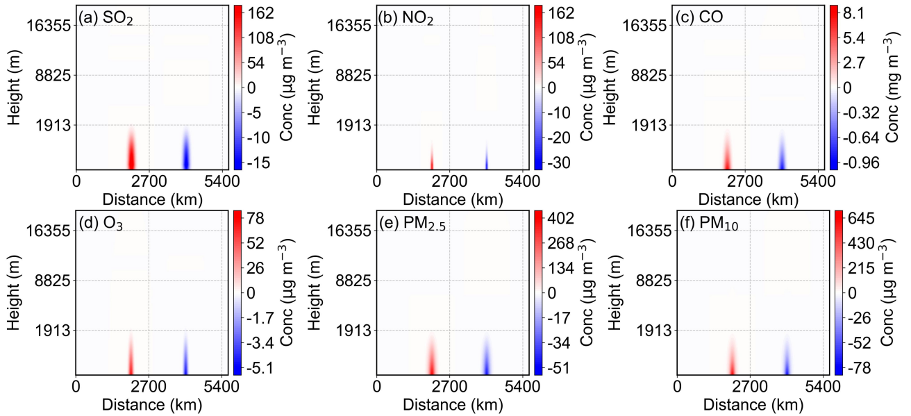
Figure 9. Vertical cross-sections of the increment fields for the six pollutants ((a) SO 2 , (b) NO 2 , (c) CO, (d) O 3 , (e) PM 2.5 , (f) PM 10 ) from the FT3DVar assimilation system in the idealized experiment. Blue and red colors represent negative and positive increments, respectively.
