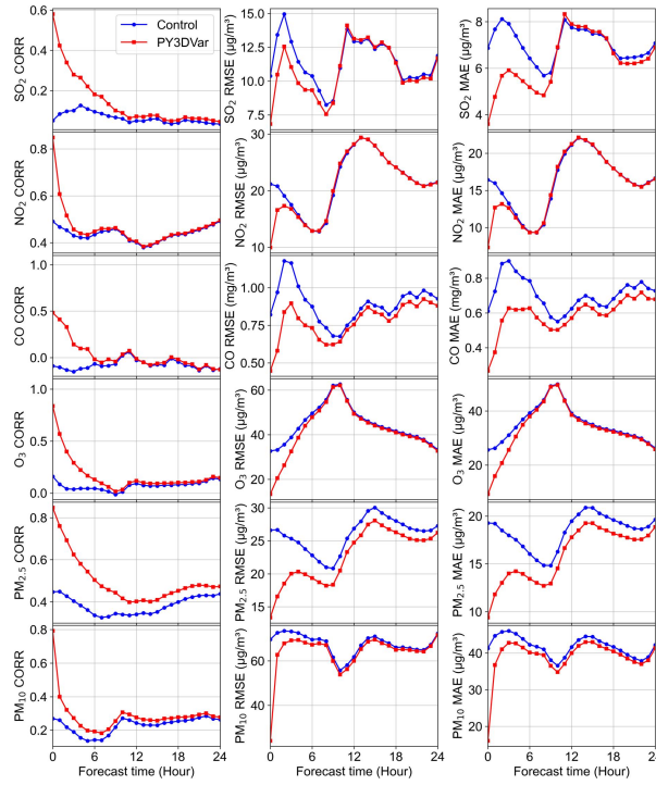
636 Figure 15. Temporal evolution of forecast performance for PY3DVar (red) and Control (blue) over the 637 24-hour period. From left to right: CORR, RMSE, MAE. From top to bottom: SO 2 , NO 2 , CO, O 3 , PM 2.5 , 638 PM 10 .
