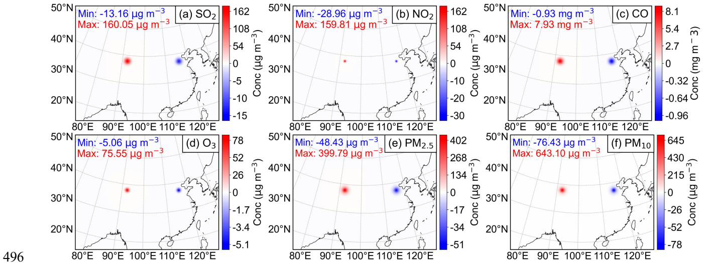
Figure 7. Surface increment fields for the six pollutants ((a) \text{SO}_2 , (b) \text{NO}_2 , (c) \text{CO} , (d) \text{O}_3 , (e) \text{PM}_{2.5} , (f) \text{PM}_{10} ) from the FT3DVar assimilation system in the idealized experiment. Blue and red colors represent negative and positive increments, respectively.
