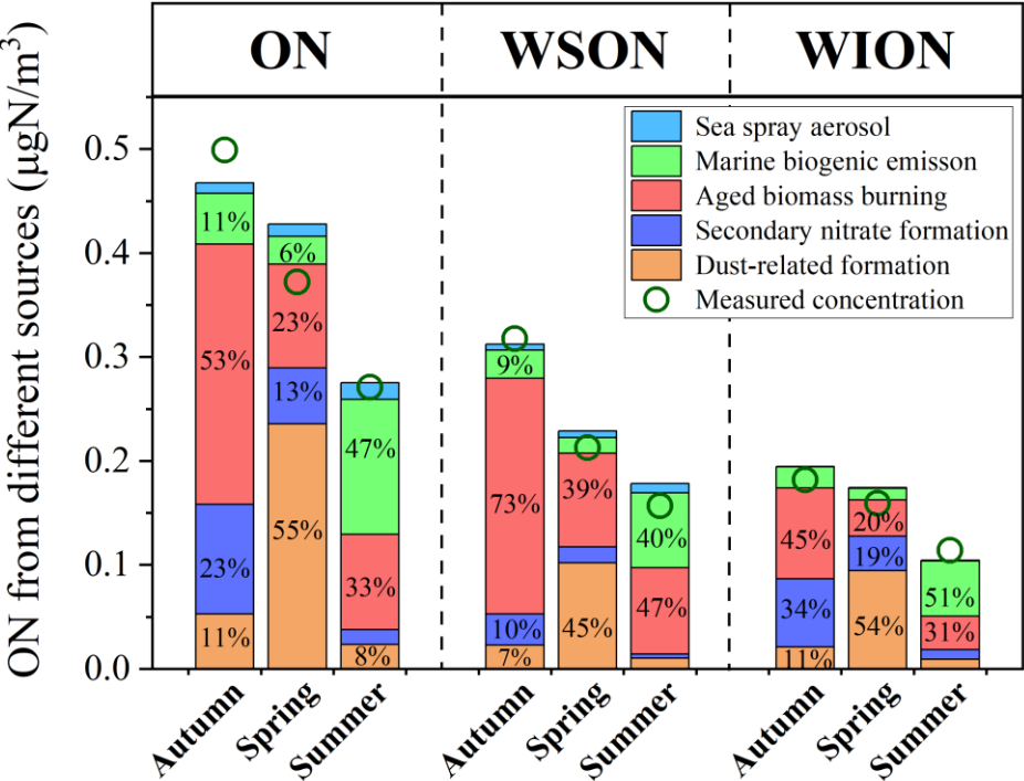
239 Figure 4. Aerosol ON, WSON, and WION from different sources resolved by PMF during cruise observations over the YBS. 240 The relative contribution of each source to the total ON, WSON, or WION is listed in the corresponding stacked column. 241
