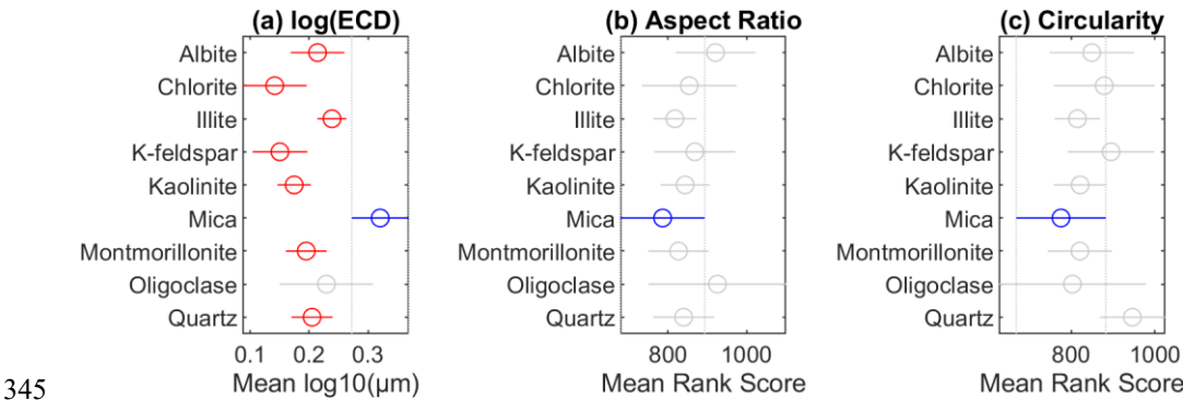
Figure 6. Multiple comparison plots for the ANOVA and Kruskal-Wallis results. Mica is highlighted in blue in all plots. Minerals highlighted in red have statistically different means than mica at the 95% level. Gray data points indicate no statistical difference in the means. (a) Results of the ANOVA for log(ECD). (b) Results of the Kruskal-Wallis analysis for aspect ratio. (c) Results of the Kruskal-Wallis analysis for circularity.
