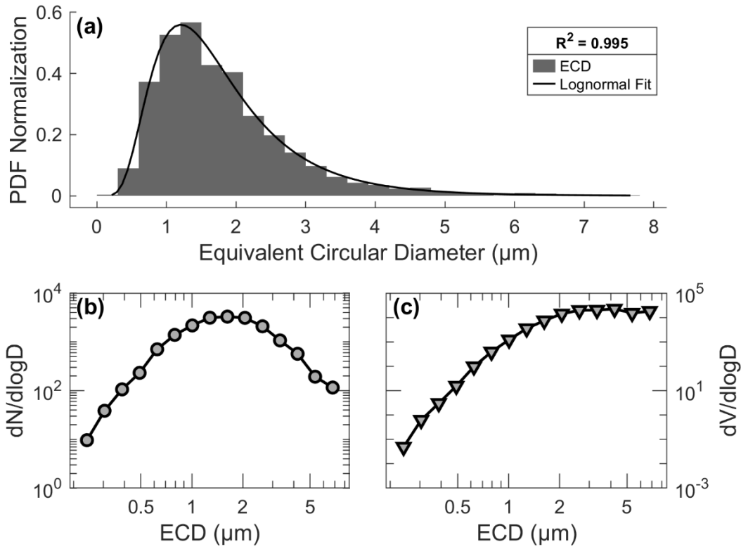
265 Figure 3. Particle size distributions and concentrations. (a) Histogram of the equivalent circular diameter (ECD) data with lognormal fit. (b) Particle concentrations as a function of ECD, normalized as dN/d\log D . (c) Volume concentrations as a function of ECD, normalized as dV/d\log D .
