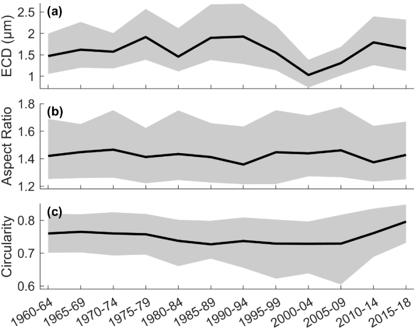
Figure 7. Time series of particle size and shape characteristics. Thick black lines represent median values; grey shaded 375 areas show the 25%–75% quartile range. (a) Equivalent circular diameter. (b) Aspect ratio. (c) Circularity.
