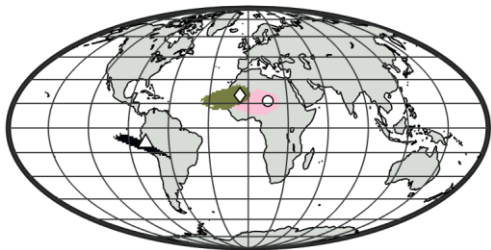
Figure 11. HYSPLIT 10 d ensemble trajectory frequency models. (a) Early wet season months December–February 2000–2015. (b) Late wet season months March–May 2000–2015. (c) Dry season months June–September 2000–2015. The El Djouf (diamond, green) and Bodélé (circle, pink) trajectories represent forward simulations pinpointing where at least 2.5%
