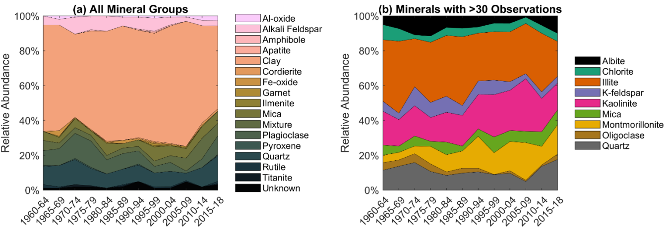
Figure 8. Stacked area time series plots showing relative mineral abundance. (a) All identified mineral groups. (b) Individual mineral species with at least 30 observations during the study period.
