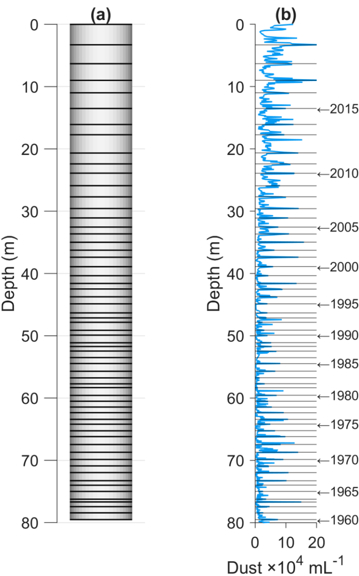
150 Figure 2. Dust sampling scheme for the 2019 Huascarán Col A ice core (HC-19A). (a) Schematic of the ice core with black lines showing the sampling depths. Made with the Core Stratigraphy Visualization tool in MATLAB® ( https://www.mathworks.com/matlabcentral/fileexchange/173320-core-stratigraphy-visualization ). (b) Microparticle concentrations as a function of depth, determined by Coulter Counter. Black horizontal lines denote the sampling depths for this study with annual labels every fifth year.
