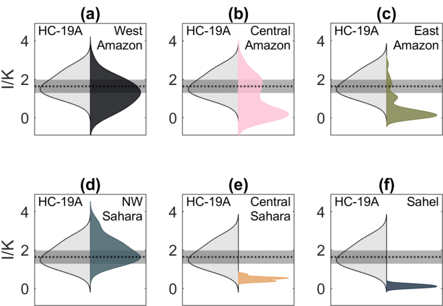
630 Figure 10. Violin plots comparing illite/kaolinite (I/K) ratios in HC-19A to potential source areas. In all figures, the black dotted line represents the calculated I/K ratio across all samples, and the surrounding shaded area is the 3σ (~99%) confidence interval based on Poisson uncertainty. The shapes of the violin plots illustrate kernel density estimates based on the I/K ratios of each sample. The I/K ratios of HC-19A are shown on the lefthand side of each violin plot. The I/K ratios of the PSAs are shown on the righthand side of each violin plot. (a-c) Soil mineral data are from Guyot et al. (2007). The Amazon is divided into three sub-regions: West (west of 65°W); Central (between 70°W and 60°W); and East (east of 65°W). In addition, all Amazonian sub-regions correspond to latitudes north of 12°S. (d-f) Soil mineral data are from Caquineau et al. (1998, 2002).
