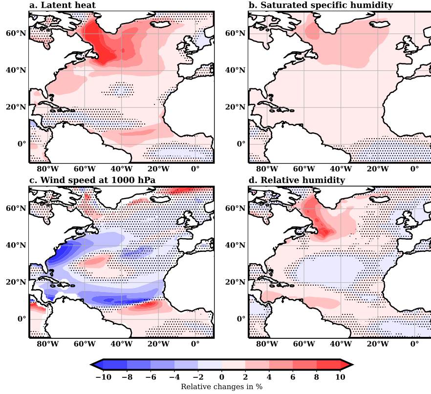
Figure 5. Multimodel averaged relative mean of fractional changes in AMV^+ minus AMV^- in JAS for: a) latent heat; b) saturation specific humidity at surface; c) wind speed at 1000 hPa; and d) near-surface relative humidity (plotted as -\delta RH/(1 - \overline{RH}) ). Relative humidity is calculated using near-surface specific humidity and the saturated specific humidity at the surface. The latter is estimated over the ocean by first calculating the saturated saturation vapour pressure based on surface temperature (WMO, 2024) and then transforming it into saturation specific humidity, taking into account sea level pressure. Note that ECMWF-IFS-HR and ECMWF-IFS-LR models were not used for surface calculations since they did not provide near-surface specific humidity. Likewise, EC-Earth3 was not used for wind speed at 1000 hPa. Changes Fractional changes are expressed relative to the climatological values at each grid point, which are calculated as half the sum of AMV^+ and AMV^- simulations. Dots mark regions where fewer than 80% of the models agree on the sign of changes, and values over land are masked out.
