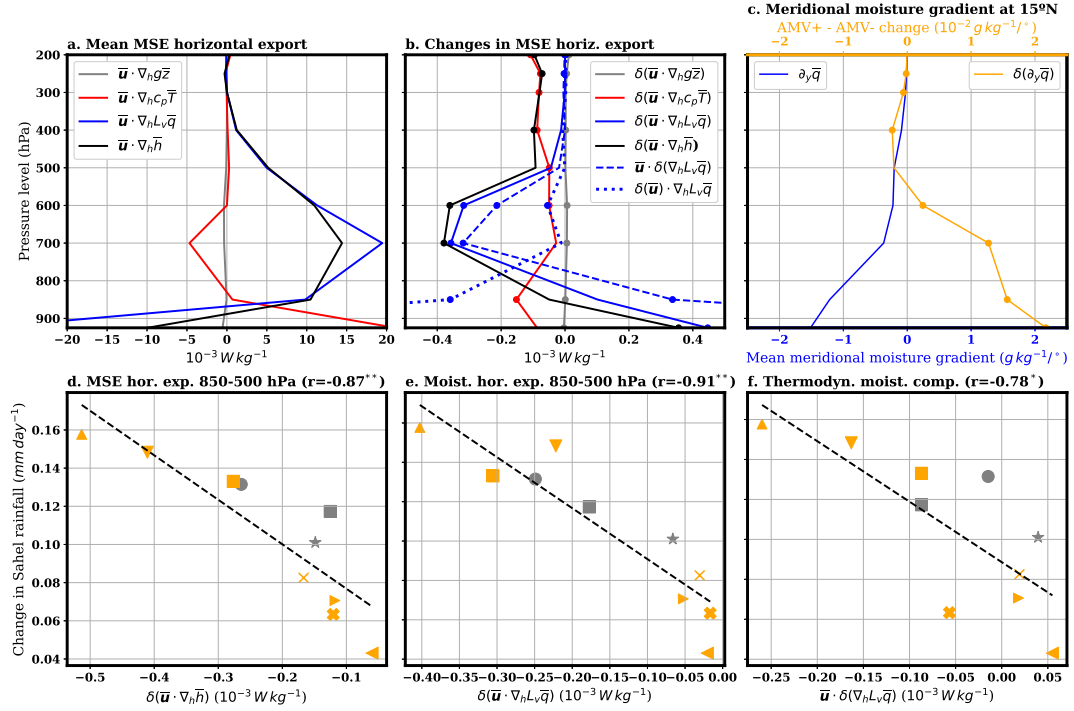
Figure 7. a) Climatological export of MSE by the time-mean horizontal flow ( \bar{\mathbf{u}} \cdot \nabla_h \bar{g} \bar{z} , black line) partitioned into the potential energy ( \bar{\mathbf{u}} \cdot \nabla_h \bar{g} \bar{z} , grey line), sensible ( \bar{\mathbf{u}} \cdot \nabla_h c_p \bar{T} , red line), and latent enthalpy ( \bar{\mathbf{u}} \cdot \nabla_h L_v \bar{q} , blue line) components averaged over the Sahel box (10°W-10°E, 10°N-20°N) for the multimodel mean. b) AMV + minus AMV - multimodel change in the export of MSE by the time-mean horizontal flow ( \delta(\bar{\mathbf{u}} \cdot \nabla_h \bar{h}) , black) partitioned into the potential energy ( \delta(\bar{\mathbf{u}} \cdot \nabla_h \bar{g} \bar{z}) , grey), sensible ( \delta(\bar{\mathbf{u}} \cdot \nabla_h c_p \bar{T}) , red), and latent enthalpy ( \delta(\bar{\mathbf{u}} \cdot \nabla_h L_v \bar{q}) , blue) averaged over the Sahel box. The change in latent enthalpy has been further decomposed into its thermodynamic ( \bar{\mathbf{u}} \cdot \delta(\nabla_h L_v \bar{q}) , blue dashed) and dynamic ( \delta(\bar{\mathbf{u}}) \cdot \nabla_h L_v \bar{q} , blue dotted) components. c) Multimodel mean meridional gradient of the 10°W-10°E zonally averaged specific humidity ( \text{g kg}^{-1} \text{ per } ^\circ ) at 15°N ( \partial_y \bar{q} , blue) and AMV + minus AMV - changes ( \delta(\partial_y \bar{q}) , orange). Scatter plots of averaged Sahel rainfall change ( \text{mm day}^{-1} ) and averages of changes over the Sahel box between 850 hPa and the 500 hPa levels of: d) total export of MSE due to time-mean horizontal flow ( \delta(\bar{\mathbf{u}} \cdot \nabla_h \bar{h}) ); e) MSE export due to horizontal moisture advection in MSE units ( \delta(\bar{\mathbf{u}} \cdot \nabla_h L_v \bar{q}) ); and f) its thermodynamic component also in MSE units ( \bar{\mathbf{u}} \cdot \delta(\nabla_h L_v \bar{q}) ). Units for the energetic terms are 10^{-3} \text{ W kg}^{-1} . For the models following the PRIMAVERA protocol (marked with orange symbols), only half of the anomalies are shown. The legend for the symbols in the scatter plots is the same as in Fig. 2c. Dots in plots b and c mark changes for which at least 80 % of the models agree on the sign. In the scatter plots, the dashed line shows the linear regression fit, and the correlation coefficient is shown in the title. Correlations are marked with one asterisk if they are statistically significant at the level of \alpha=0.05 when taking all the models as independent samples. Two asterisks are used if correlations are statistically significant when lowering the number of independent samples to 6.
