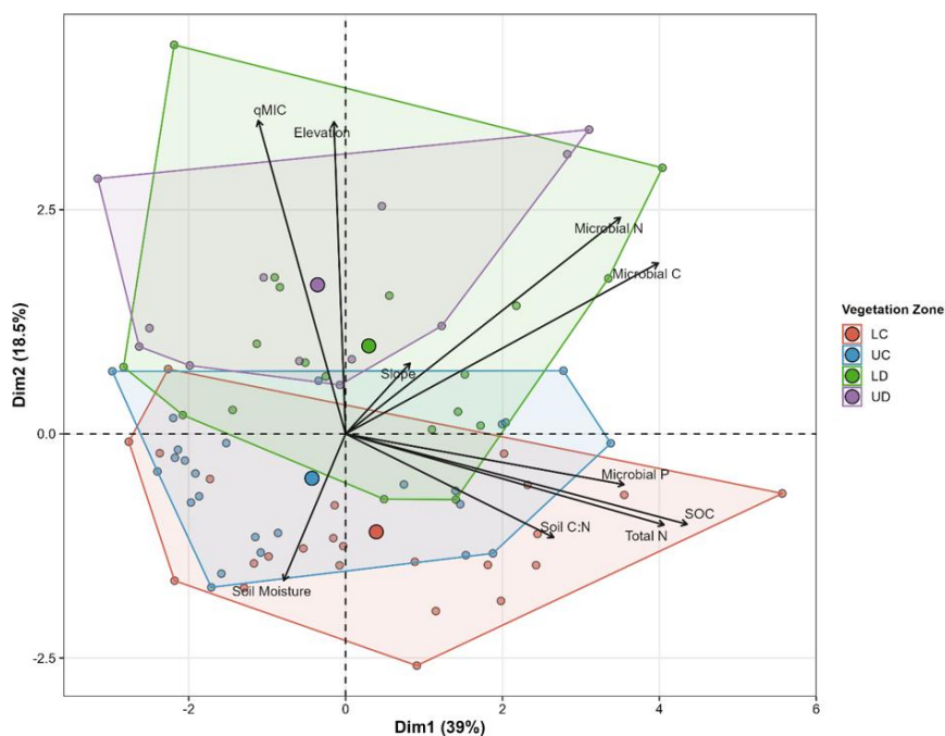
Figure 6. Principal component analysis (PCA) of microbial biomass fractions, microbial stoichiometric indices, bulk soil nutrient concentrations, and environmental variables across four altitudinal–vegetational zones of the Rolwaling treeline ecotone. Polygons represent the distribution of samples within each vegetation zone. Vector length and direction indicate the relative contribution of individual variables to the ordination space.
