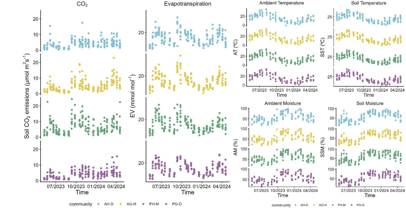
Figure 2. Scatter plots showing climate variables values over time for the four plant communities.
