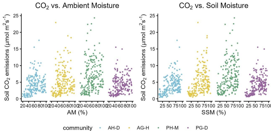
230 Figure 6. Relationship between soil CO 2 emissions and climate (left) and soil (right) moisture of the four plant communities.
