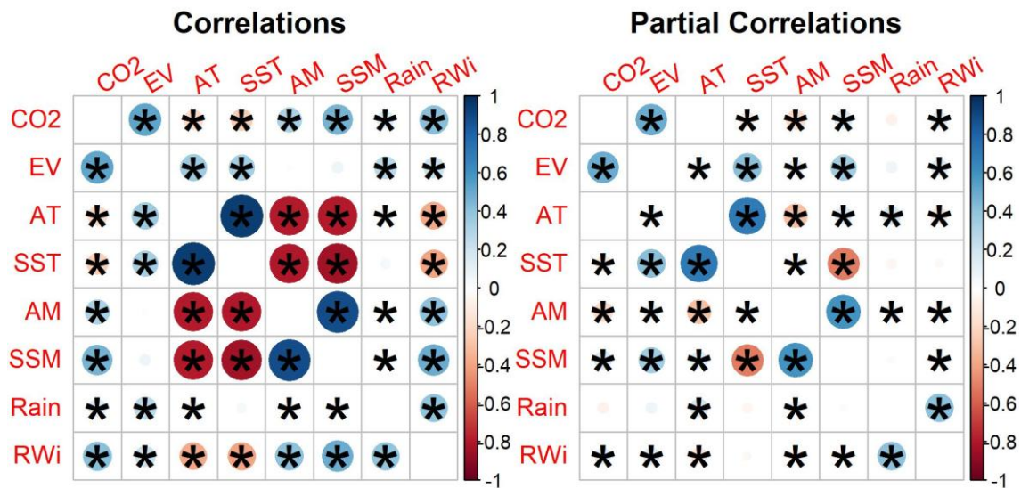
Figure 4. Correlation (left) and partial correlation (right) coefficients between variables within the whole sample. Correlation values are shown as size and colour of the circles. Only significant correlations are shown.
