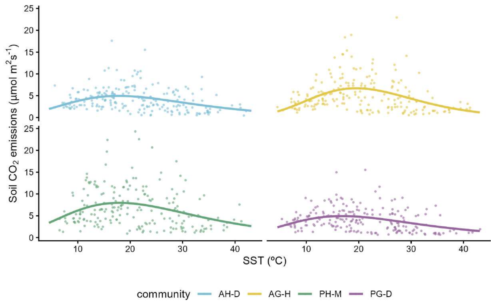
CO 2 vs. SST
