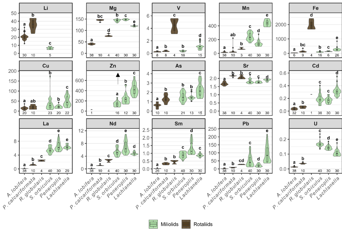
Figure 4: Distribution of El/Ca between different taxa. Values are expressed as \mu\text{mol/mol} except for Mg/Ca and Sr/Ca that are \text{mmol/mol} . The colors separate the species into two orders; rotaliids (brown) and miliolid (green) foraminifera. Letters above each distribution indicate statistically significant differences between species in each order. Numbers at the x-axes represents the number of replicate analyses. The arrow marks an outlier Zn/Ca value ( 4063 \mu\text{mol/mol} ) that was excluded from the plot.
