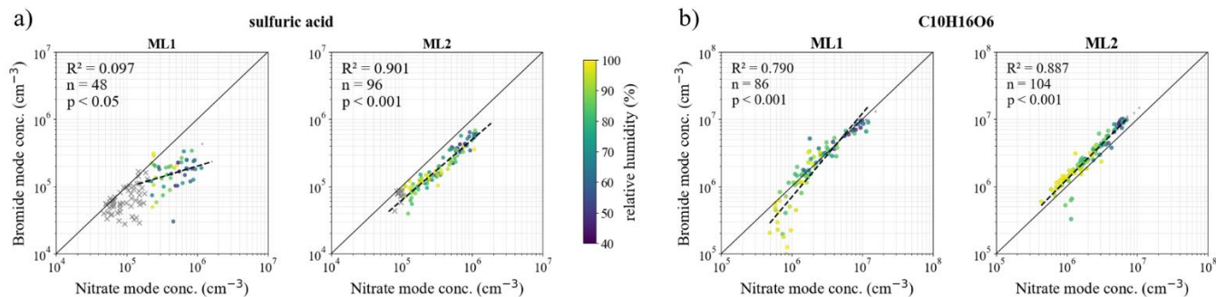
Figure 7 Scatter plots of hourly median concentrations measured in bromide mode versus nitrate mode for (a) sulfuric acid and (b) C_{10}H_{16}O_6 obtained with ML1 and ML2 during 27-30 July 2024. Dashed lines indicate linear regressions for each plot, with the corresponding coefficient of determination ( R^2 ), number of data points considered (n), and probability value (p) reported. The color of the points represents the relative humidity, as indicated by the color bar in the center. Points falling below the corresponding LOD_{CIMS} are shown as crosses (X), while outliers are plotted as smaller semi-transparent points; both are excluded from the linear fits.
