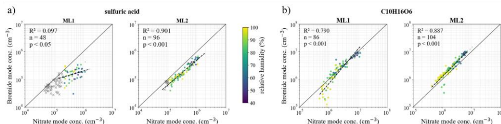
Figure 7 Scatter plots of hourly median concentrations measured in bromide mode versus nitrate mode for (a) sulfuric acid and (b) \text{C}_{10}\text{H}_{16}\text{O}_6 obtained with ML1 and ML2 during 27–30 July 2024. Dashed lines indicate linear regressions for each plot, with the corresponding coefficient of determination ( R^2 ), number of data points considered ( n ), and probability value ( p ) reported. The color of the points represents the relative humidity, as indicated by the color bar in the center. Points falling below the corresponding \text{LOD}_{\text{CIMS}} are shown as crosses (X), while outliers are plotted as smaller semi-transparent points; both are excluded from the linear fits.
