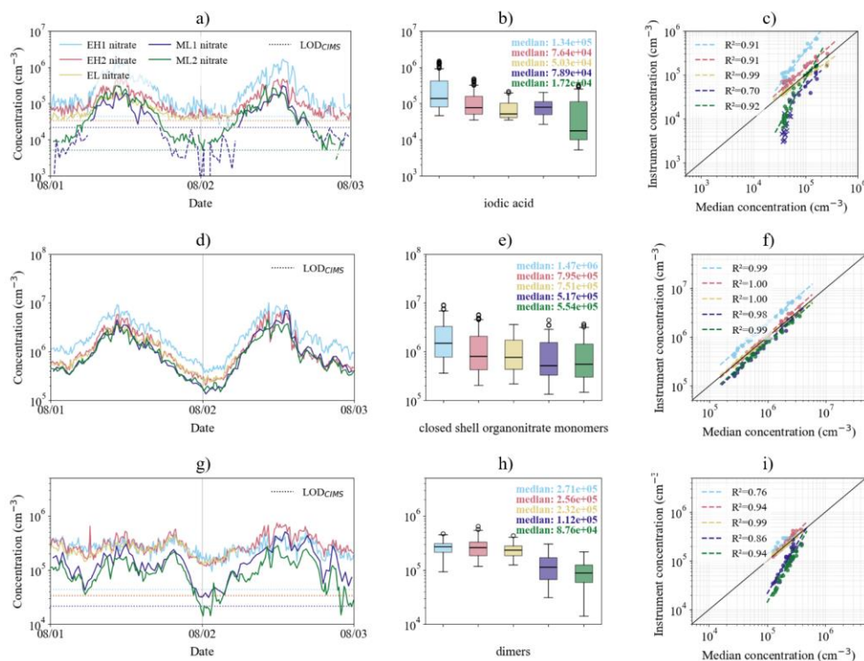
Figure 5 Concentrations of (top panel) iodic acid, (central panel) closed shell organonitrate monomers, and (bottom panel) dimers measured in nitrate mode by five mass spectrometers (CI-API-ToFs) during 1-2 August 2024. For each panel, the left plot-figure ((a), (d), and (g)) shows concentration time series, with instrument-specific LOD_{CIMS} values indicated by dotted horizontal lines. The central figure ((b), (e), and (h)) plot shows a box plot summarizing the distributions over the same period; boxes indicate the interquartile range, horizontal lines indicate the median, whiskers represent the non-outlier range, and empty circles denote outliers. Data points below LOD_{CIMS} are excluded from the box plot. The right figure ((c), (f), and (i)) plot shows the hourly median concentrations measured by each instrument against the median of the hourly median concentrations across all five instruments. Dashed lines indicate log-log linear regressions for each instrument, with the corresponding coefficient of determination ( R^2 ) reported in the legend. Points below the corresponding LOD_{CIMS} are shown as crosses (X), while outliers are plotted as smaller semi-transparent points; both are excluded from the linear fits.
