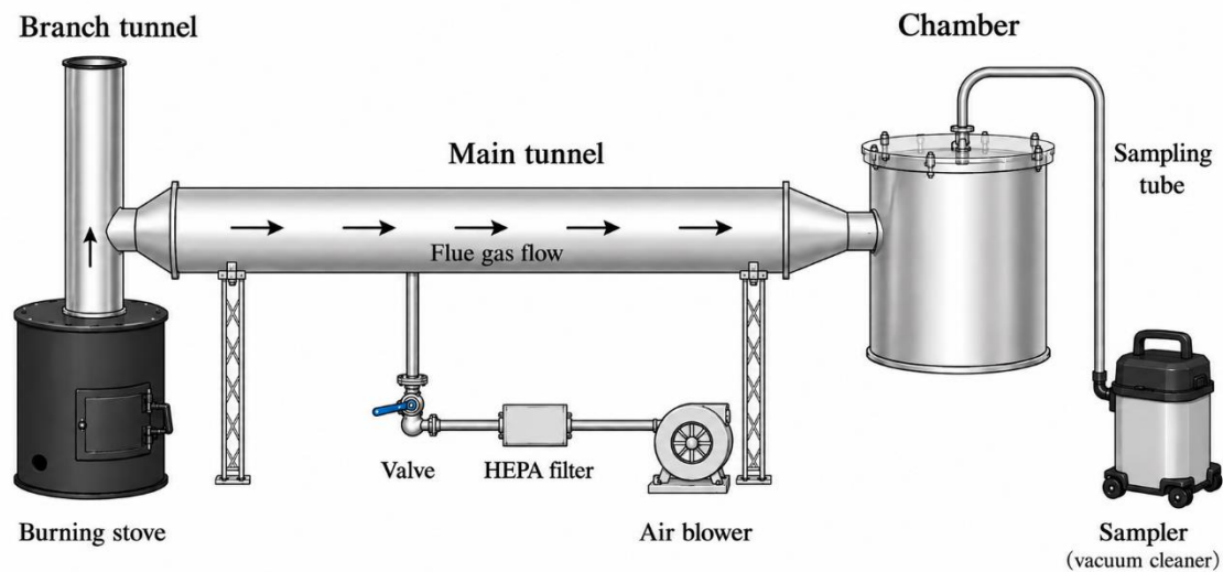
Figure 1. Schematic diagram of the device used in our study to generate and collect biofuel burning aerosols. This figure was created with the assistance of ChatGPT.
