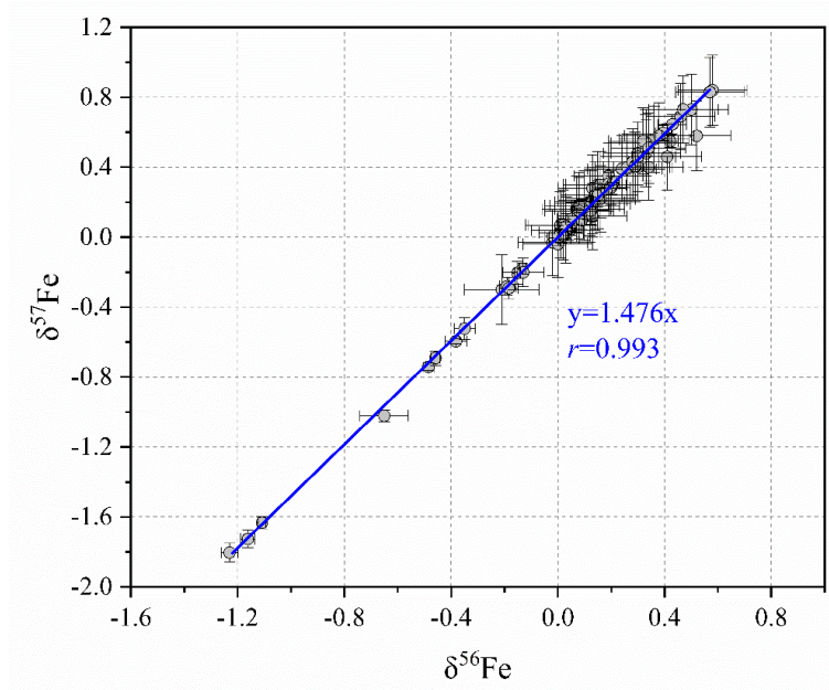
Figure 2. Comparison of \delta^{56}\text{Fe} versus \delta^{57}\text{Fe} values measured in our work. All the individual measurements (84 in total, including measurements of standards) conducted in this work are presented in this figure.
