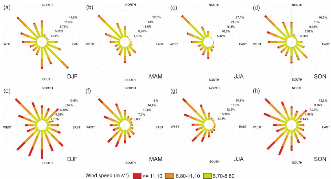
389 Figure 7. Seasonal winds above the sediment transport threshold for the 1991–2020 period. (a– 390 d): San Antonio Oeste, (a): summer, (b): fall, (c): Winter, (d): spring. (e–h): Viedma, (e): summer, (f): 391 fall, (g): winter, (h): spring.
