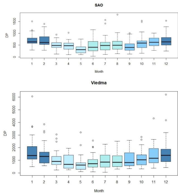
385 Figure 6. Boxplots showing the monthly Drift Potential values obtained from SAO and Viedma 386 meteorological stations during the 1991–2020 period.
