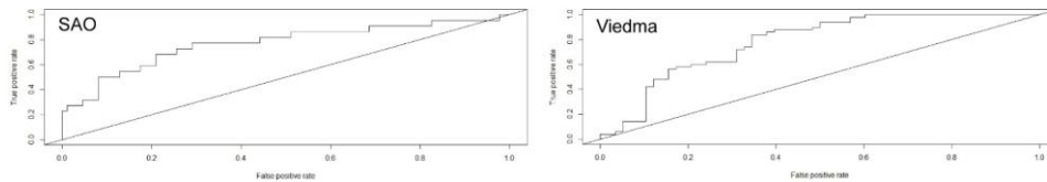
Figure 109. Area Under the Receiver Operating Characteristic (AUC-ROC) curves for the logistic regression model in SAO (left) and Viedma (right). The ROC curve represents the trade-off between sensitivity (true positive rate) and 1 – specificity (false positive rate) across classification thresholds, while the AUC summarizes the model's discrimination ability. The diagonal line represents the random guess (0.5).
