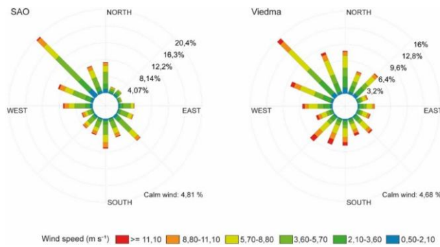
Figure 54. Wind rose of all data from San Antonio and Viedma meteorological stations.
