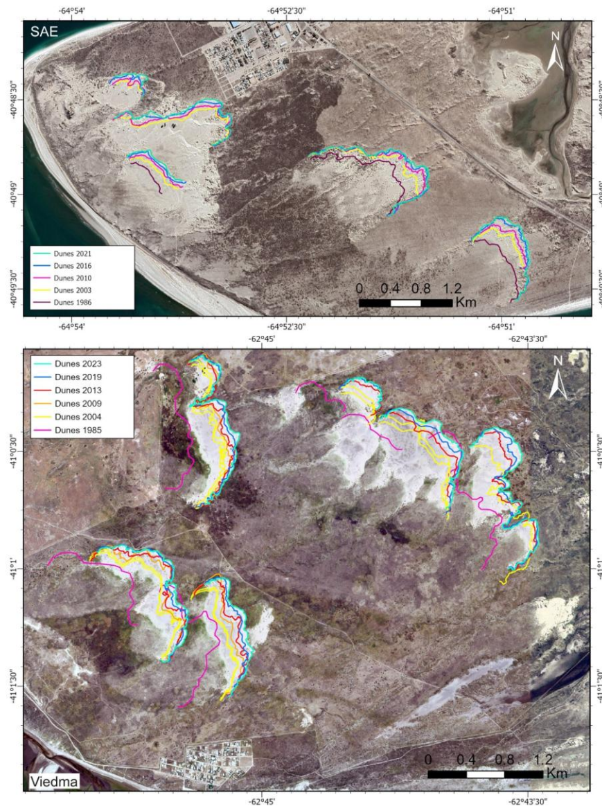
Figure 132. Dune migration between 1985 and 2023 in the San Antonio Este (SAE) area and the Viedma–Villa 7 de Marzo areas. Imagery © 2025-2026 CNES/Airbus and Maxar Technologies, Map data © 2003-2023 Google.
