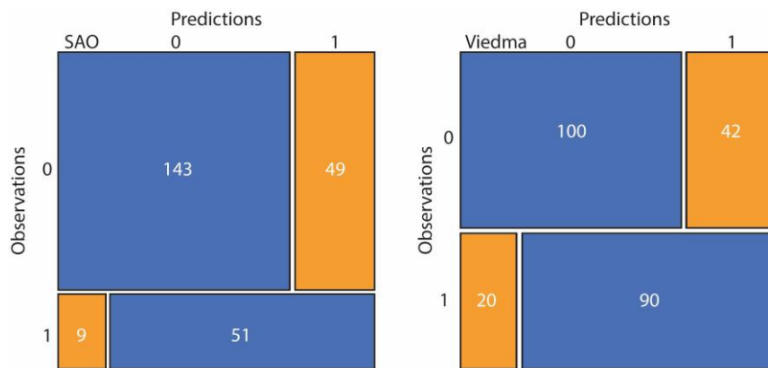
Figure 110. Confusion matrix for the training data in SAO (left) and Viedma (right). The blue areas represent the number of observations equal to predictions, while the orange ones represent the observations different from predictions: (0,0) for true negatives, (1,0) for false positives, (0,1) for false negatives, (1,1) for true positives.
