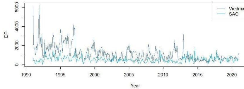
Figure 87. Drift Potential variation between 1991 and 2020, according to the recorded winds in Viedma and SAO.
