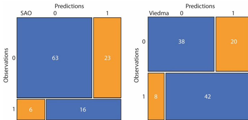
Figure 12. Confusion matrix for the test data in SAO (left) and Viedma (right). The blue areas represent the number of observations equal to predictions, while the orange ones represent the observations different from predictions: (0,0) for true negatives, (1,0) for false positives, (0,1) for false negatives, (1,1) for true positives.
