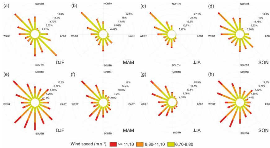
Figure 76. Seasonal winds above the sediment transport threshold for the 1991-2020 period. (a-d): San Antonio Oeste, (a): summer, (b): fall, (c): Winter, (d): spring. (e-h): Viedma, (e): summer, (f): fall, (g): winter, (h): spring.
