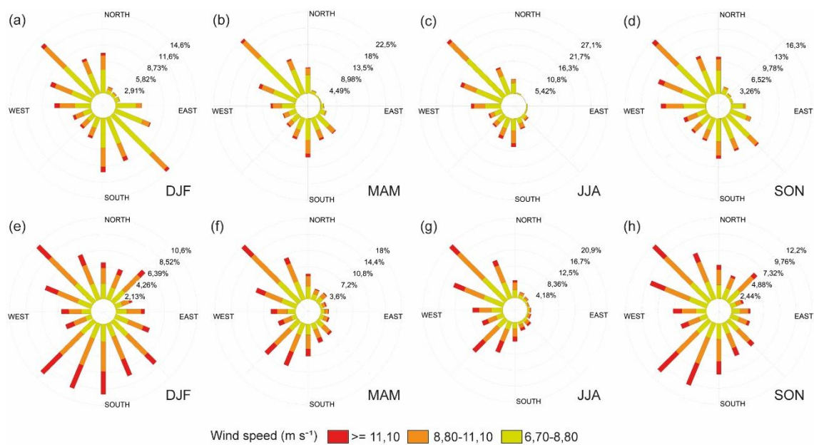
381 Figure 65. Seasonal winds above the sediment transport threshold for the 1991–2020 period. 382
