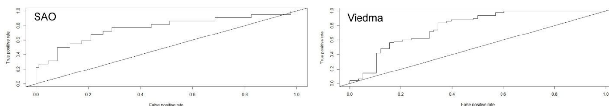
Figure 98. Area Under the Receiver Operating Characteristic (AUC-ROC) curves for the logistic regression model in SAO (left) and Viedma (right). The ROC curve represents the trade-off between sensitivity (true positive rate) and 1 - \text{specificity} (false positive rate) across classification thresholds, while the AUC summarizes the model's discrimination ability. The diagonal line represents the random guess (0.5).
