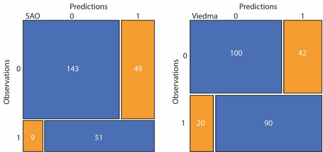
454 Figure 109. Confusion matrix for the training data in SAO (left) and Viedma (right). The blue areas 455 represent the number of observations equal to predictions, while the orange ones represent the 456 observations different from predictions: (0,0) for true negatives, (1,0) for false positives, (0,1) for false 457 negatives, (1,1) for true positives.
