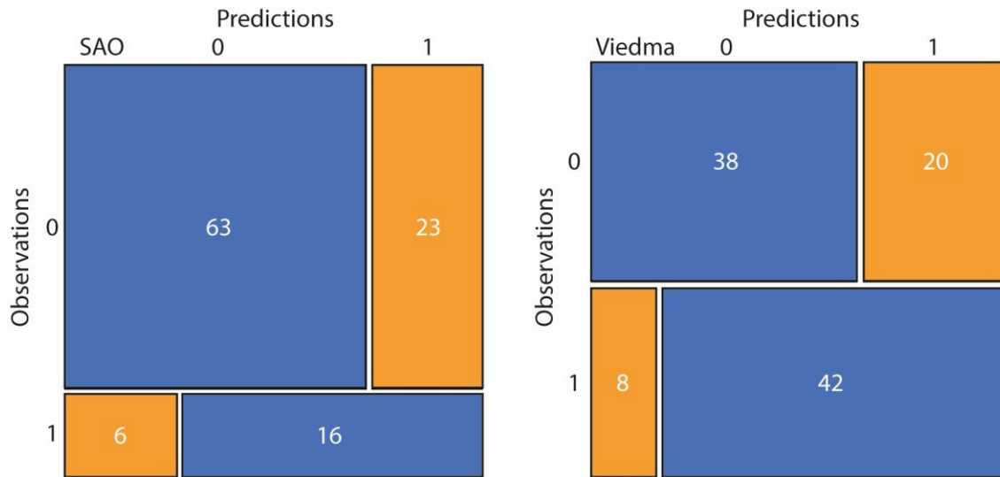
Figure 110. Confusion matrix for the test data in SAO (left) and Viedma (right). The blue areas represent the number of observations equal to predictions, while the orange ones represent the observations different from predictions: (0,0) for true negatives, (1,0) for false positives, (0,1) for false negatives, (1,1) for true positives.
