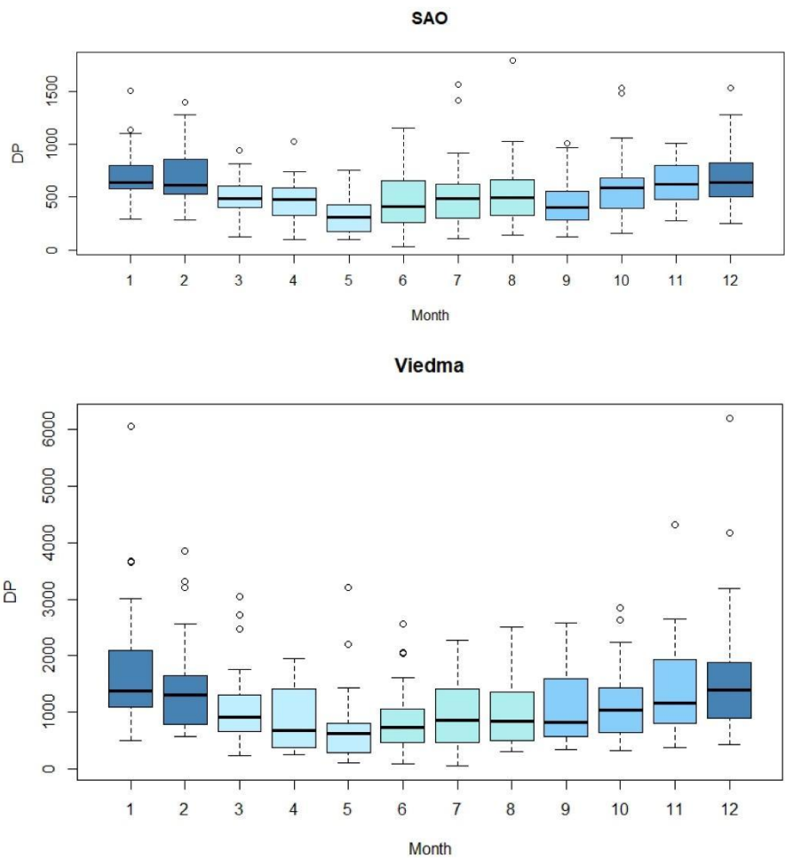
378 Figure 54. Boxplots showing the monthly Drift Potential values obtained from SAO and 379 Viedma meteorological stations during the 1991–2020 period. 380
