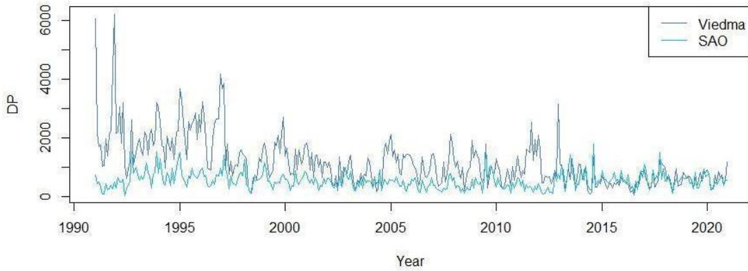
Figure 76. Drift Potential variation between 1991 and 2020, according to the recorded winds in Viedma and SAO.
