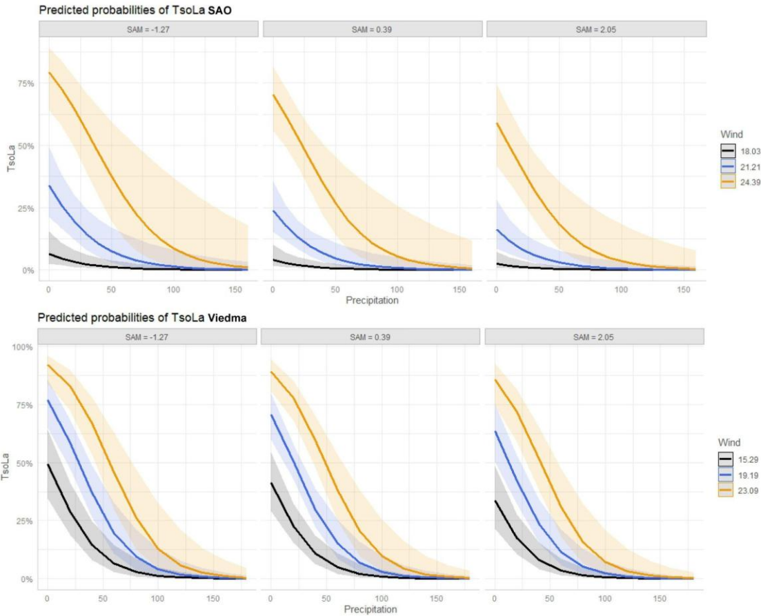
Figure 87. The plots show how the TsoLa probability diminishes when precipitation increases and
