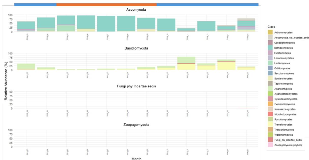
Fig. 4 Class level classification of fungal communities associated with monthly aerosol samples. The bar at the top identifies the “warm” months (mean air temperature > 13.29^\circ\text{C} , indicated in orange) and the “cold” months (mean air temperature < 13.29^\circ\text{C} , indicated in blue). The value 13.29^\circ\text{C} is the mean annual temperature between March 2019 and February 2020.
