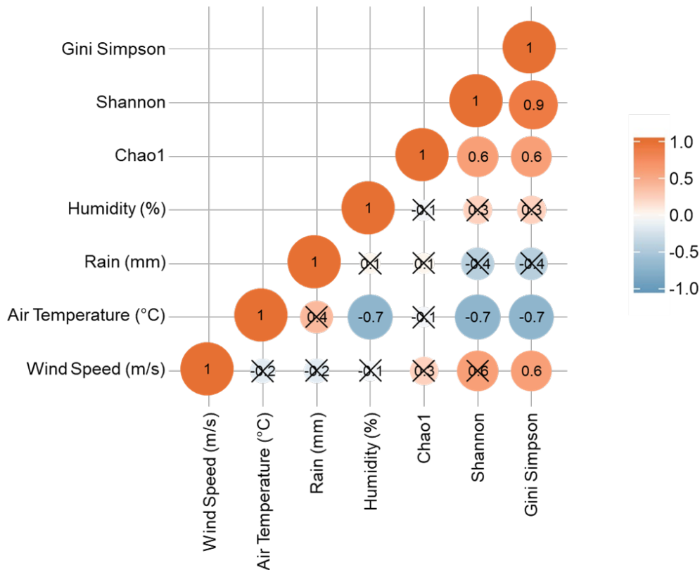
Fig. 2 Spearman's correlation between alpha diversity and meteorological factors. Red/orange circles show positive correlation, and blue circles show negative correlation. A cross "X" on the circle indicates no significance ( p > 0.05 ).
