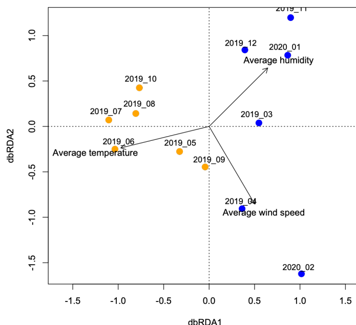
Fig. 3 Analysis of distance-based redundancy (dbRDA) relating meteorological variables with fungal community structure of aerosol samples. The coloured circles represent the respective months for each season, with orange indicating warmer months and blue indicating colder months.
