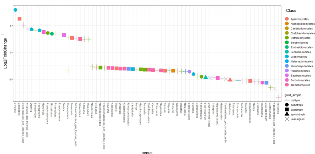
Fig. 5 Log 2 fold change in abundance of fungal genera in response to seasonal changes in temperature ( i.e. “warm” vs “cold”), grouped by fungal guild. Each point represents a genus, coloured by fungal class and shaped by simplified guild category (pathotroph, symbiotroph, saprotroph, unassigned, or multiple guild assignments). Genera are displayed along the x-axis, with log 2 fold change on the y-axis. The shape legend indicates guild affiliation, highlighting differences in functional responses across ecological guilds.
