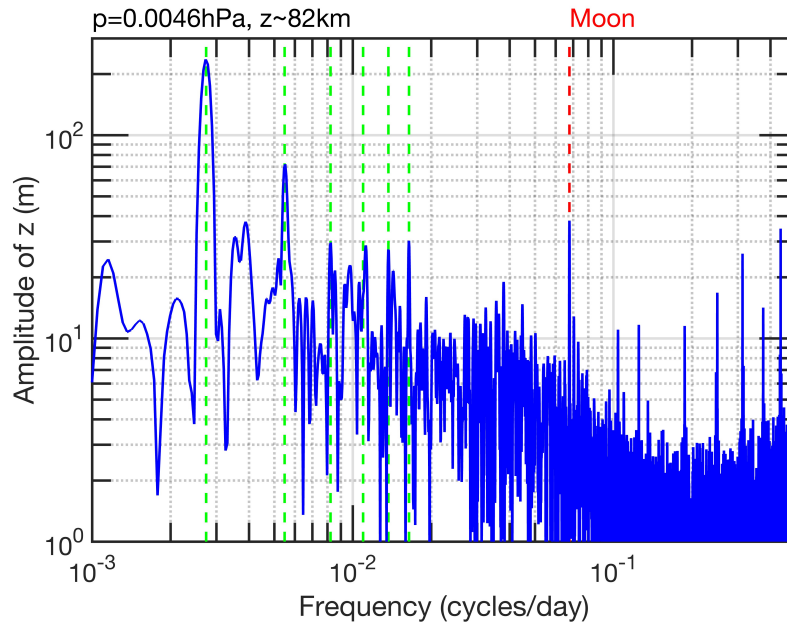
Figure 2. FFT amplitude spectrum of oscillations of geopotential height z of a fixed pressure level (0.0046 hPa) in about 82 km height. Aura/MLS data from the equatorial latitude belt (10°S to 10°N) were taken for the time interval from 2004 to 2021. The vertical red dashed line indicates the frequency of the lunar semimonthly tide. The green dashed lines indicate the annual oscillation and its harmonics.
