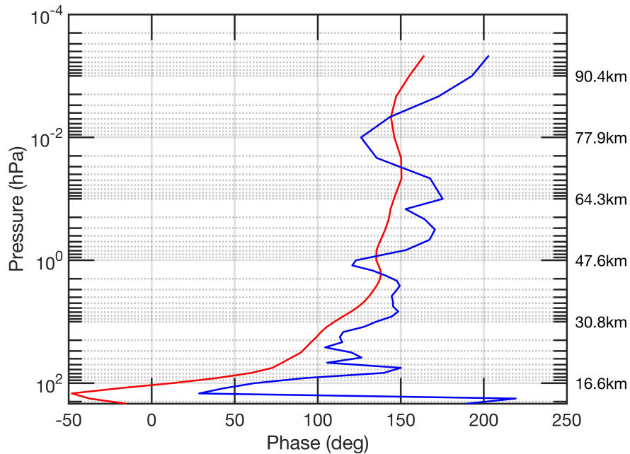
Figure 6. Vertical profiles of lunar tidal phase in geopotential height (red line) and temperature (blue line). Aura/MLS data from the equatorial latitude belt ( 10^{\circ}\text{S} to 10^{\circ}\text{N} ) were taken for the time interval from 2004 to 2021. The approximated heights of the pressure levels are given by labels at the right-hand side. Phase 0^{\circ} means that Aura/MLS measures the maximum of the tidal wave at New Moon. Phase 180^{\circ} means that Aura/MLS measures the maximum of the tidal wave at First Quarter Moon.
