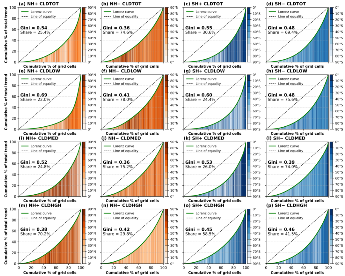
Figure 6. Asymmetry of cloud trends between hemispheres. Lorenz curves of long-term CLDTOT (a-d), CLDLOW (e-h), CLDMED (i-l), CLDHGH (m-p) trend in the Northern Hemisphere (0° to 90°N) and Southern Hemisphere (0° to 90°S) during the 2015–2100 in CTL run. The share indicates the percentage of an increase or decrease in the trend. The results of the AF50, BE50, and REAL experiments can be found in Fig. S23-S25.
