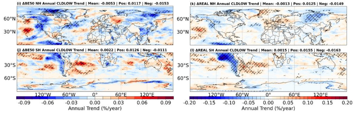
Figure 2. Spatial patterns of long-term total and low-level cloud cover trends driven by diverse land-use scenarios. Maps display the anomalous annual trends (%/year) of total cloud cover (a–f) and low-level cloud cover (g–l) for both the Northern and Southern Hemispheres. The visualized trends represent the differences (denoted by symbol \Delta ) between the specific land-use forcings (idealized afforestation, bioenergy expansion, and realistic afforestation) and the control simulation. Blue shading indicates a decreasing trend in cloud cover, while red shading depicts an increasing trend. The cross-hatching highlights grid cells where the long-term trends are statistically significant ( p < 0.05 ). Panel headers provide the regional mean trend, alongside the averages of all positive (Pos) and negative (Neg) grid-level trends within the respective domains.
