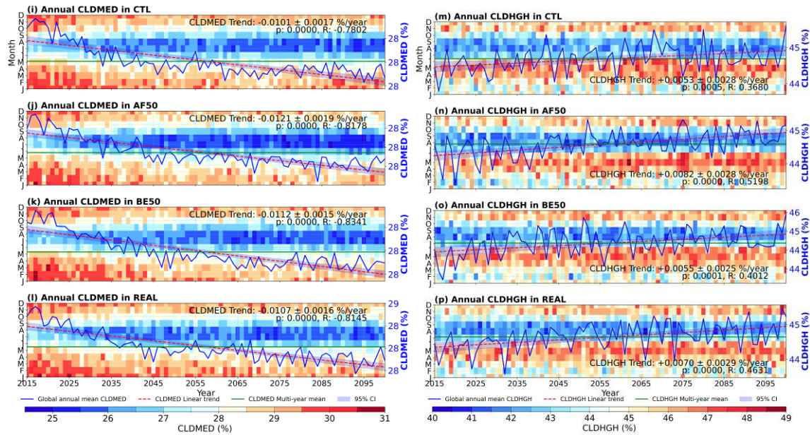
Figure 1. Simulated long-term trends and seasonal variations of area-weighted global mean cloud cover. Panels display the time series (2015–2100) for total (a–d), low (e–h), medium (i–l), and high-level (m–p) cloud cover under CTL, AF50, BE50, and REAL scenarios. In each panel, heatmaps show the monthly variations, while blue and solid lines track the global annual means. Linear trend lines (dashed) and multi-year means (horizontal solid lines) are superimposed, with statistical significance ( p ) and regression coefficients ( R ) provided. The shaded areas indicate the 95% confidence intervals (CI). Uncertainty propagation for baseline subtractions was performed via quadrature addition of standard errors (Taylor, 1997; Mastrandrea et al., 2010).
