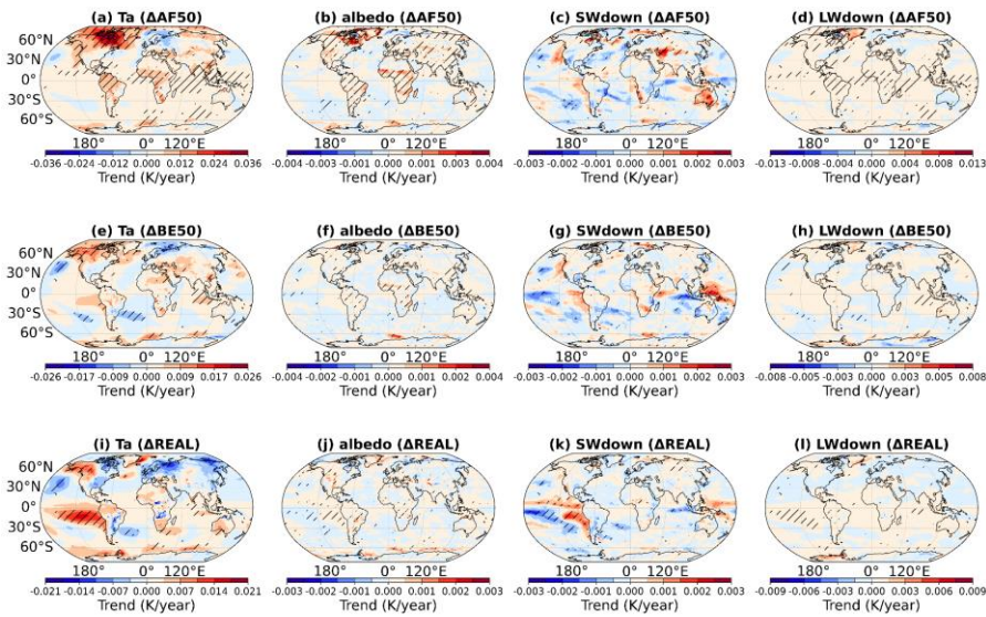
Figure 5. Long-term trends of key physical terms (decomposed by the surface energy balance equation) induced by different LUCC. T_a represents the atmospheric feedback term, albedo denotes the surface albedo term, and SWdown ( SW_d ) and LWdown ( LW_d ) indicate the downward shortwave and longwave radiation terms, respectively. The black hatch indicates the grids that passed the test of significance ( p<0.05 ).
