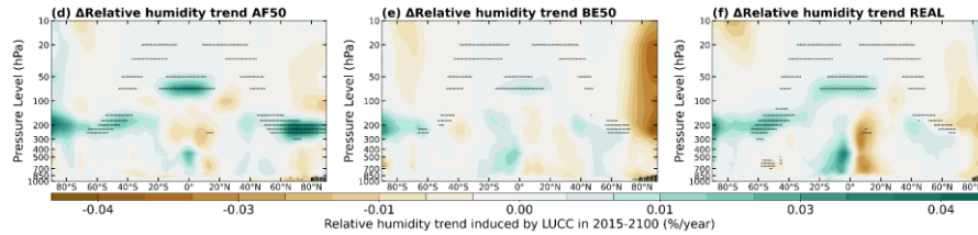
Figure 1011. Vertical profiles of Trends in temperature and relative humidity trends induced by different LUCC at vertical heights. The black asterisks denote grid cells with statistically significant trends. black asterisk indicates the grids that passed the test of significance ( p < 0.05 ).
