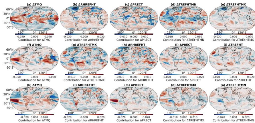
Figure 910. Spatial drivers and contribution of CLDTOT revealed by machine learning response to different land use change. The first to third rows represent AF50, BE50 and REAL experiments respectively. The contribution is expressed in SHapley Additive exPlanations (SHAP) value (Berdugo et al., 2022). The corresponding results for CLDLOW, CLDMED, and CLDHGH are presented in Figure S27, S29, and S31, respectively.
