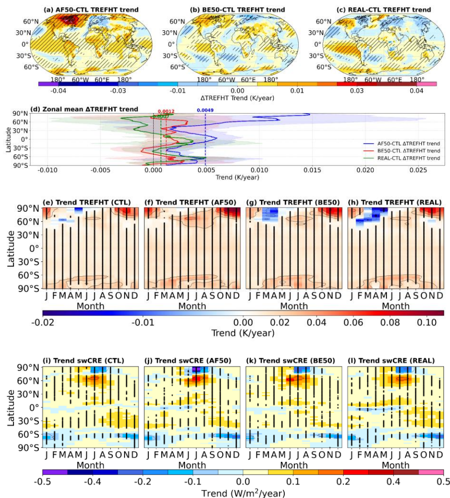
Figure 4. Spatiotemporal change Long-term trends of reference height temperature at reference height (TREFHT) and shortwave cloud radiative effect (swCRE). (a-d) Spatial patterns and zonal mean distribution of reference height temperature TREFHT induced by different land use and land cover change. (e-l) Seasonal trends in temperature-TREFHT and shortwave cloud radiative effects swCRE (swCRE)
