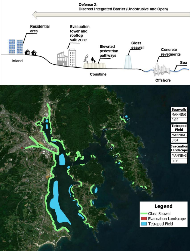
Fig. 4: Multi-layered defence cross-section and in-situ placement for the Discreet Integrated Barrier system (Defence 2). Sentinel-2 imagery by © European Union, Copernicus Programme. All rights reserved.
