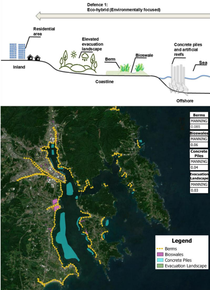
Fig. 3: Multi-layered defence cross section and placement within Kesennuma for the Eco-hybrid defence system (Defence 1). Sentinel-2 imagery by © European Union, Copernicus Programme. All rights reserved.
