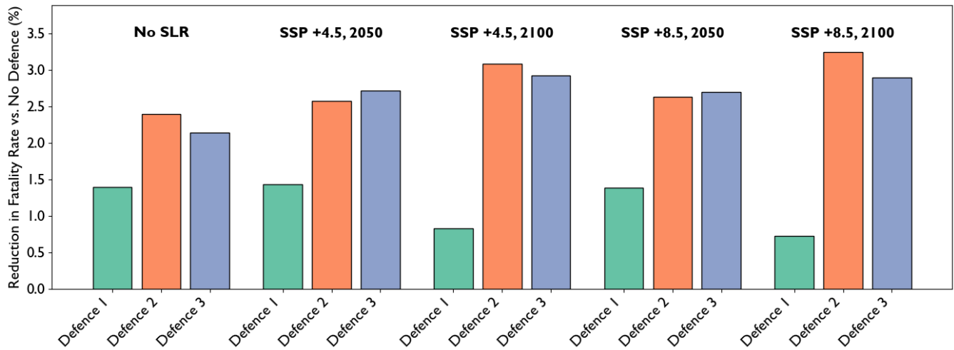
Fig. 12: Fatality reduction relative to the no-defence baseline for the three defence configurations under all SLR scenarios for (a) Kesennuma and (b) Karakuwa, based on the Japan Trench tsunami source model. In Kesennuma, Defence 2 and Defence 3 show increasing reduction as SLR increases, while Defence 1's reduction falls sharply under late-century, high-emission scenarios. The same pattern is observed in Karakuwa.
