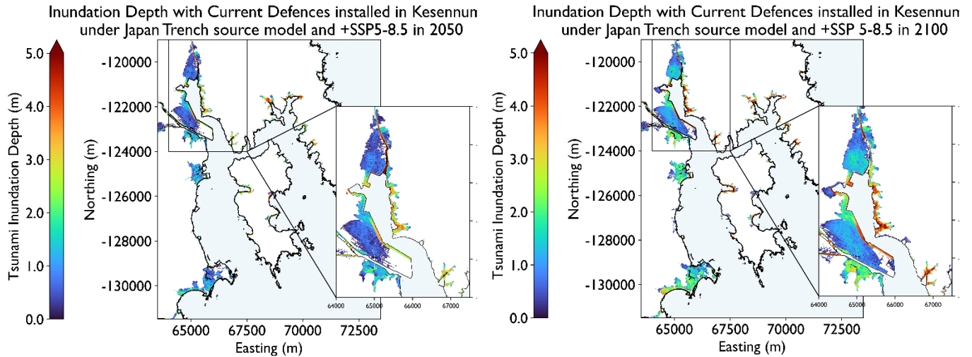
Fig. 9: Increasing inundation extent and depth under different SLR scenarios (a) No SLR, (b) SSP2-4.5 in 2050, (c) SSP2-4.5 in 2100, (d) SSP5-8.5 in 2050 and (e) SSP5-8.5 in 2100 for the defences currently installed within Kesennuma. Results are shown for the Japan Trench scenario as the representative case, as all three modelled sources produced consistent relative patterns.
