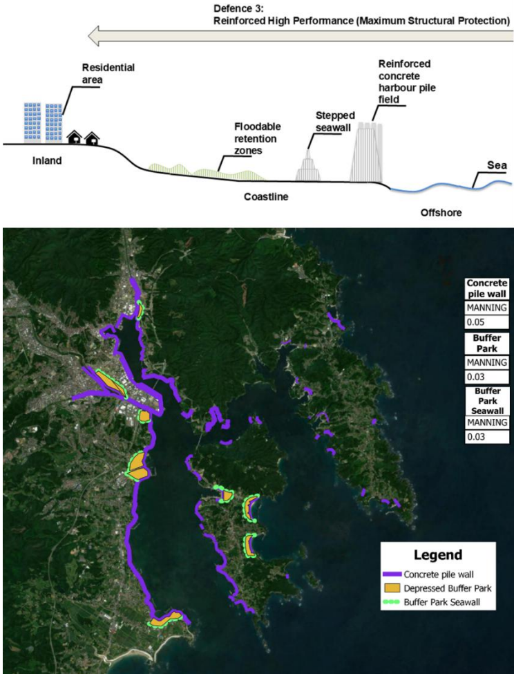
Fig. 5: Cross-section and in-situ placement of the three elements from the Reinforced High-Performance system (Defence 3). Sentinel-2 imagery by © European Union, Copernicus Programme. All rights reserved.
