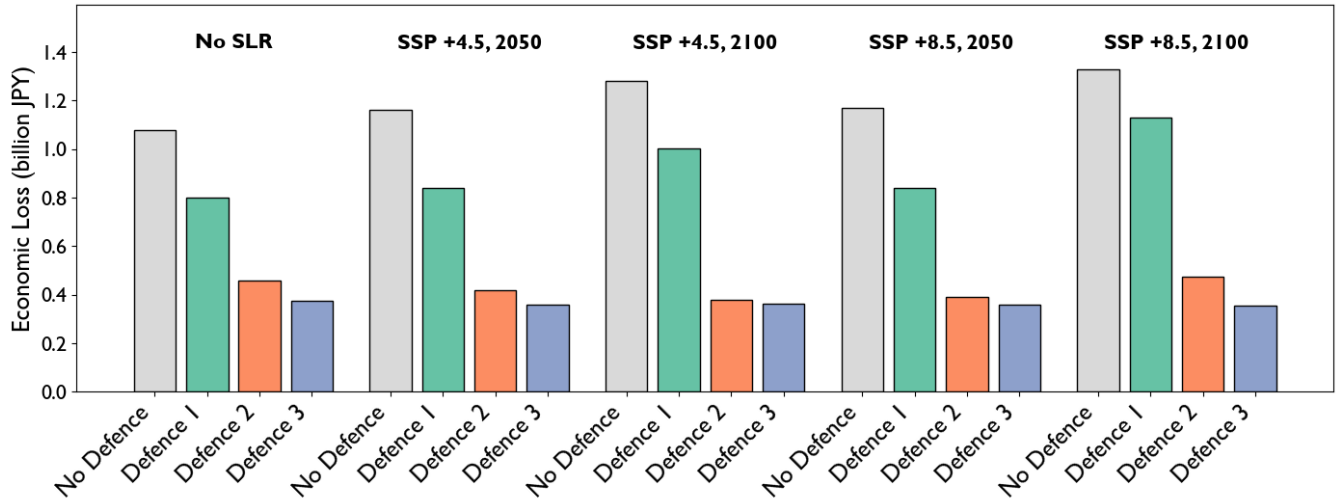
Economic Loss for Key Buildings in Kesennuma under Japan Trench source model
