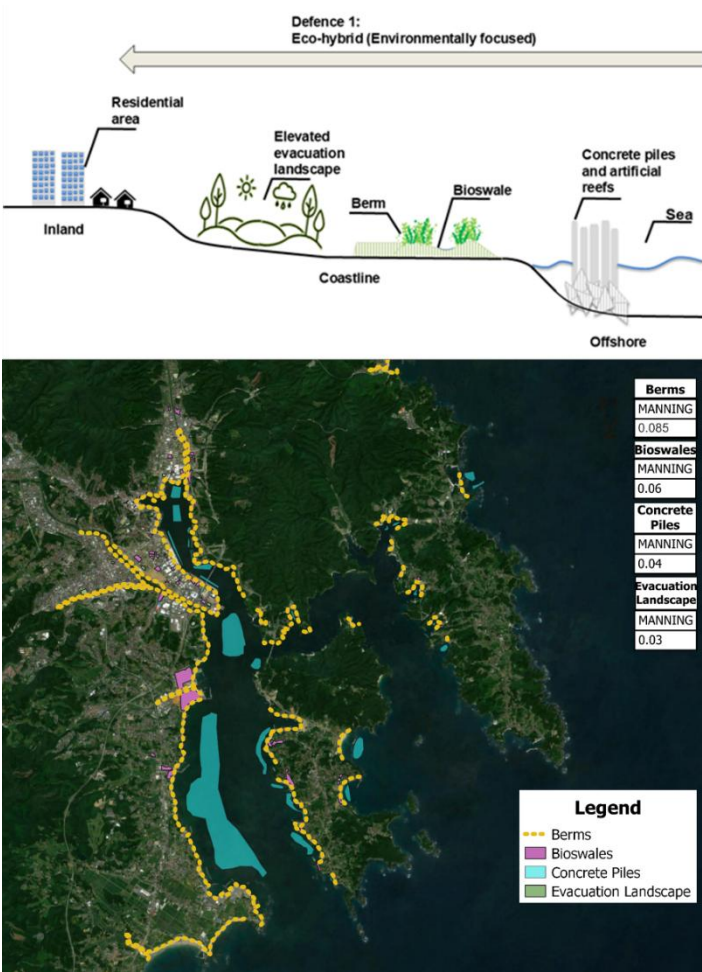
Fig. 3: Multi-layered defence cross section and placement within Kesennuma for the Eco-hybrid defence system (Defence 1). Sentinel-2 imagery by © European Union, Copernicus Programme. All rights reserved.
