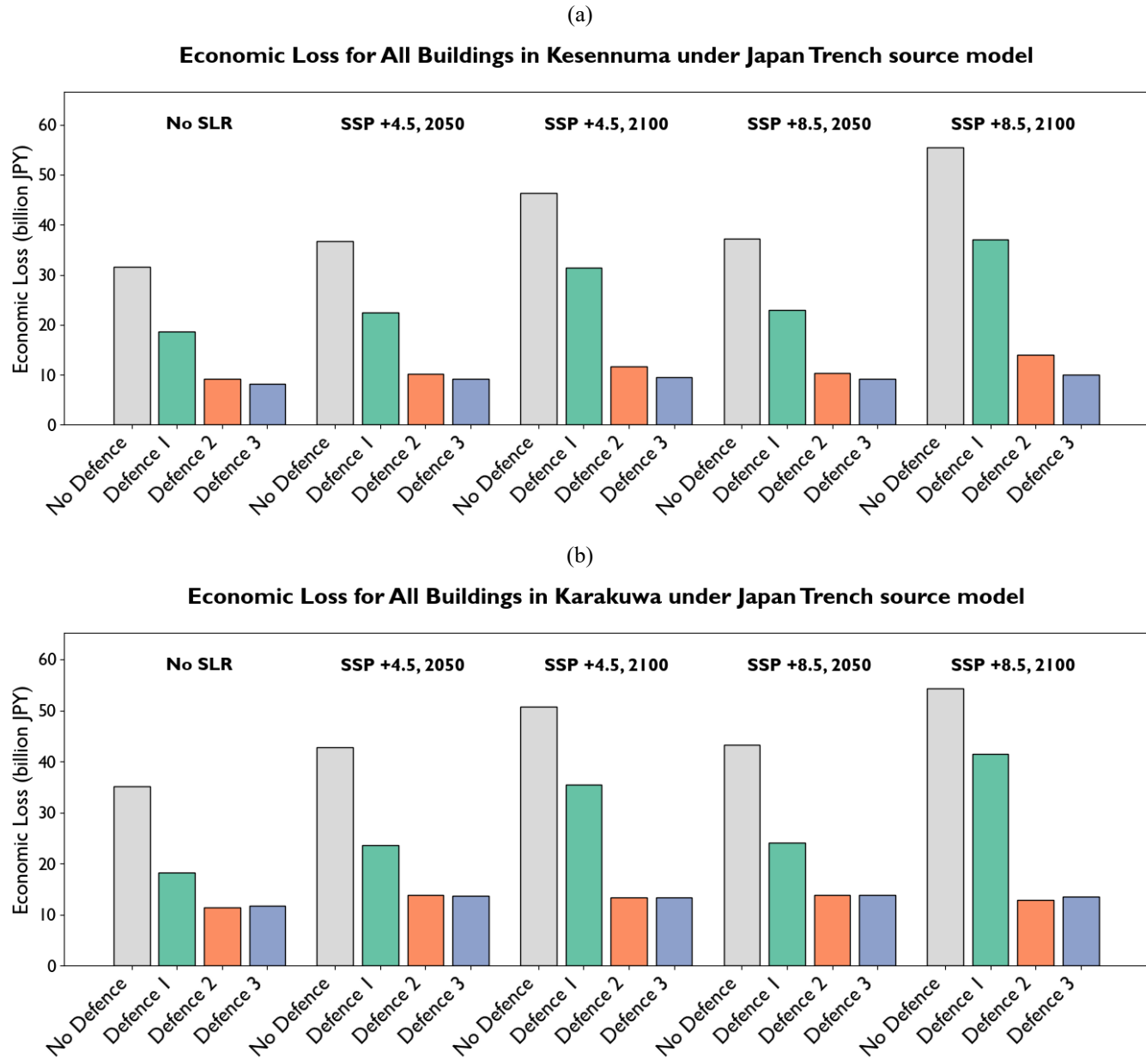
Fig. 13: Economic loss for all buildings in (a) Kesennuma and (b) Karakuwa. Defence 1 produces consistently higher losses across all scenarios, while Defences 2 and 3 differ only marginally.
