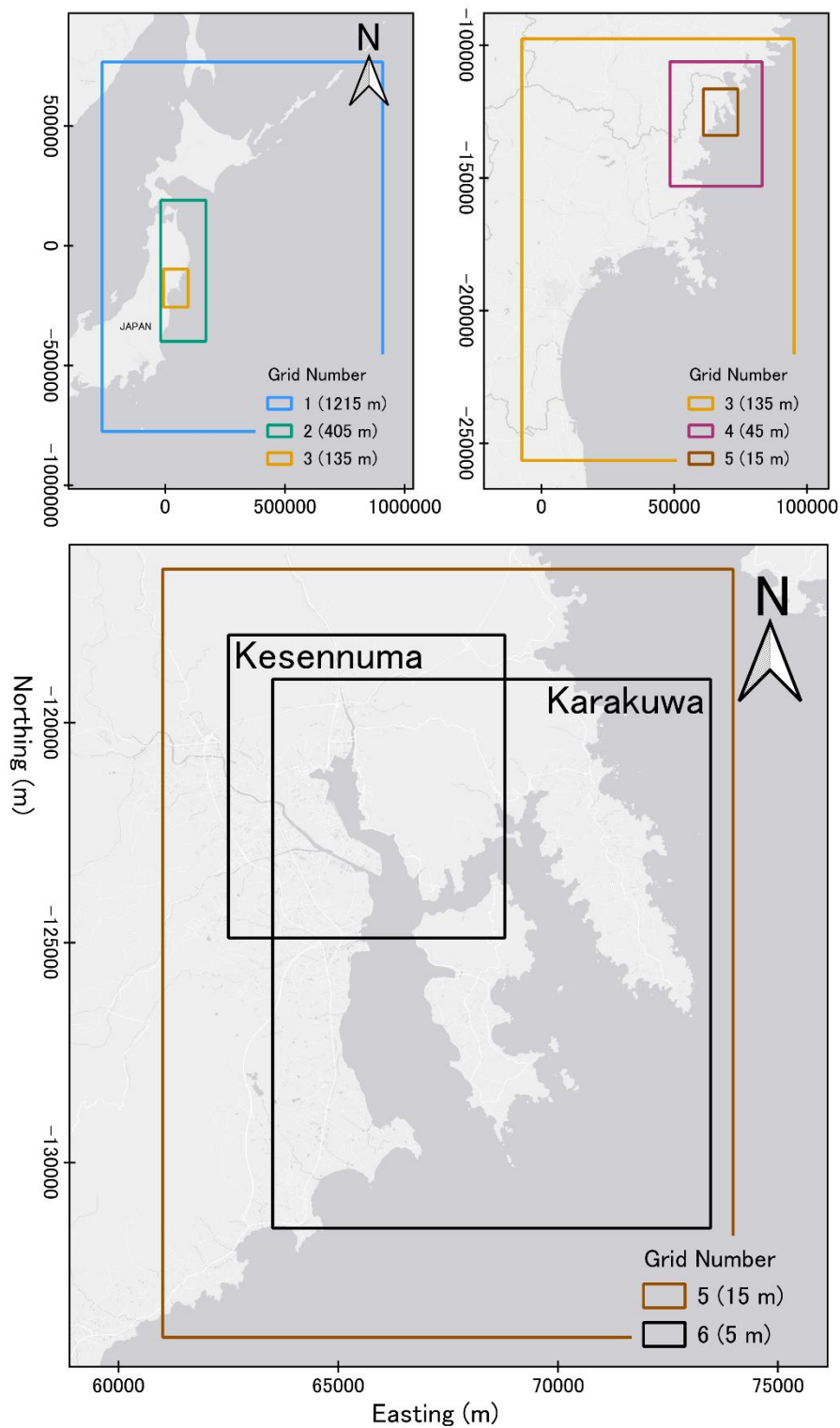
Fig. 6: Computational Domain (Grid 1) and the subsequent nesting grids, showing the difference in locations of the Kesennuma and Karakuwa final grids. Sources: Esri (World Gray Canvas) | Powered by Esri.
