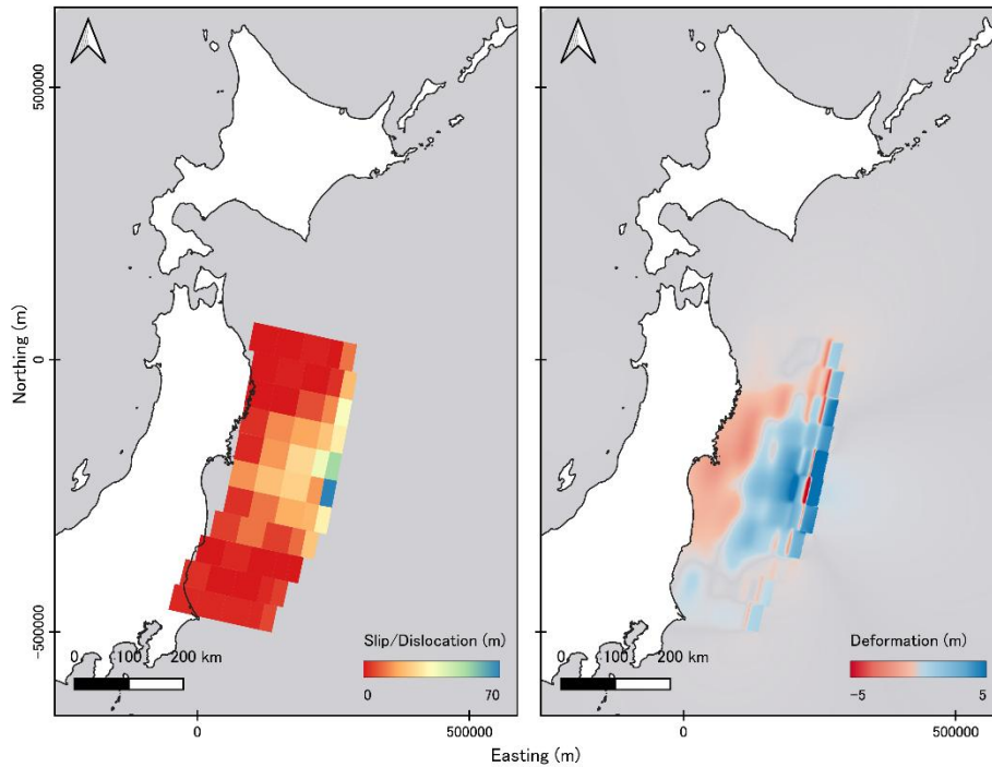
Fig. 7: Tsunami source model locations, slip distribution and deformation for (a) Kuril Trench (b) Japan Trench and (c) 2011 GEJE (Tohoku).
