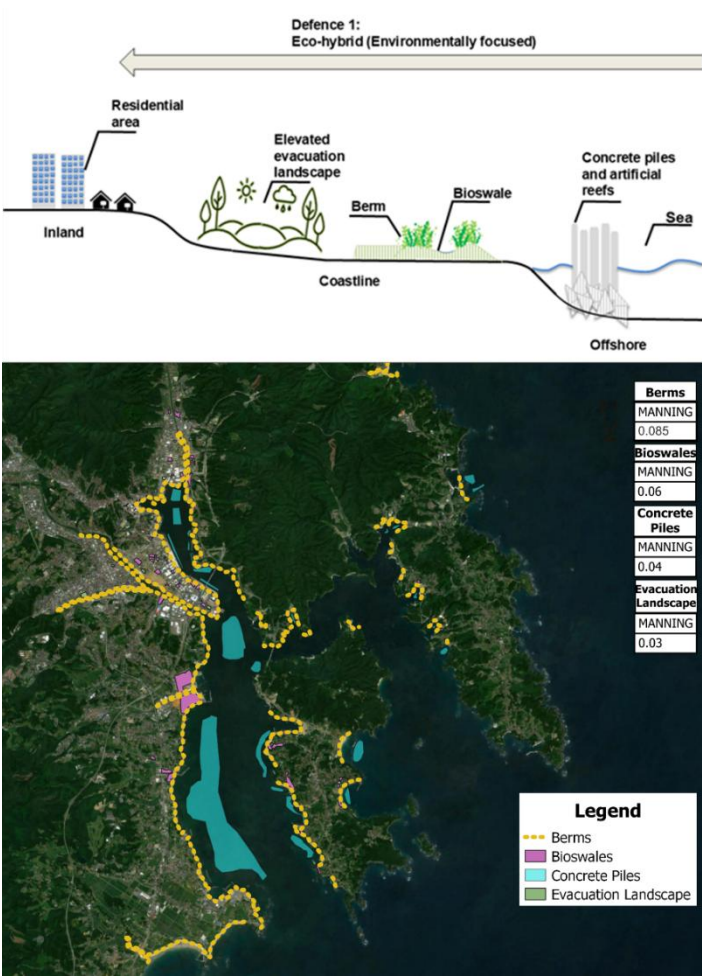
Fig. 3: Multi-layered defence cross section and placement within Kesennuma for the Eco-hybrid defence system (Defence 1). Base from Sentinel-2 imagery, Copernicus Programme, European Union.
