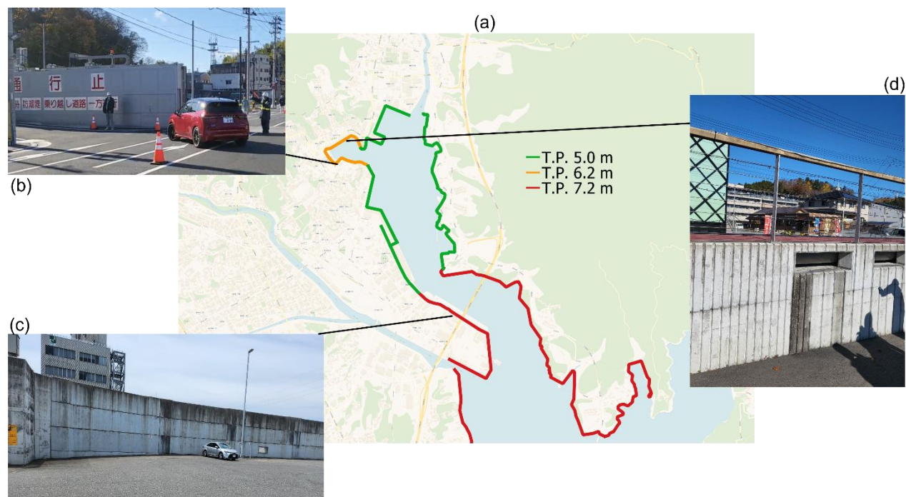
Fig. 2: Current tsunami mitigation infrastructure in Central Kesennuma (a) Seawall heights (b) Automatic seagate controlled remotely by J Alert in Tokyo (c) Tallest concrete seawall observed at Kesennuma Port (d) Barrier hydraulically activated by water ingress, increasing barrier height by 1 metre. Base map from OpenStreetMap contributors.
