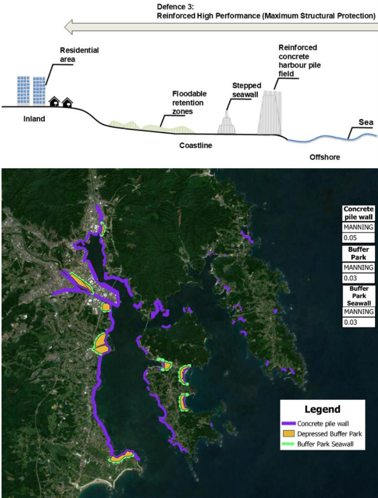
Fig. 5: Cross-section and in-situ placement of the three elements from the Reinforced High-Performance system (Defence 3). Base from Sentinel-2 imagery, Copernicus Programme, European Union.
