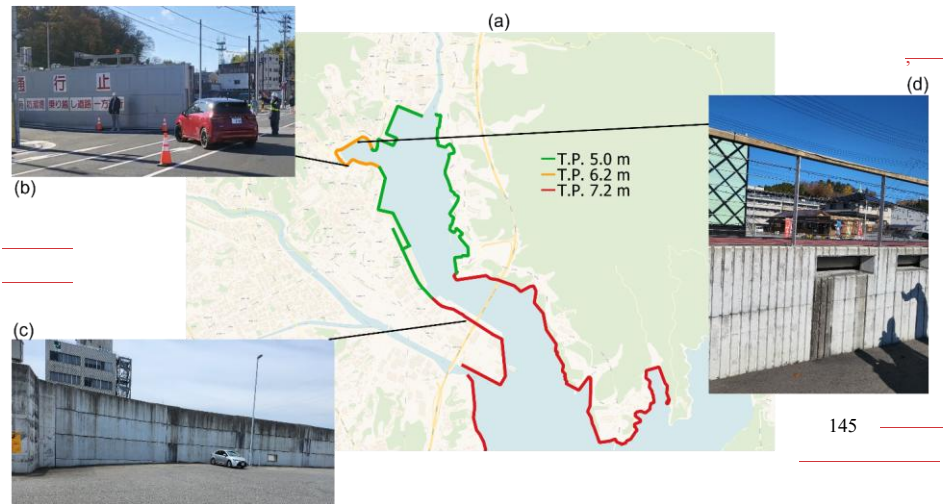
Fig. 2: Current tsunami mitigation infrastructure in Central Kesennuma (a) Seawall heights (b) Automatic seagate controlled remotely by J Alert in Tokyo (c) Tallest concrete seawall observed at Kesennuma Port (d) Barrier hydraulically activated by water ingress, increasing barrier height by 1 metre. Base map from OpenStreetMap contributors.
