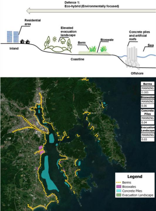
Fig. 3: Multi-layered defence cross section and placement within Kesennuma for the Eco-hybrid defence system (Defence 1). Base from Sentinel-2 imagery, Copernicus Programme, European Union.
