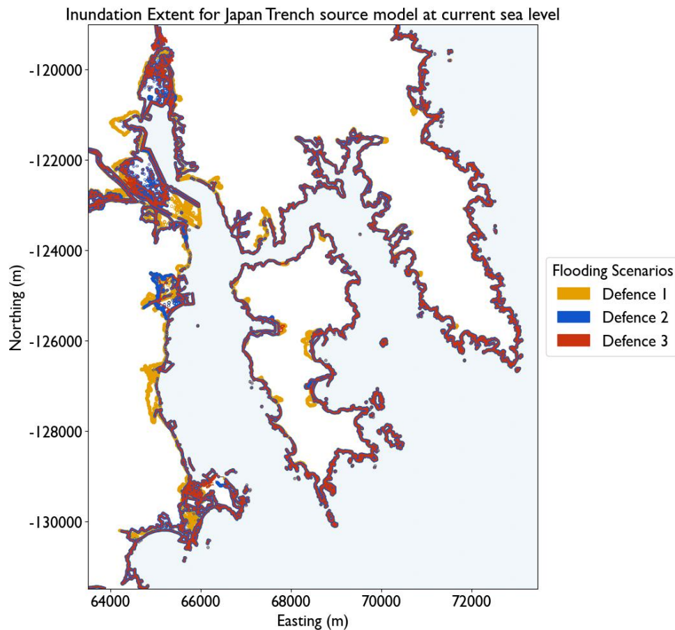
Fig. 11: Spatial extents showing differences in inundation patterns and areas for each defence configuration.
