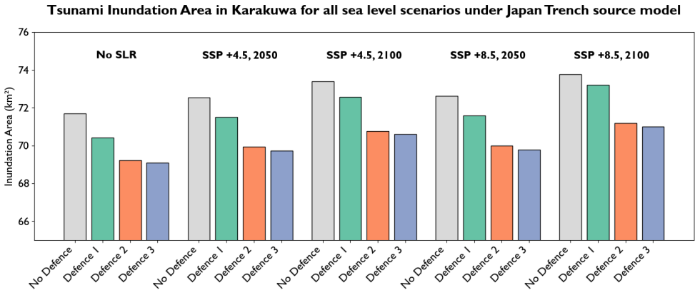
Fig. 10: Inundation area for (a) Kesennuma and (b) Karakuwa across all SLR scenarios for the three defence configurations and a No Defence baseline, based on the Japan Trench tsunami source model, shown as the representative case because all three modelled sources produced the same relative performance hierarchy among the defence configurations. In both locations, inundation extent increases with SLR, with Defence 2 and Defence 3 limiting area more effectively than Defence 1.
