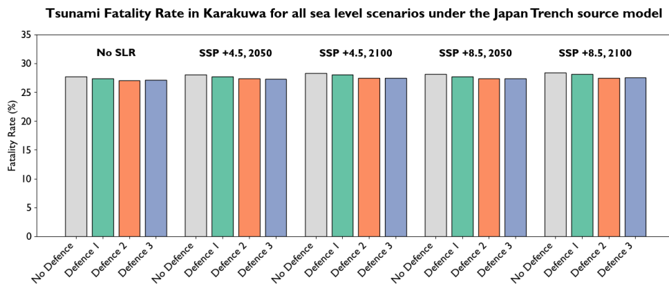
Fig. 12: Fatality estimates for the three defence configurations under all SLR scenarios for (a) Kesennuma and (b) Karakuwa, based on the Japan Trench tsunami source model. Fatality rates increase significantly at the highest sea level increase in Kesennuma, and the relative performance of the defences stays consistent throughout, although differences are marginal within Karakuwa.
