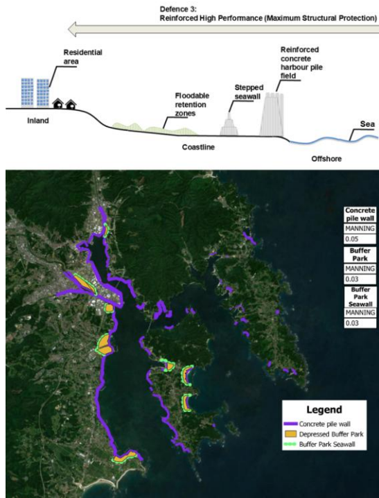
Fig. 5: Cross-section and in-situ placement of the three elements from the Reinforced High-Performance system (Defence 3). Base from Sentinel-2 imagery, Copernicus Programme, European Union.
