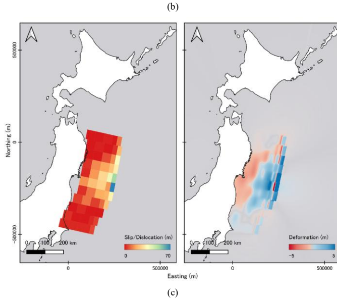
Fig. 7: Tsunami source model locations, slip distribution and deformation for (a) Kuril Trench (b) Japan Trench and (c) 2011 GEJE (Tohoku).
