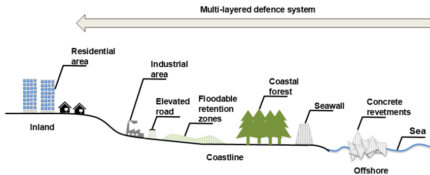
Fig. 1: Example of a multi-layered defence system promoted by the MLIT post-2011.
