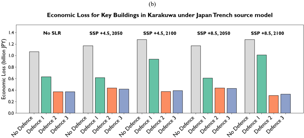
Fig. 15: Economic loss for key buildings in (a) Kesennuma and (b) Karakuwa, mirroring results from all buildings where Defence 1 produces consistently higher losses across all scenarios and Defences 2 and 3 differ only marginally.
