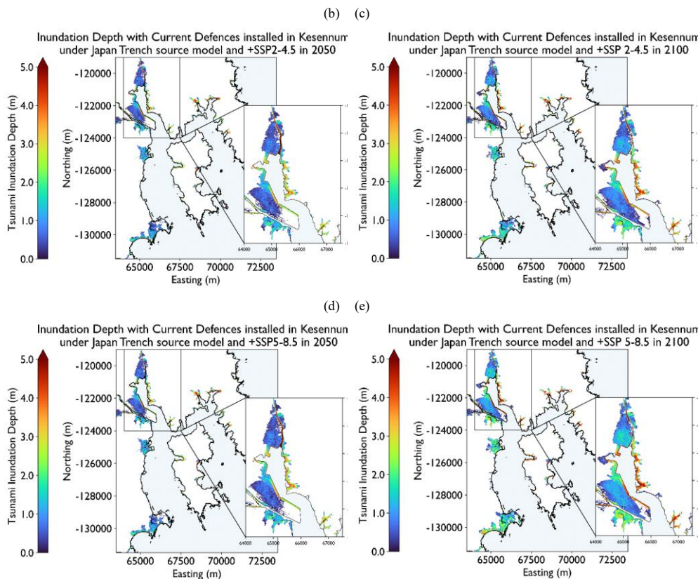
Fig. 9: Increasing inundation extent and depth under different SLR scenarios (a) No SLR, (b) SSP2-4.5 in 2050, (c) SSP2-4.5 in 2100, (d) SSP5-8.5 in 2050 and (e) SSP5-8.5 in 2100 for the defences currently installed within Kesennur. Results are shown for the Japan Trench scenario as the representative case, as all three modelled sources produced consistent relative patterns.
