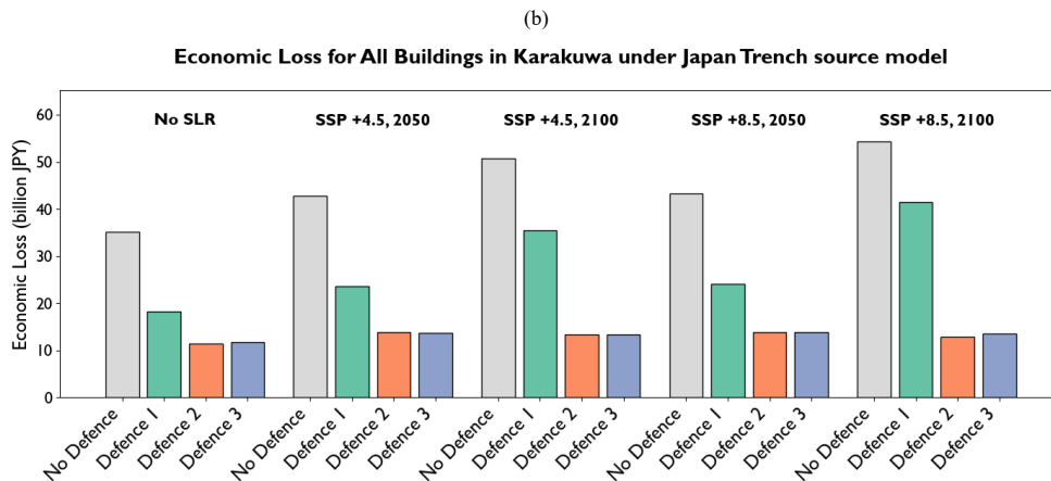
Fig. 13: Economic loss for all buildings in (a) Kesennuma and (b) Karakuwa. Defence 1 produces consistently higher losses across all scenarios, while Defences 2 and 3 differ only marginally.
