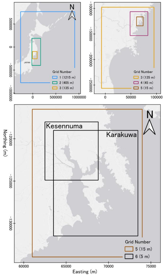
Fig. 6: Computational Domain (Grid 1) and the subsequent nesting grids, showing the difference in locations of the Kesennuma and Karakuwa final grids. Sources: Esri (World Gray Canvas) | Powered by Esri.
