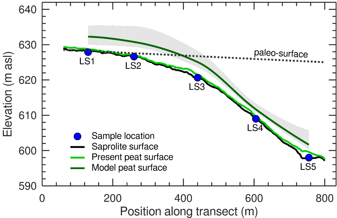
Figure 3: Study hillslope cross section with 10× vertical exaggeration showing the five hillslope sample positions (LS1 to LS5). The black, solid line shows the elevation of the top of the saprolite surveyed with ground penetrating radar (Henrion et al., 2024). The light green line shows the elevation of the modern peat surface. The cosmogenic nuclide-based estimate of peat thickness, interpolated between measurement points, is shown by the dark green line and the 90% confidence interval by the grey band. The dashed, black line shows the elevation and dip of the pre-Senonian surface (labeled paleo-surface).
