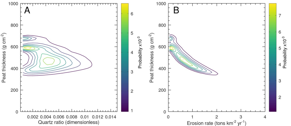
Figure 6: Joint-distribution plots showing (A) the quartz ratio (saturated peat/saprolite) vs. the watershed-averaged saturated peat thickness (g cm -2 ) and (B) the saturated peat thickness vs. the erosion rate of the saprolite inferred from the Markov Chain Monte Carlo inversion of the stream sediment (LSR-1).
