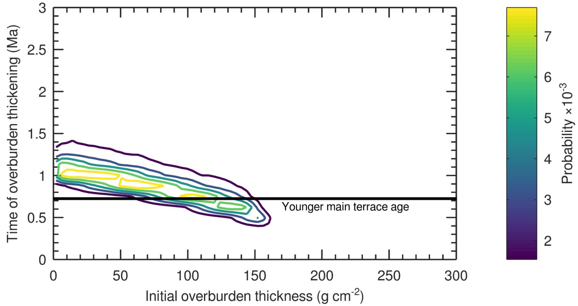
Figure 5: Joint-distribution plot showing the original overburden thickness vs. timing of the overburden thickening event resolved by the Markov Chain Monte Carlo inversion for LS1. The initial overburden thickness has been corrected by the overburden mass between the sample and the contact between the saprolite and peat, assuming a density of saturated saprolite of 1.8 g cm -3 . The thickening event may correspond to the onset of peat cover. The black line shows the younger main terrace age at Romont reported by Rixhon et al. (2011), a temporal marker of Ardennes uplift (Section 6.3).
