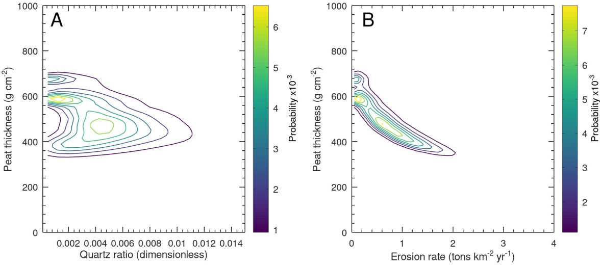
Figure 6: Joint-distribution plots showing (A) the quartz ratio (saturated peat/saprolite) vs. the watershed-averaged saturated peat thickness (g cm -2 ) and (B) the saturated peat thickness vs. the erosion rate of the saprolite inferred from the Markov Chain Monte Carlo inversion of the stream sediment (LSR-1).
