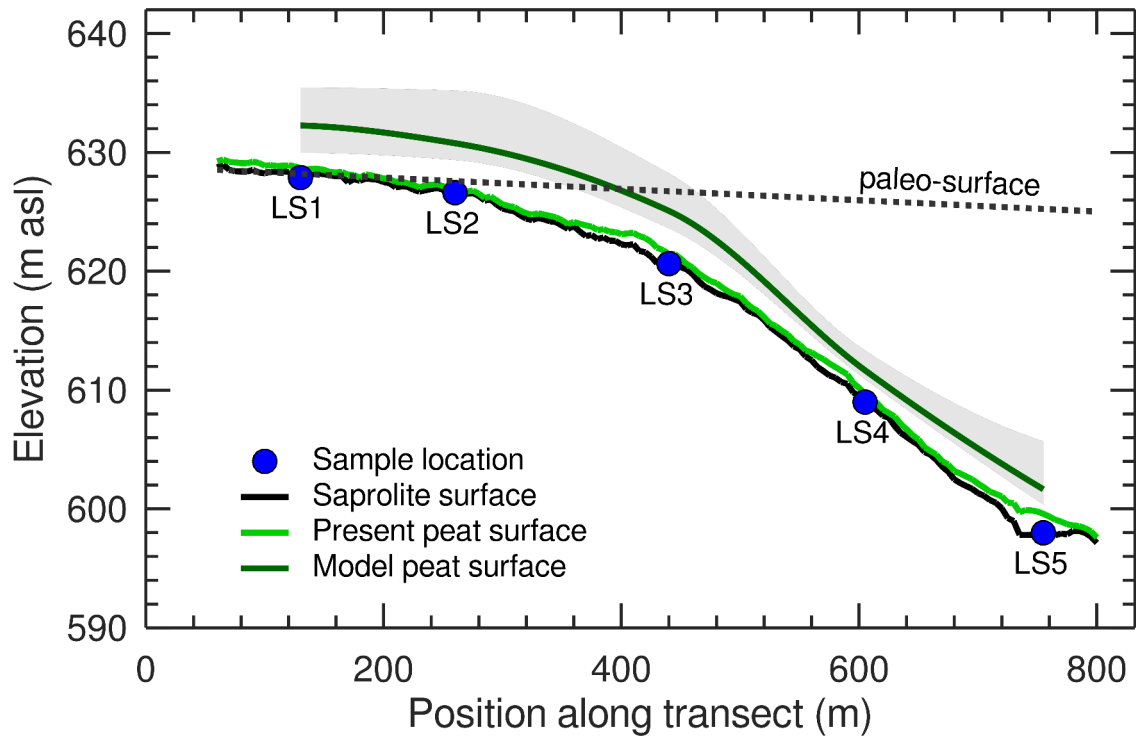
Figure 3: Study hillslope cross section with 10× vertical exaggeration showingwith the five hillslope sample positions (LS1 to LS5). The black, solid line shows the elevation of the top of the saprolite surveyed with ground penetrating radar (Henrion et al., 2024). The light green line shows the elevation of the modern peat surface. The cosmogenic nuclide-based estimate of peat thickness, interpolated between measurement points, is shown by the dark green line and the 90% confidence interval by the grey band. The dashed, black line shows the elevation and dip of the pre-Senonian surface (labeled paleo-surface).
