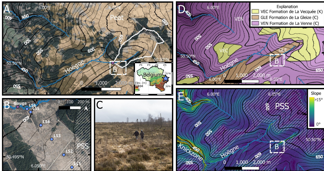
Figure 1: A. Regional map showing the locations of the study hillslope (dashed box labeled B) and study catchment (denoted by the white, solid polygon upstream of the purple marker) and the modern distribution of peat soils (orange shading) (citation) with reference to 2020 orthophotography (Source: Walloon Public Service, CC-BY 4.0 License). Contour elevations (m) are given by the white numbers. B. Local map of the study hillslope showing the locations of samples LS1 to LS6, the stream gauge where LSR-1 was collected, and the pre-Senonian surface (PSS). C. View of the study hillslope looking upslope. D. Approximate bedrock geologic map adapted from Demoulin et al. (2018b) and the provisional geological map of Marion et al. (2018). E. Regional slope map showing the knickzone on the Hoëgne. The location extent of the pre-Senonian surface (PSS) was calculated from a three point problem, assuming a planar geometry.
